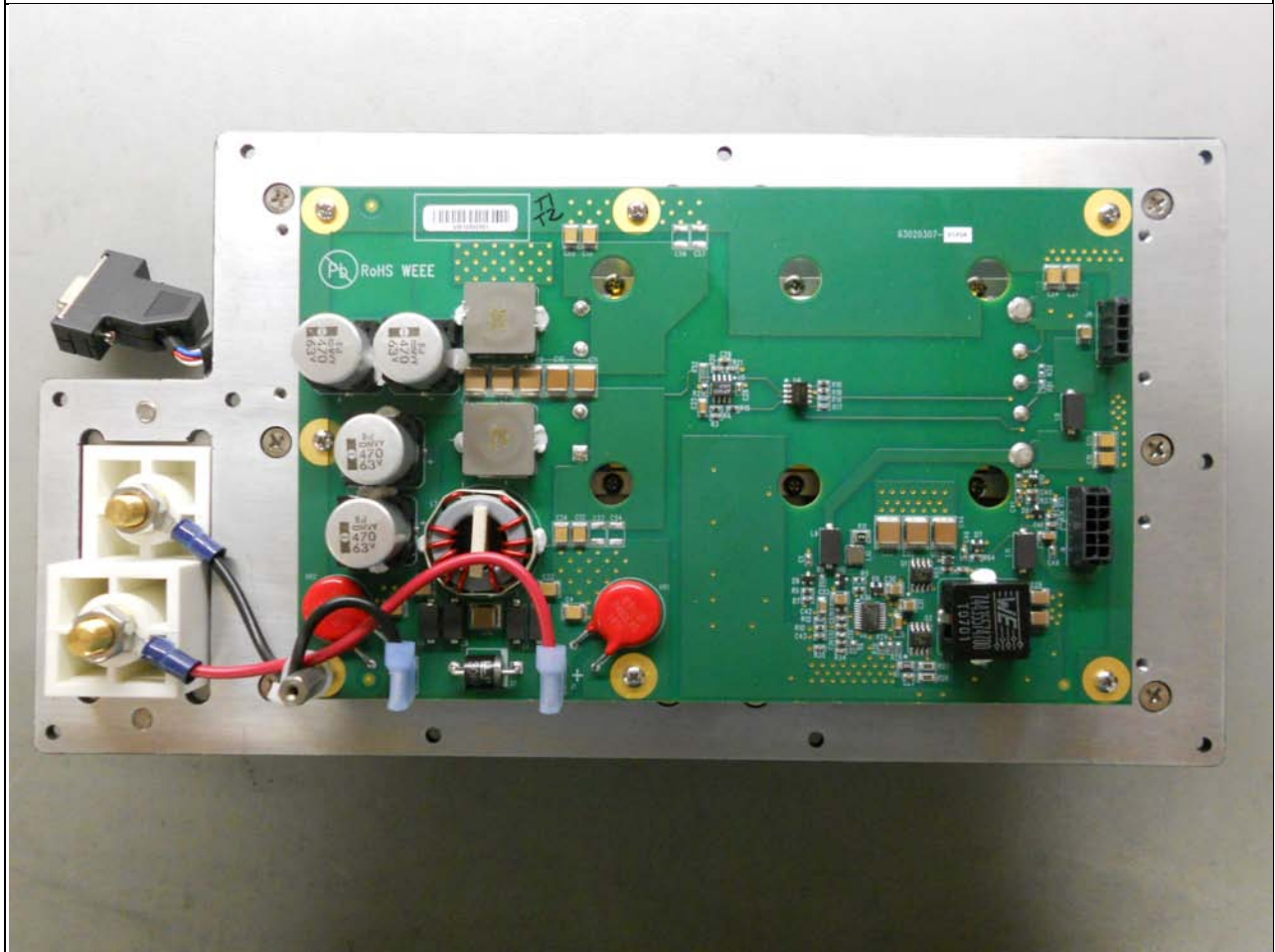
Power Supply Heatsink Assembly
