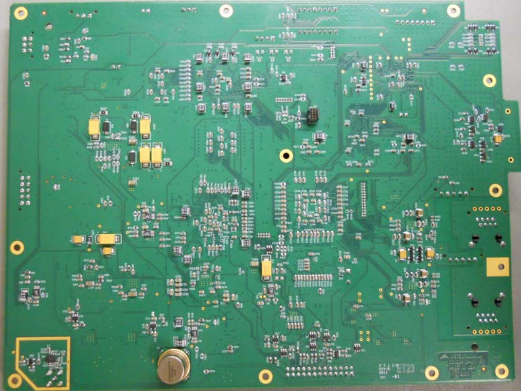
Master Board, Bottom Side
