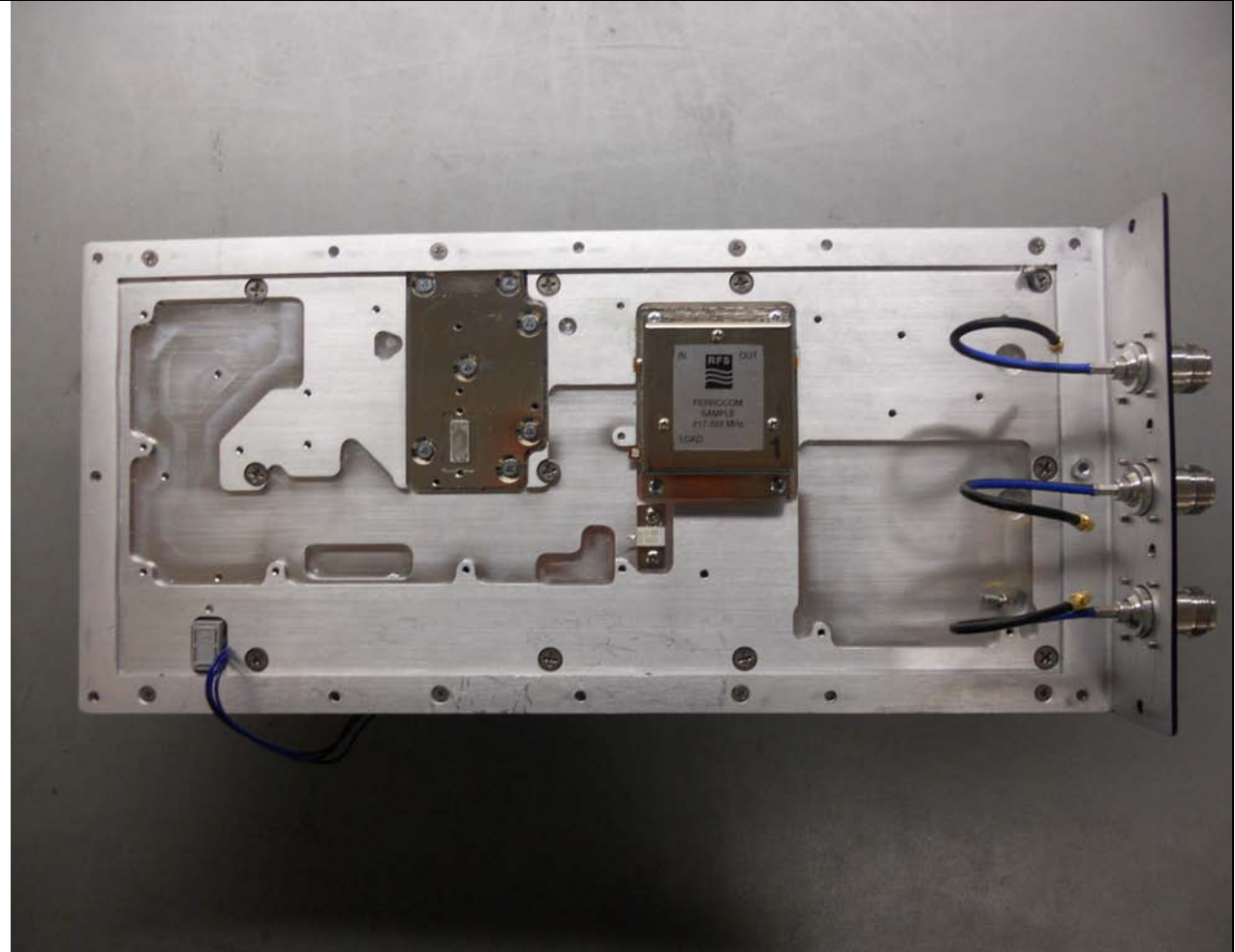
PA Heatsink with Circulator, without boards
