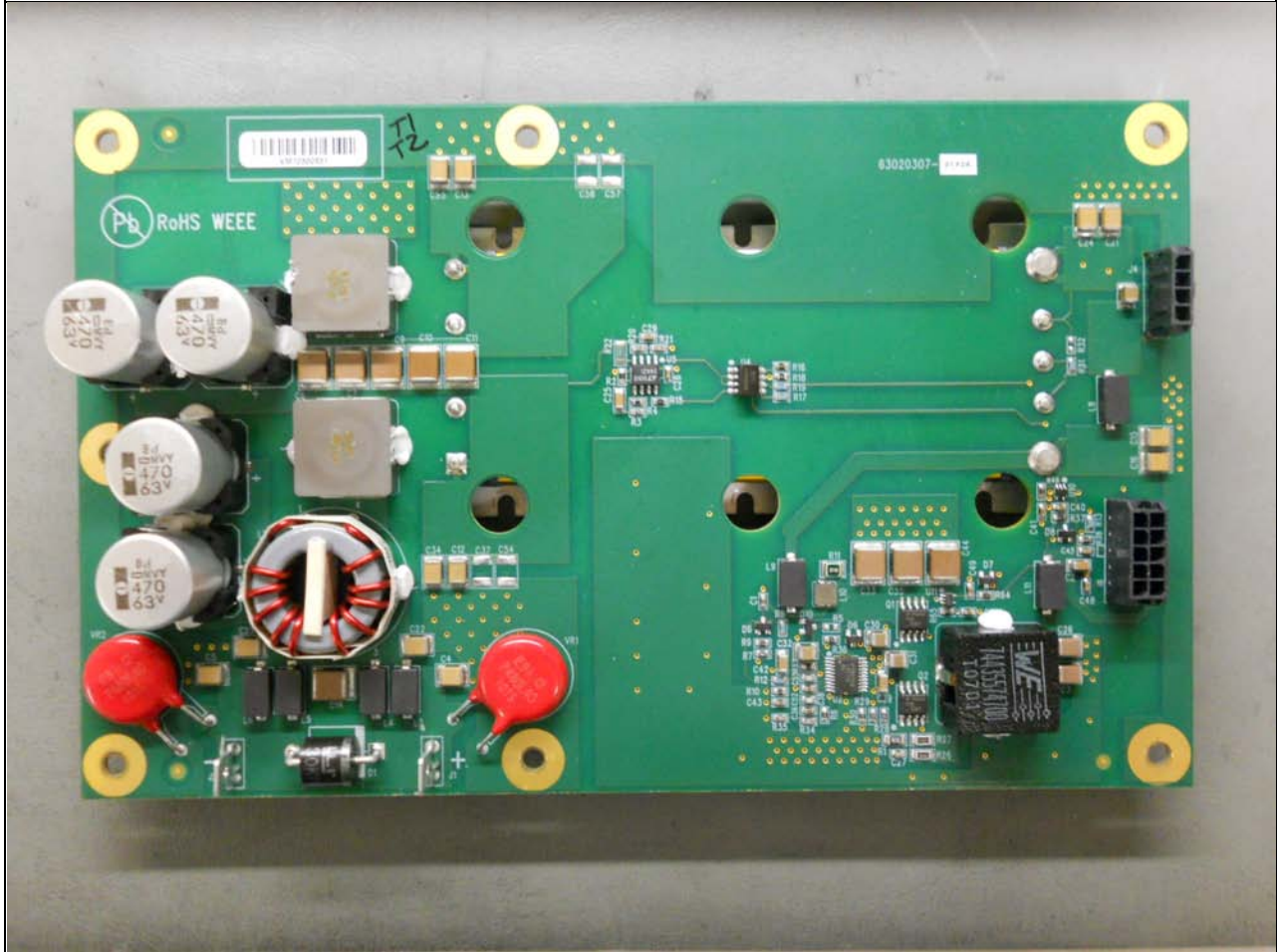
Power Supply Board, Top Side
