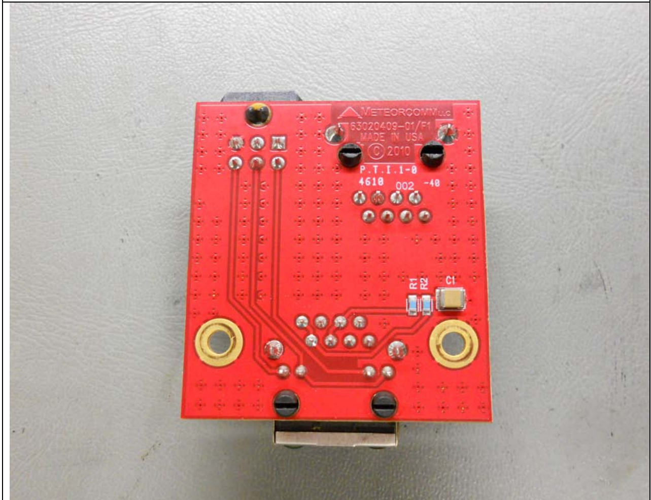
Ethernet Interface Board, Bottom Side
