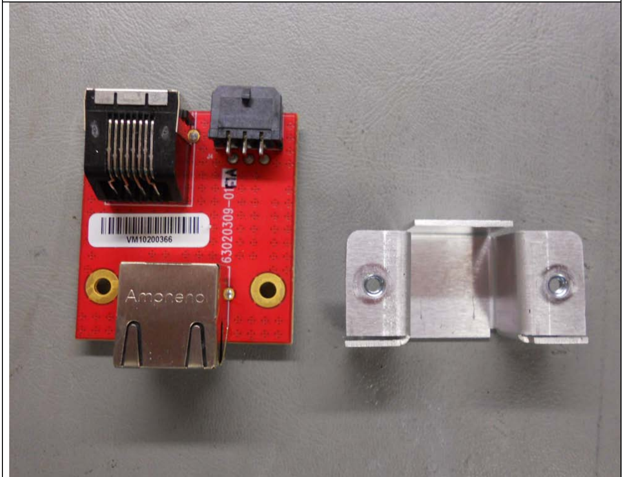
Ethernet Interface Board, Top Side
