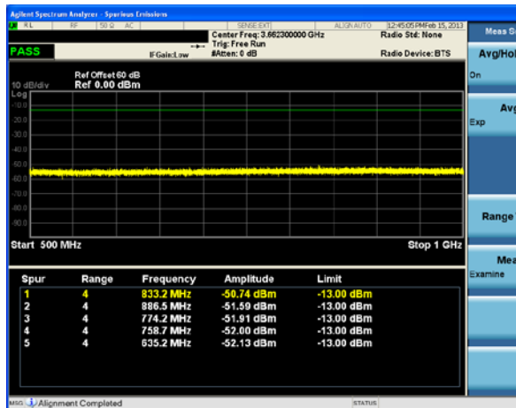
Figure 8C7 500 to 1000 MHz, 10kHz BW
