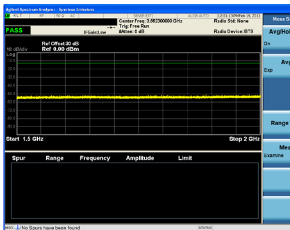
Figure 8C9 1.5 to 2 GHz, 1 MHz BW
