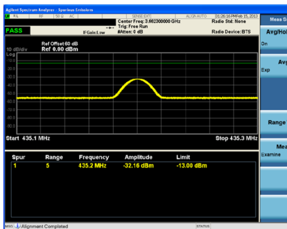
Figure 8C11, Zoom 2xfo, 435.2 MHz
