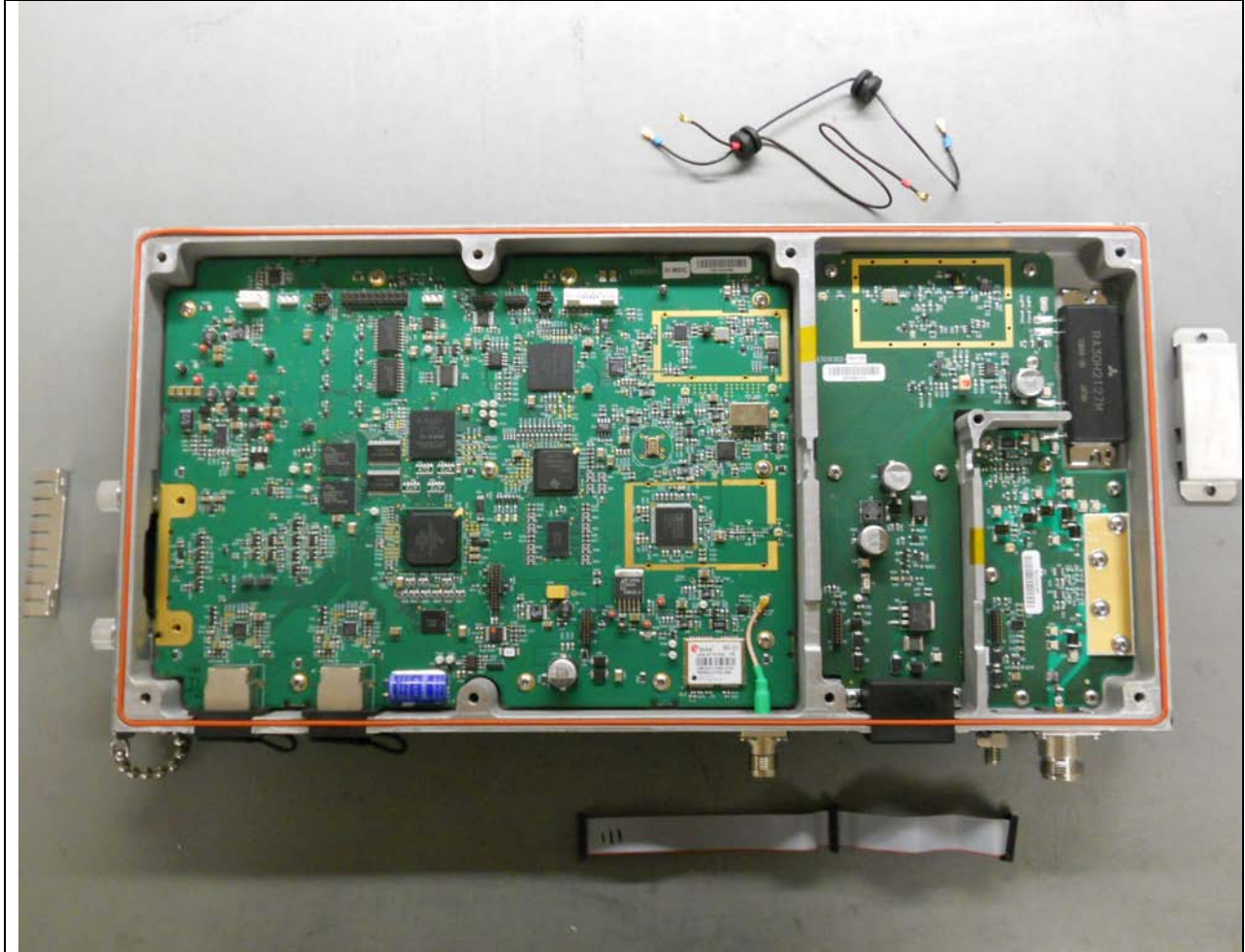
Chassis Internal View, cables & shields removed
