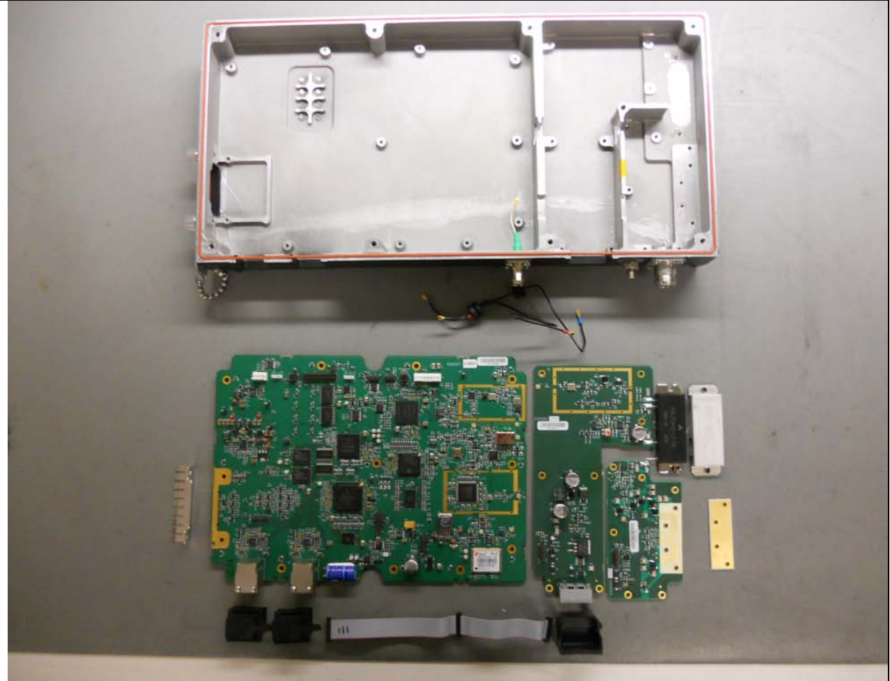
Heatsink Chassis, Exploded View
