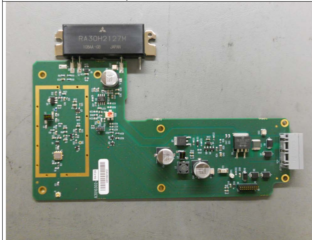
PA Board, Top View
