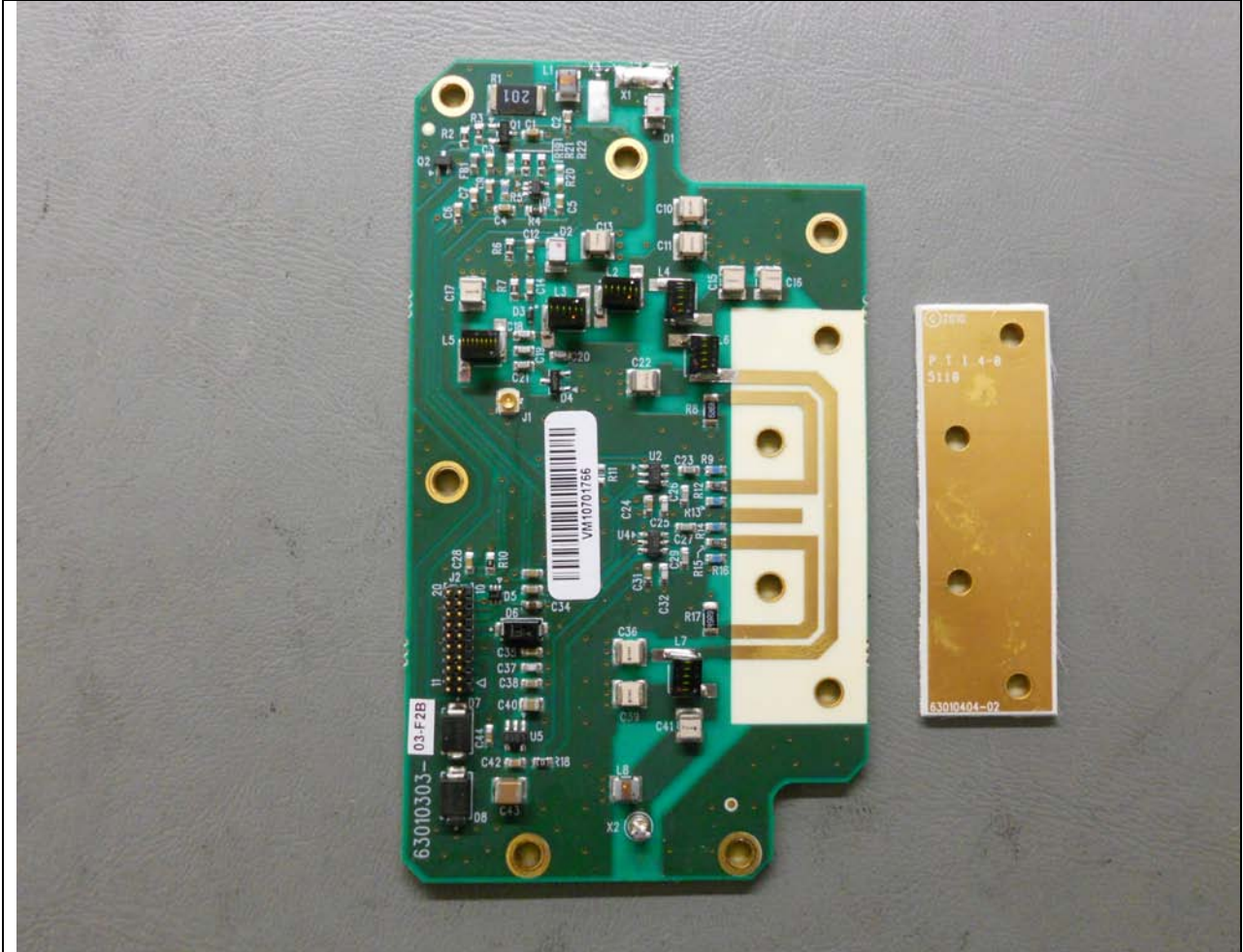
Front-End Board, Top View, RF Coupler cover removed
