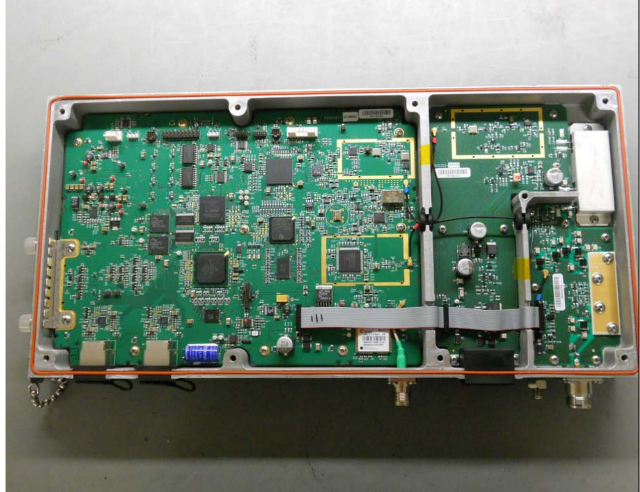
Chassis Internal View, back cover removed
