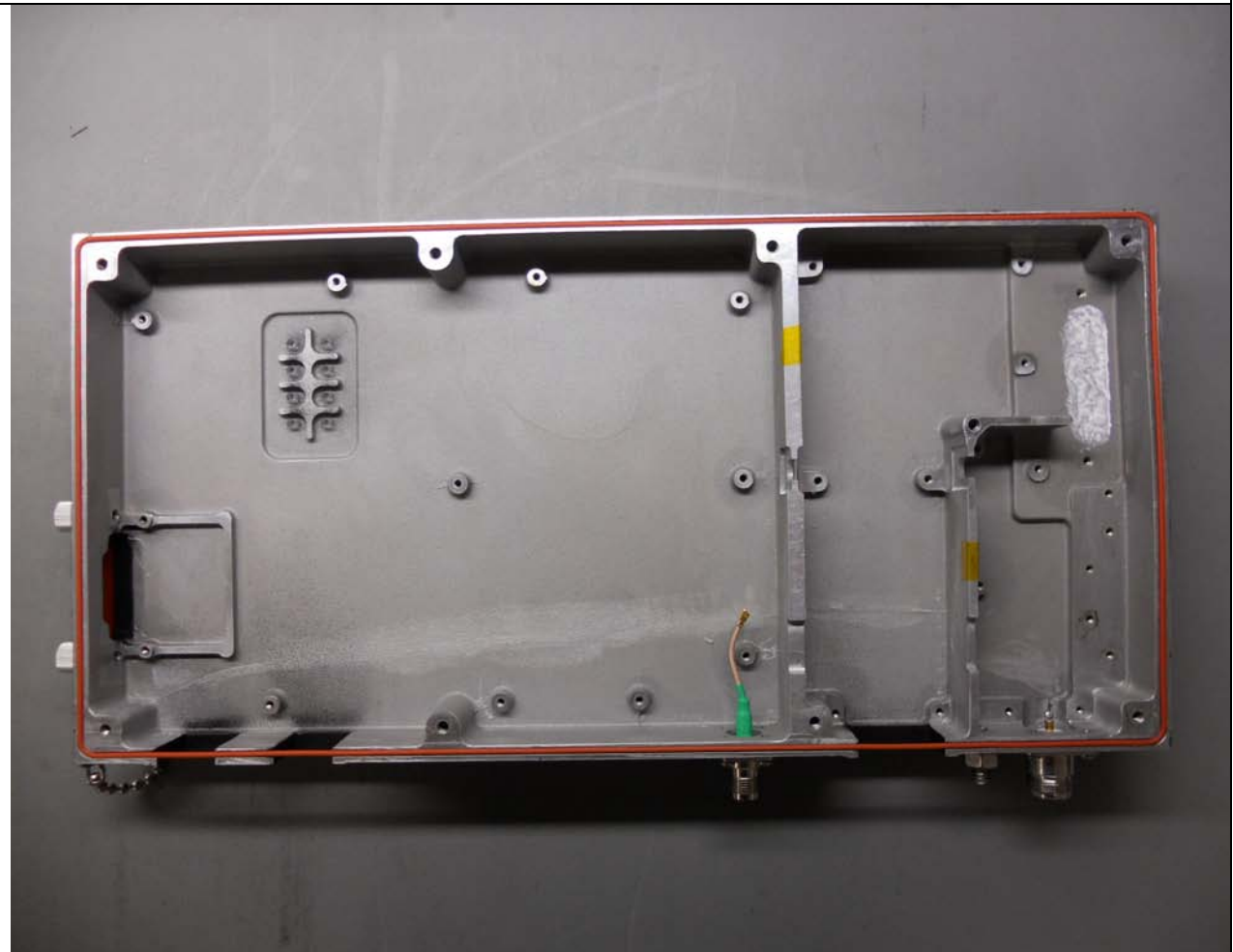
Heatsink Chassis
