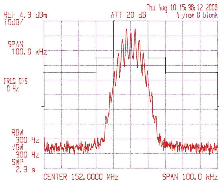
Figure 8HB3.4 Fo = 152.000 MHz, 25kHz Voice 16K0F3E, Mask B
