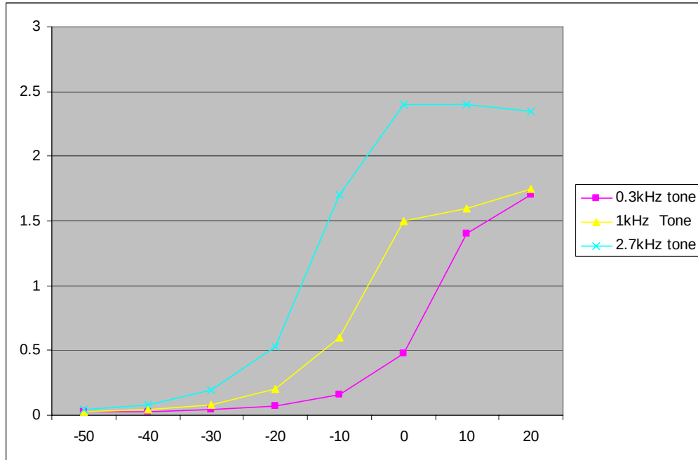
8HB.2.2.1 Modulation Limiting, 159.000 MHz, 12.5 kHz channel spacing
