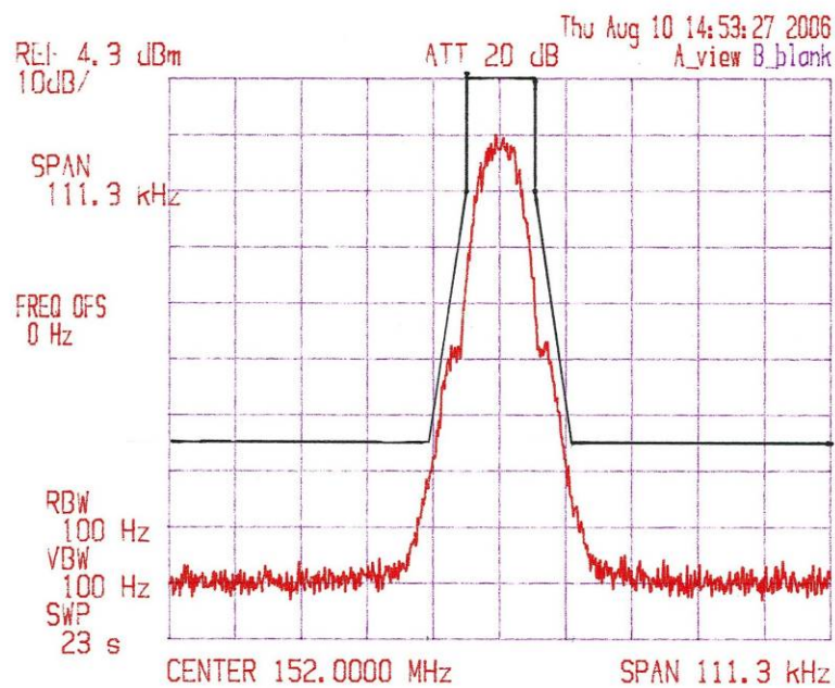
Figure 8HB3.3 F_o = 152.000 MHz, 9.6kbps GMSK BT=.30 11K0F1D, Mask D
