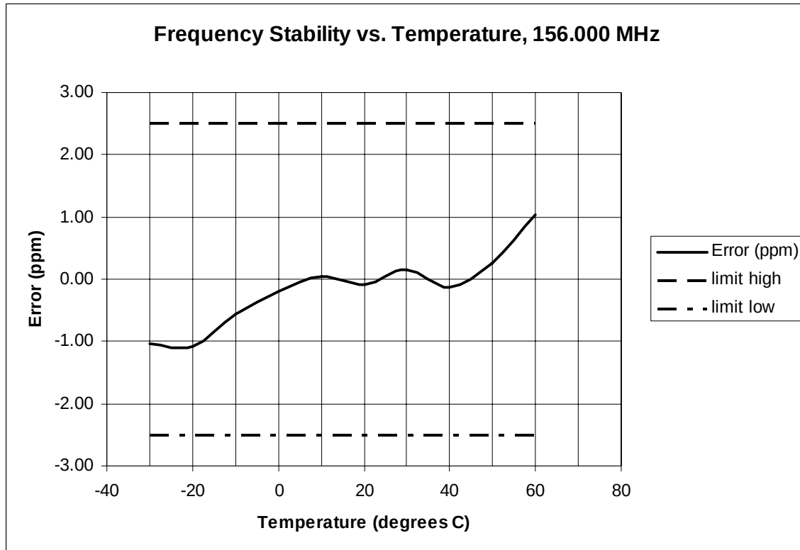
Figure 8HB.7.1 Frequency Stability vs. Temperature, fo=156.000 MHz
