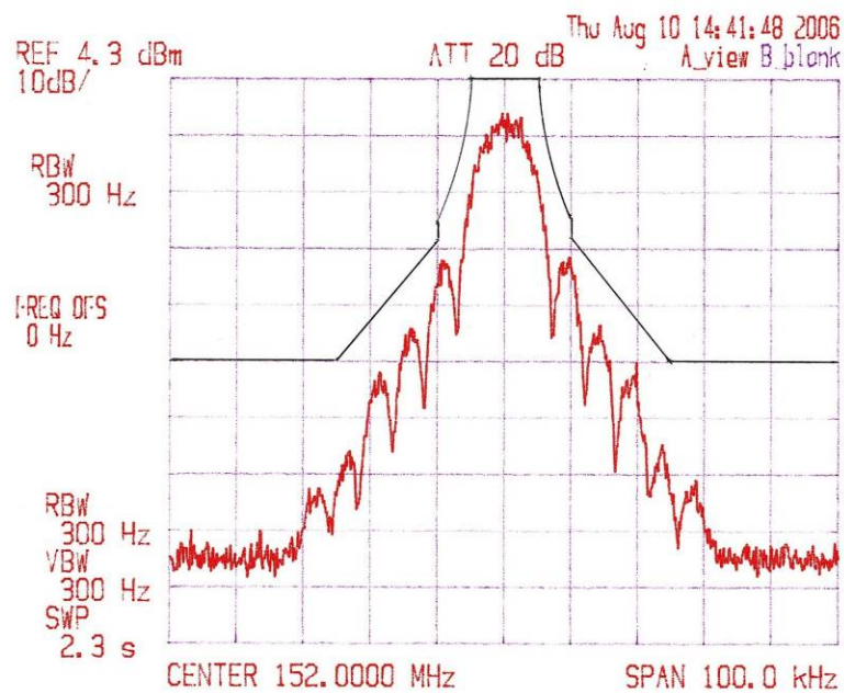
Figure 8HB3.2 F_o = 152.000 MHz, 9.6kbps GMSK BT=1.0 14K4F1D, Mask C
