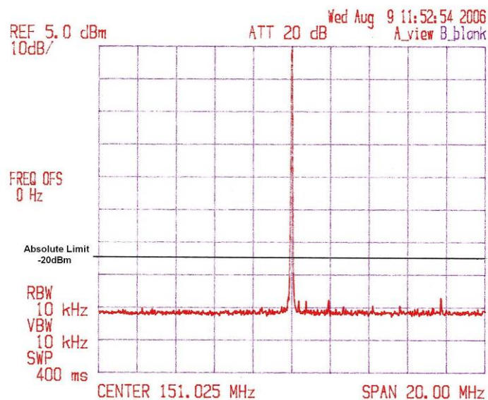
Figure 8HB.5.2 Fo=151.025 MHz, 20 MHz Span
