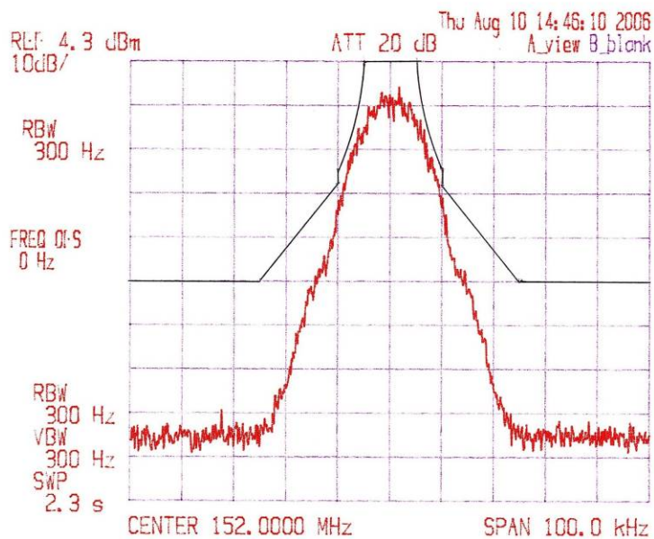
Figure 8HB3.1 Fo = 152.000 MHz, 19.2kbps GMSK BT=.22 20K0F1D, Mask C
