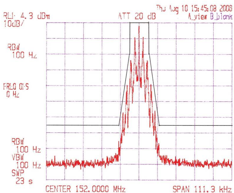
Figure 8HB3.5 Fo = 152.000 MHz, 12.5kHz Voice 11K0F3E, Mask D
