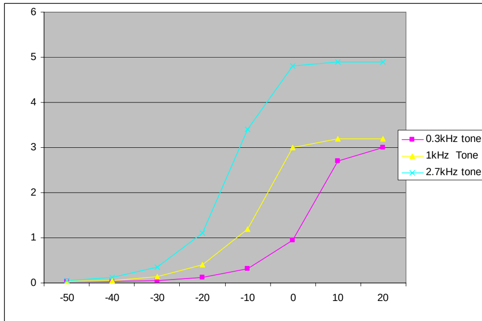
8HB.2.2.2 Modulation Limiting, 159.000 MHz, 25 kHz channel spacing
