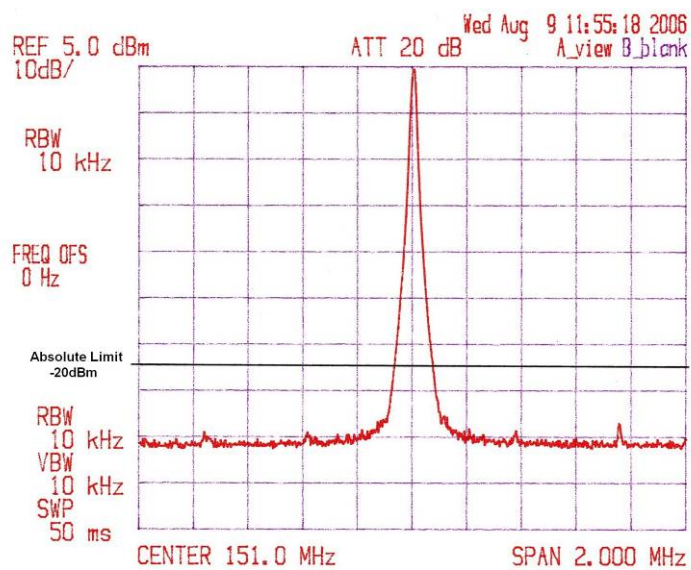
Figure 8HB.5.1 Fo=151.025 MHz, 2 MHz Span
