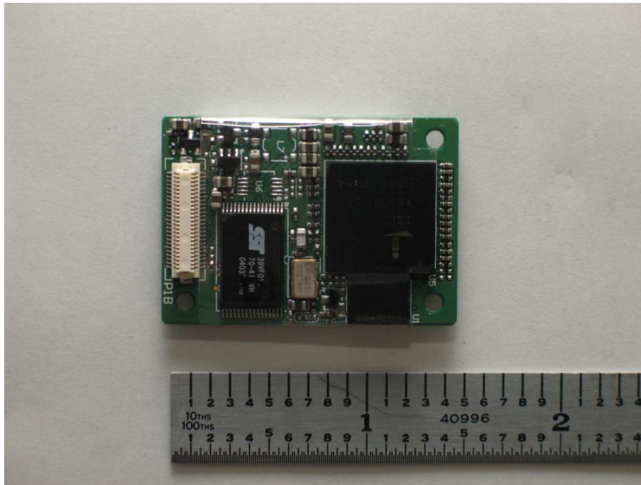
Figure 5F-1 DPAC 802.11(b) Board, top
