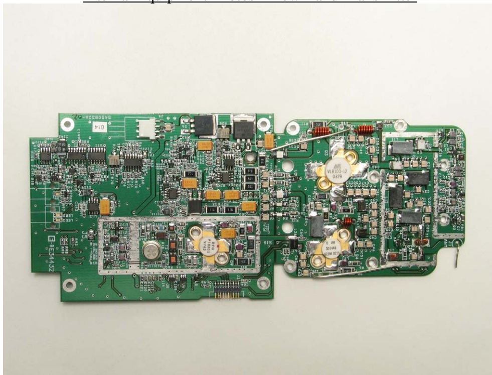
Figure 5D-1 Low Band Board, top, with shield removed
