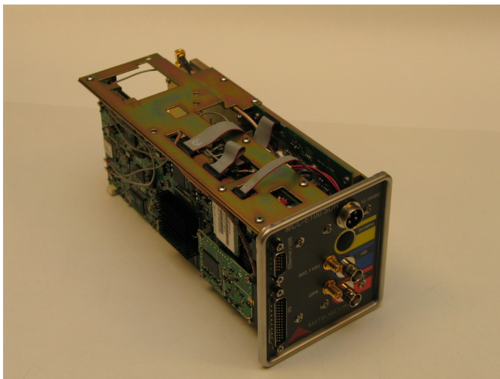
Figure 5B-3 Top side view with cover removed
