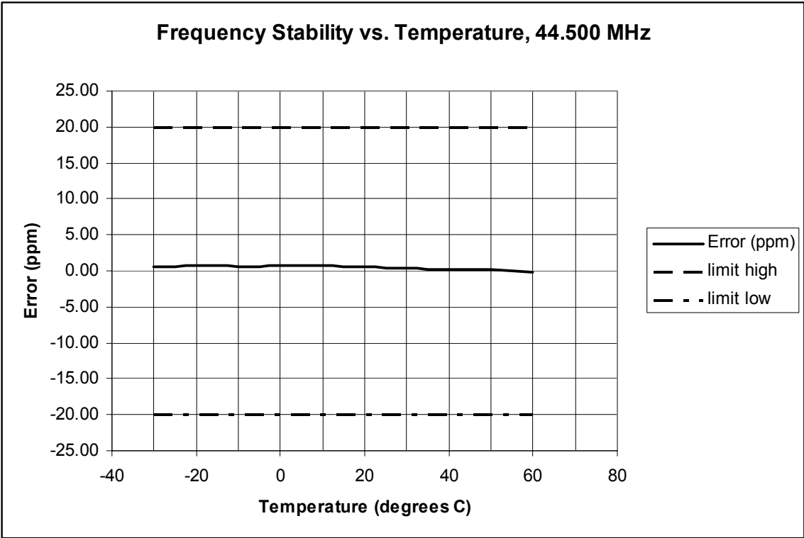
Figure 8LB.7.1 Frequency Stability vs. Temperature, fo=44.500 MHz
