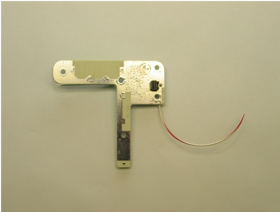
Figure 5F-4 900MHz Low Pass Filter Board, bottom
