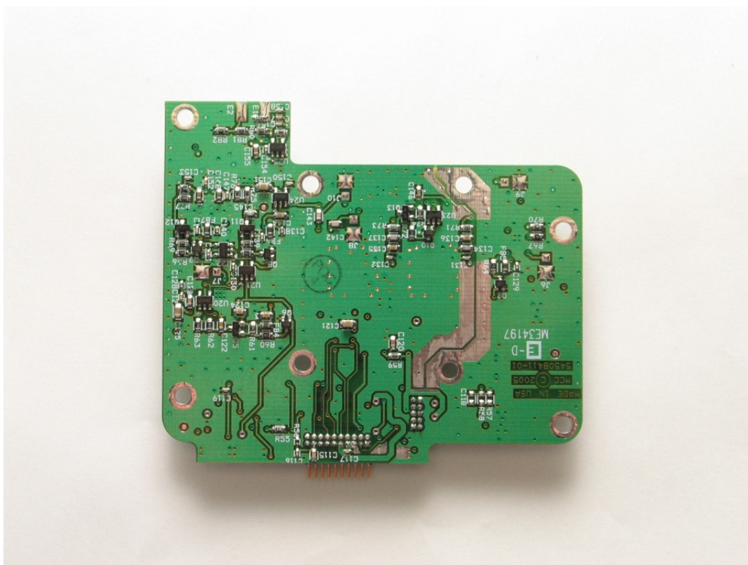
Figure 5F-2 900MHz Main Board, bottom
