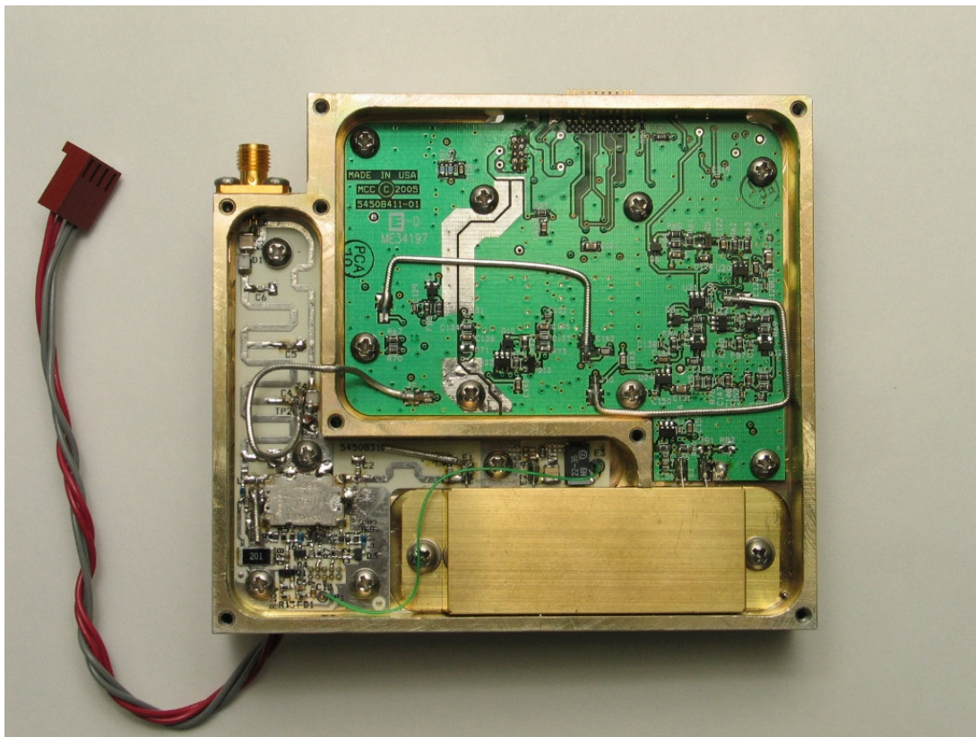
Figure 5F-6 900MHz Assembly, bottom
