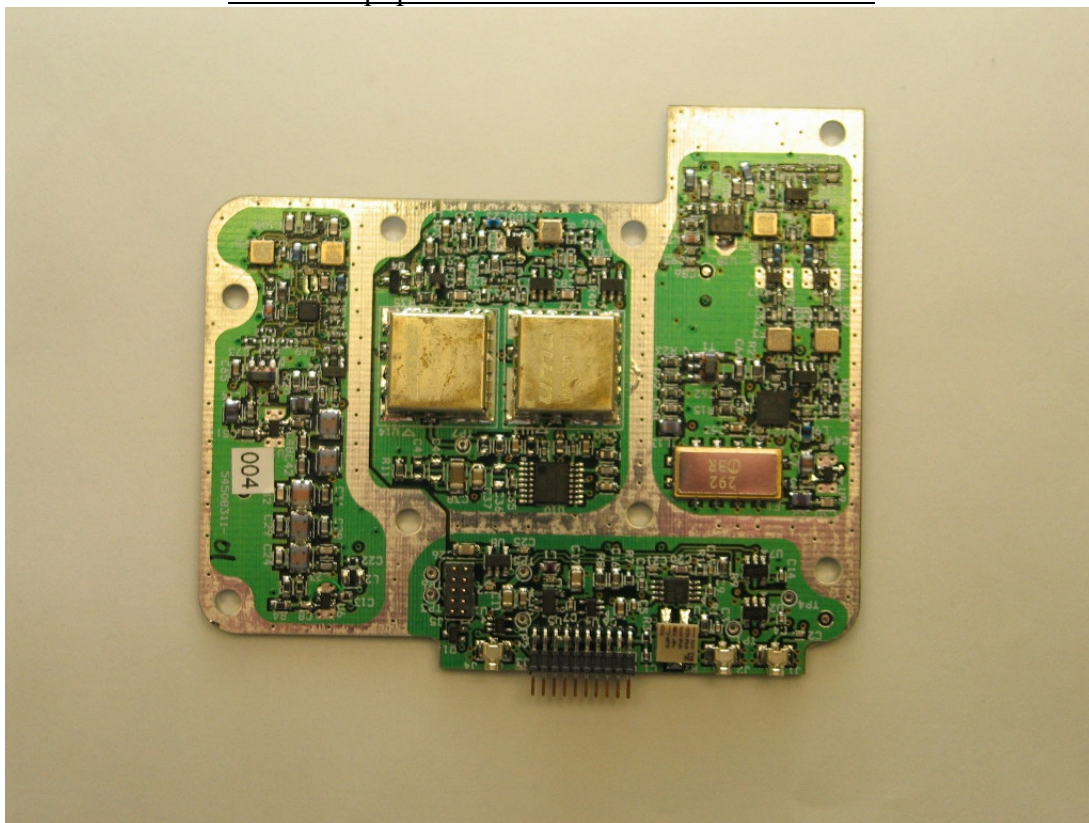
Figure 5F-1 900MHz Main Board, top
