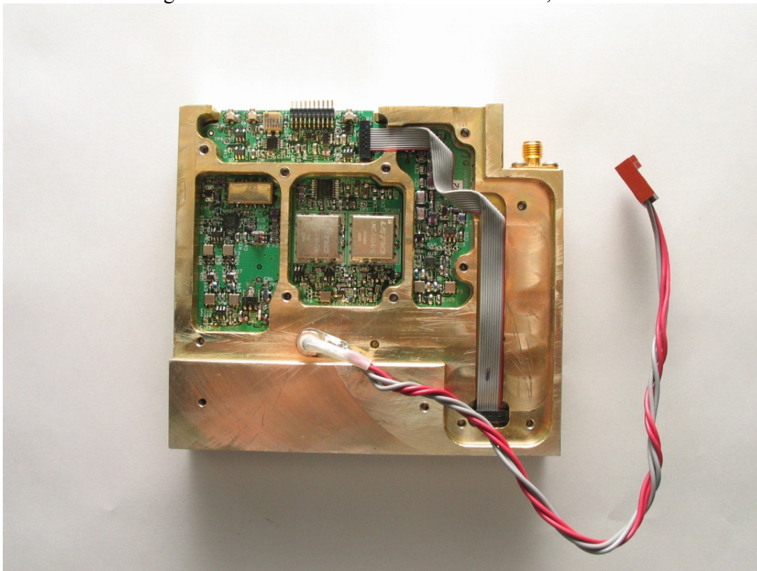
Figure 5F-5 900MHz Assembly, top
