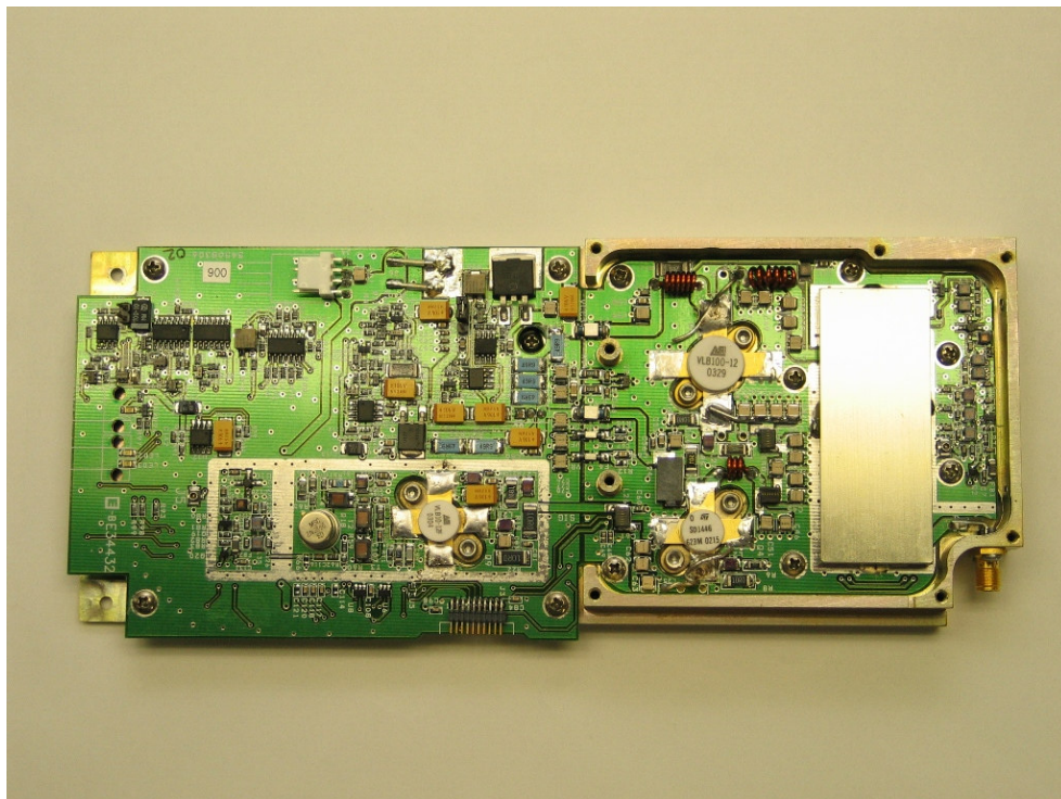
Figure 5D-4 Low Band Assembly, top, with shield installed
