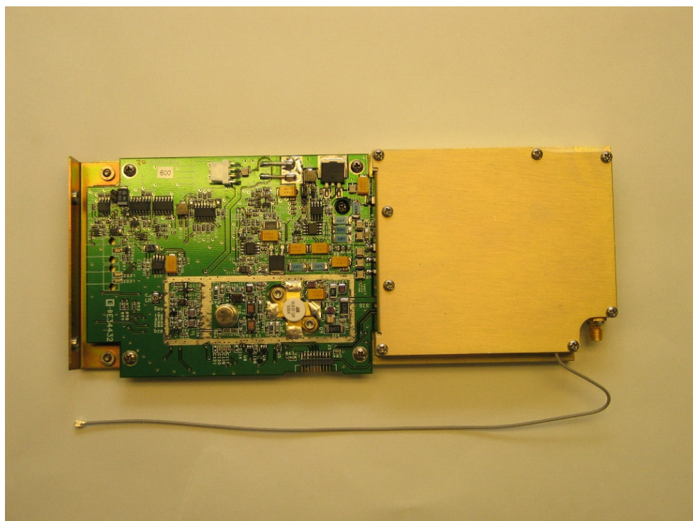
Figure 5D-2 Low Band Assembly, top, with cover installed
