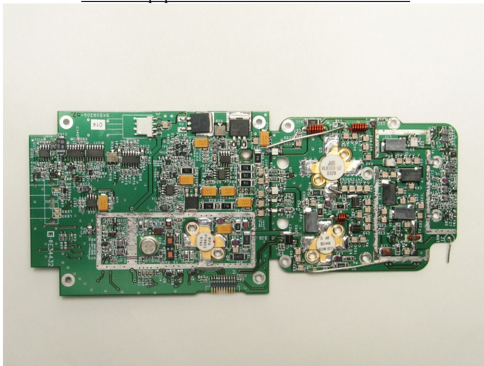
Figure 5D-1 Low Band Board, top, with shield removed
