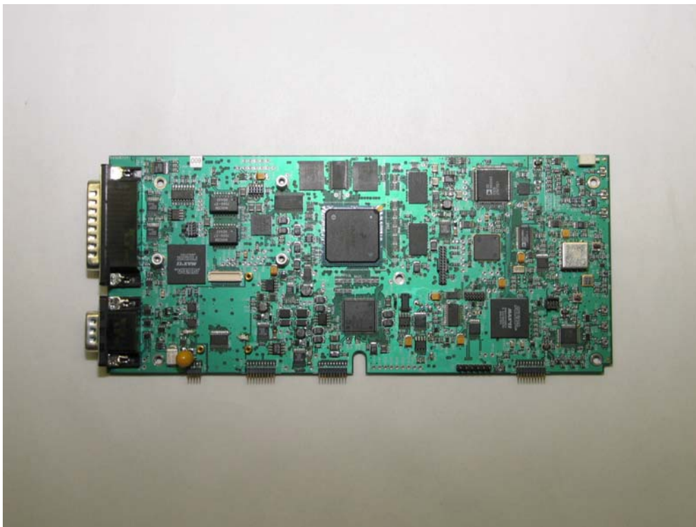
Figure 5C-2 CMU Board, top, with 802.11(b) and GPS modules removed
