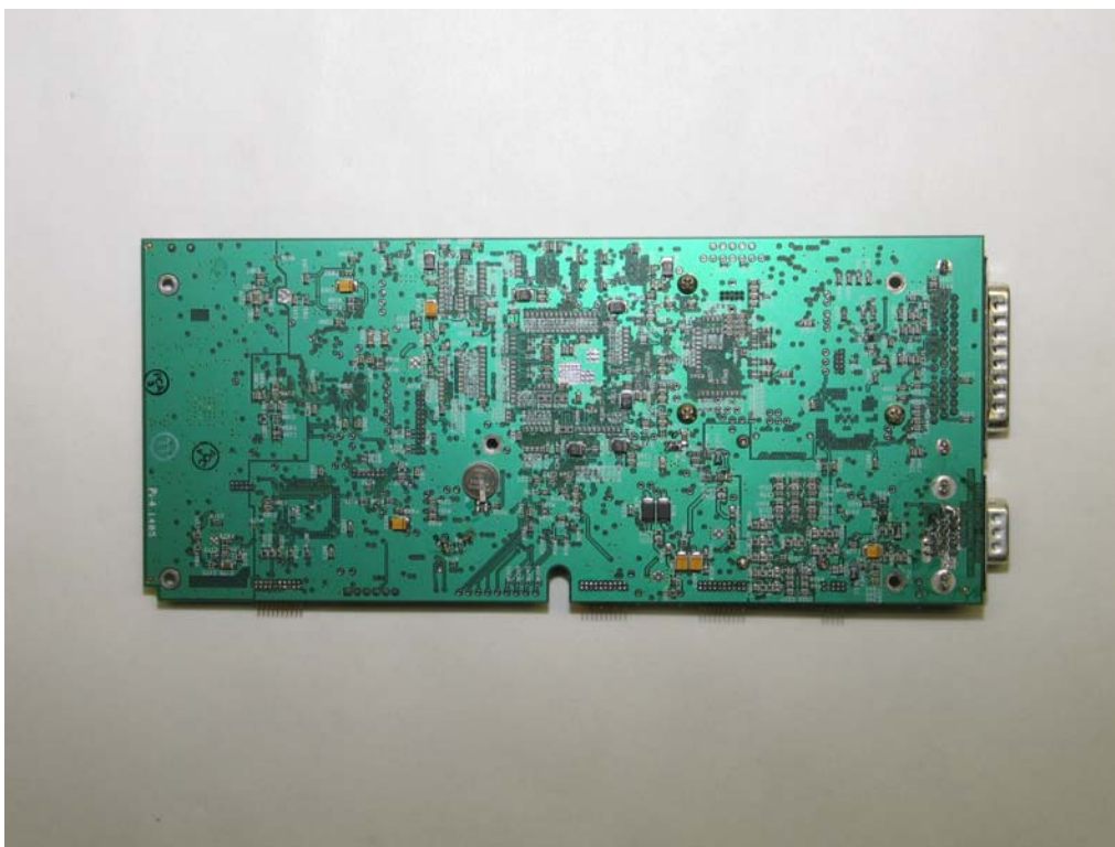
Figure 5C-3 CMU Board, bottom
