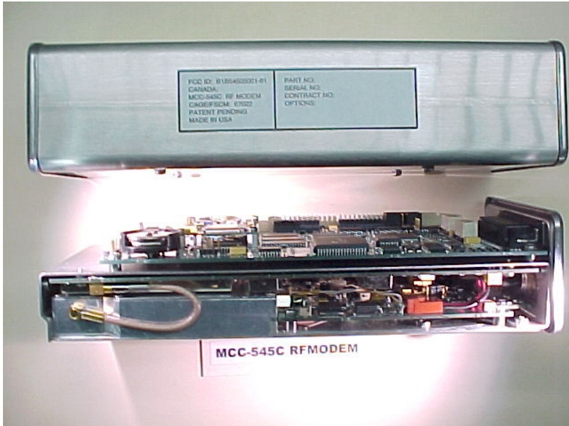
Photo 1. Top view cover on FCC ID Label location and removed
