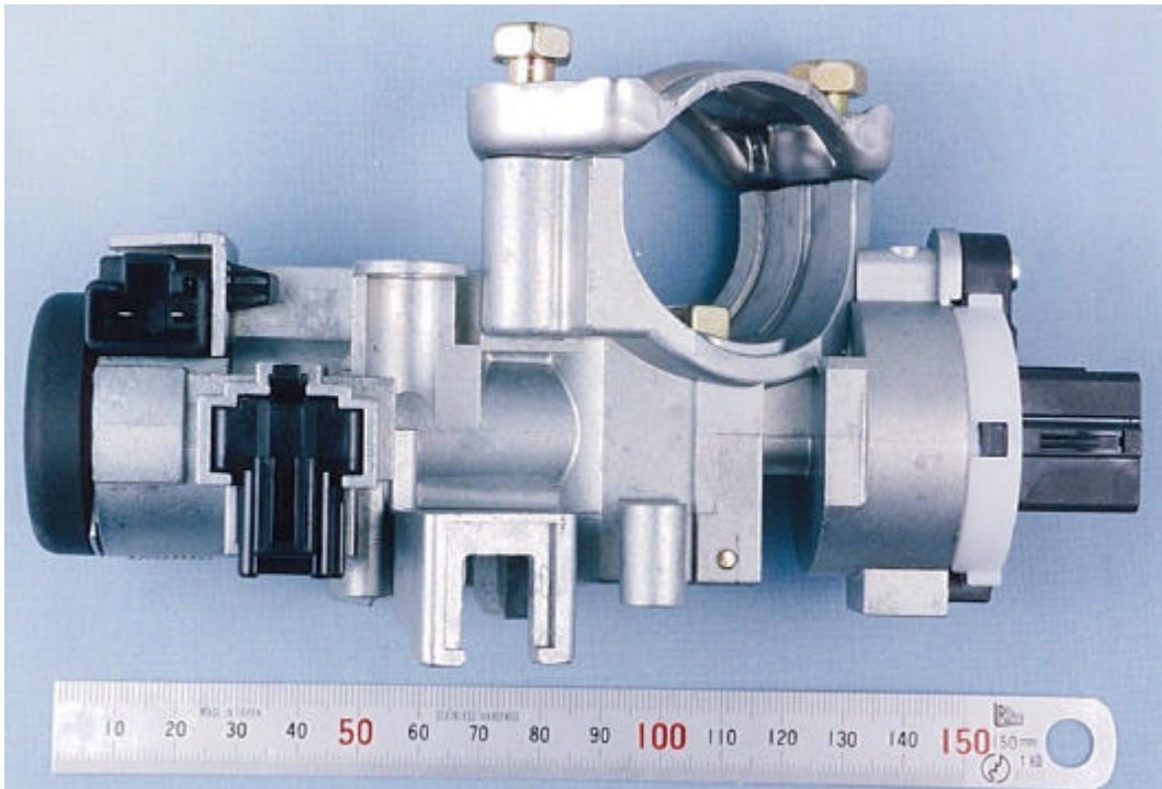
Immobilizer Antenna (type 1: X1T25271)
