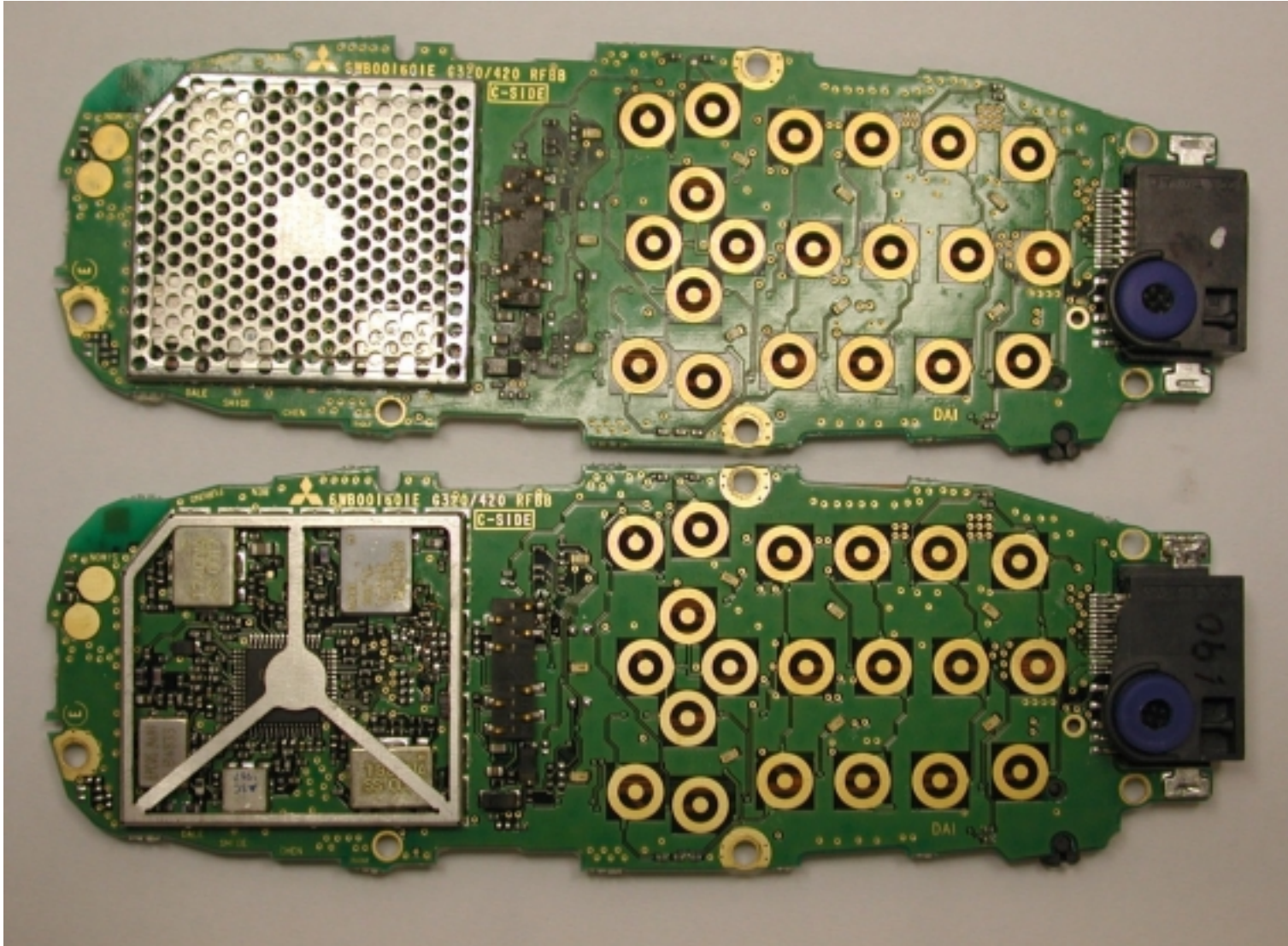
Photograph 8 MT289XG01A (Front PWB with One-Piece Shield and Two-Piece Shields With Cover Removed)
