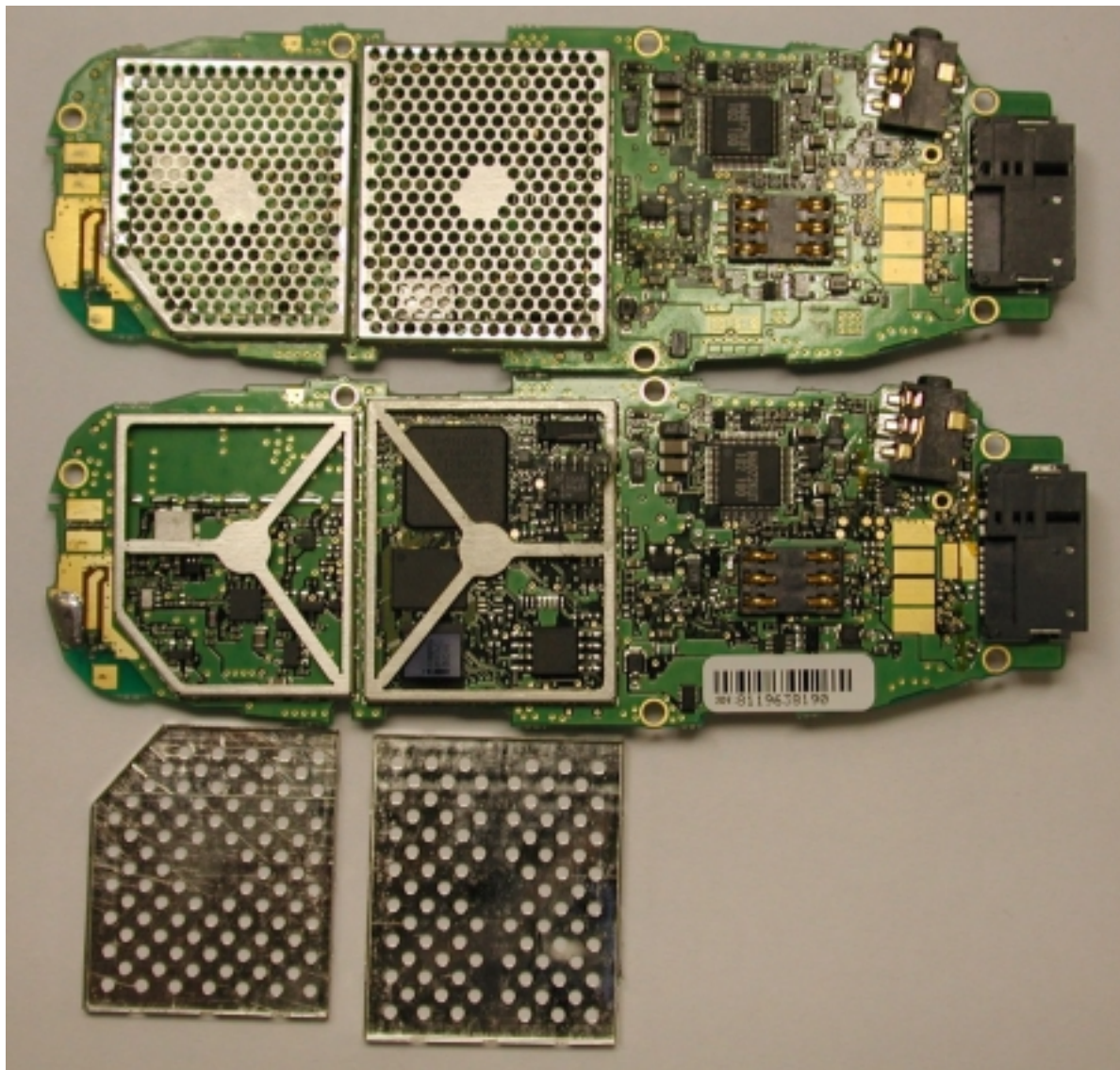
Photograph 7 MT289XG01A (Back PWB with One-Piece Shield and Two-Piece Shields With Cover Removed)
