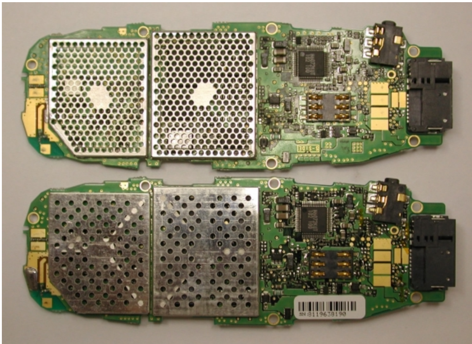
Photograph 6 MT289XG01A (Back PWB with One-Piece and Two-Piece Shields)
