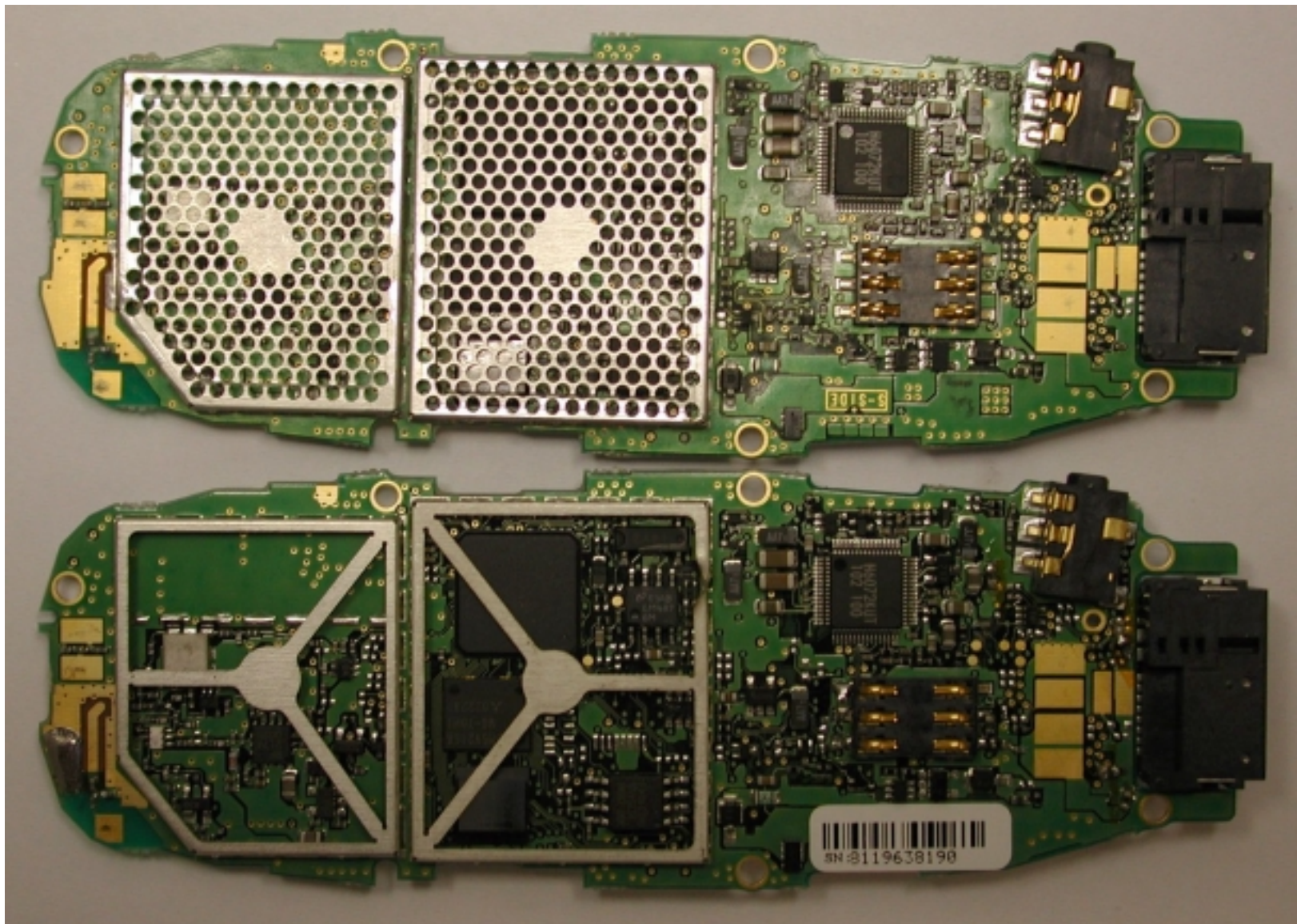
Photograph 9 MT289XG01 (Back PWB with One-Piece Shield and Two-Piece Shields With Cover Removed)
