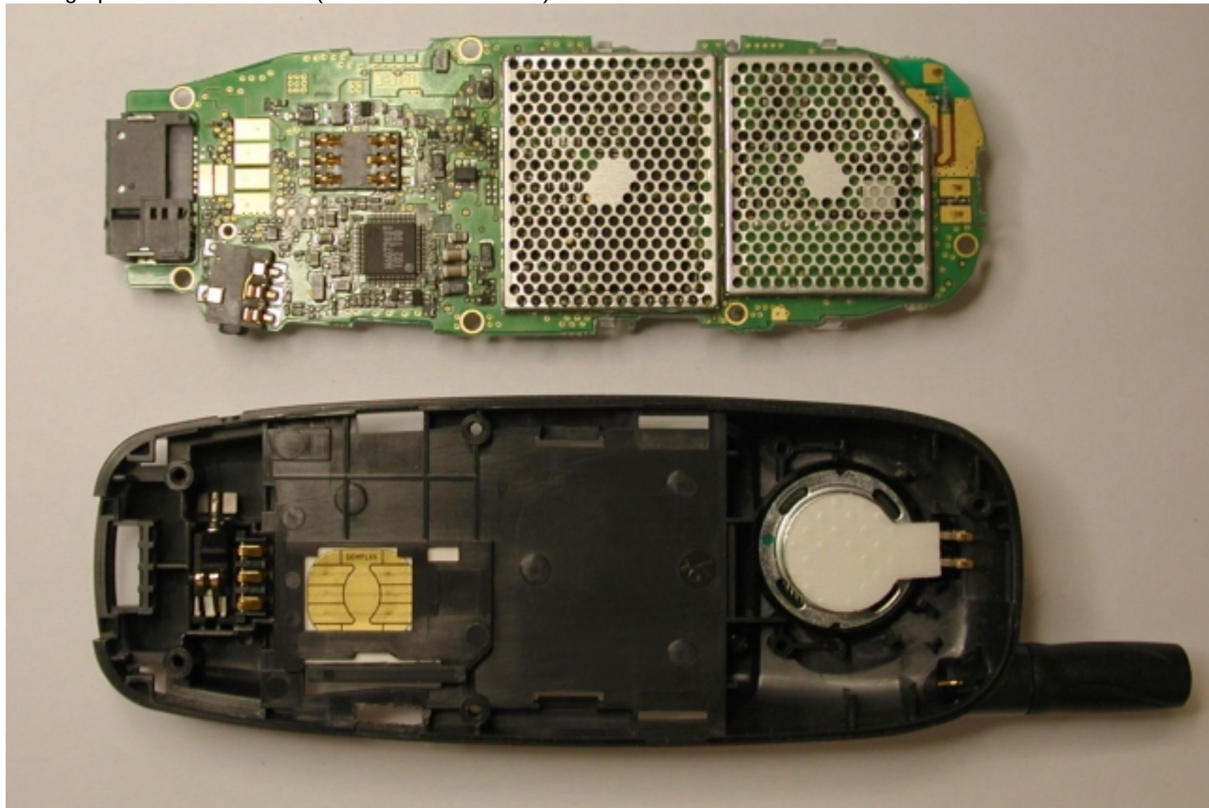
Photograph 1 MT289XG01A (Back Cover Removed)
