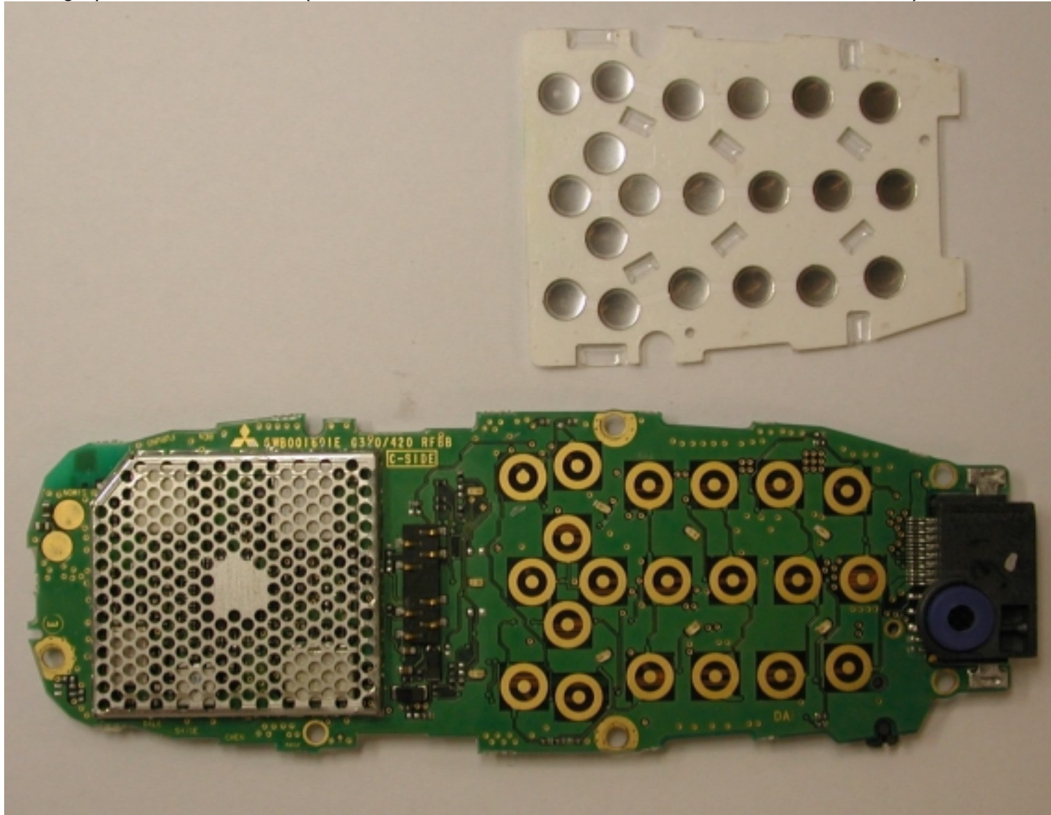
Photograph 5 MT289XG01A (Front PWB with One-Piece Shield and Metal Dome Removed)
