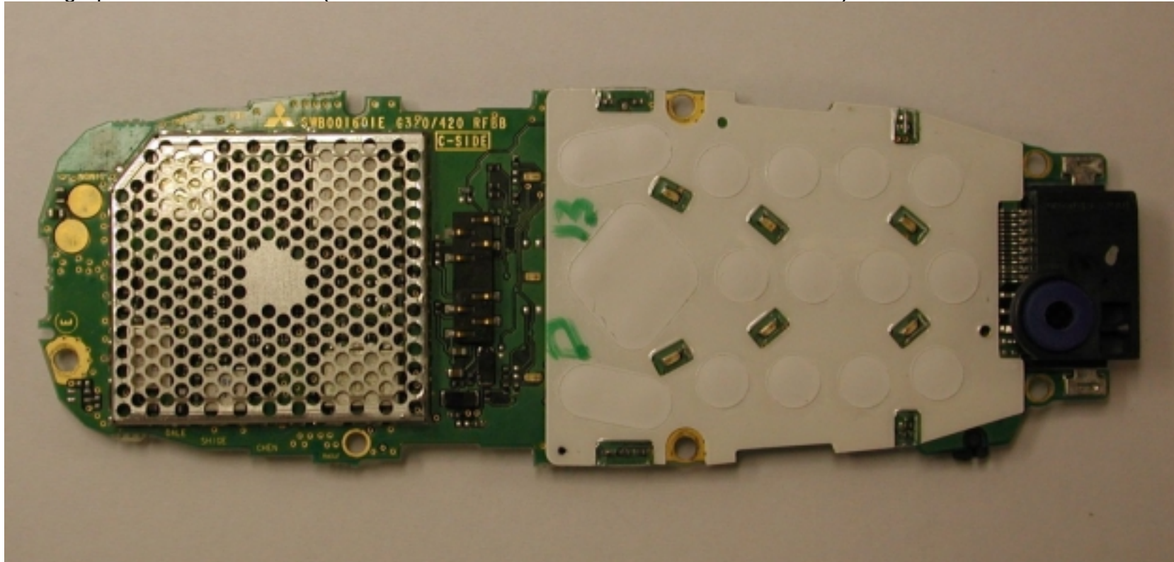
Photograph 4 MT289XG01A (Front PWB with One-Piece Shield and Metal Dome)
