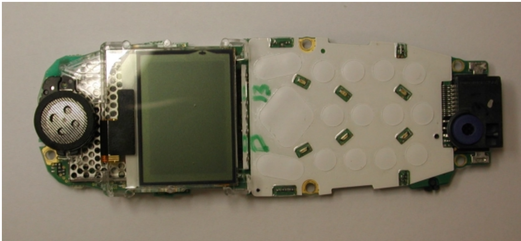
Photograph 3 MT289XG01A (Front PWB LCD and Metal Dome Installed)
