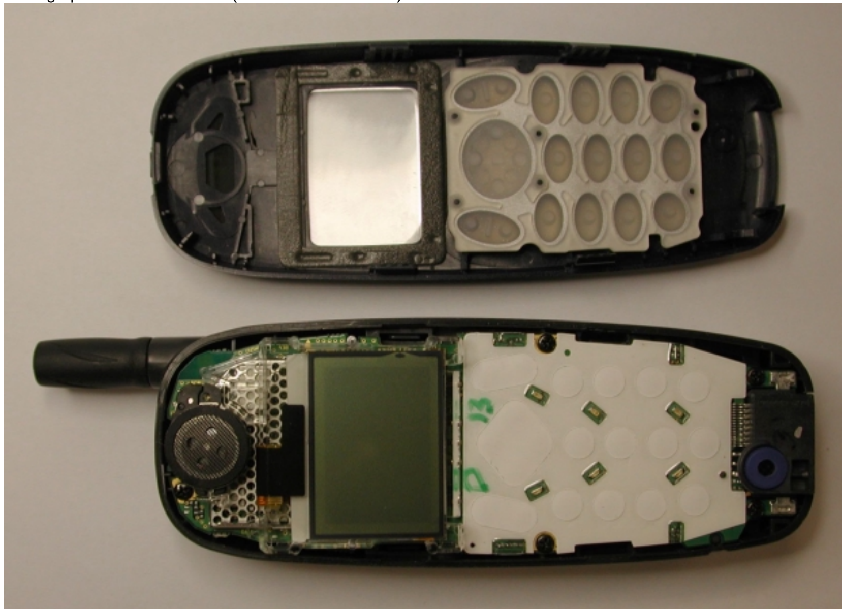
Photograph 2 MT289XG01A (Front Cover Removed)
