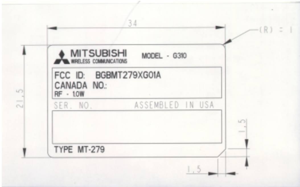
Figure 7.1.1 Identification Plate Drawing
