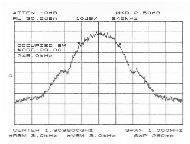
Figure 5.4.12 Block C Upper Edge 99% Power Occupied Bandwidth (Ch 810)
