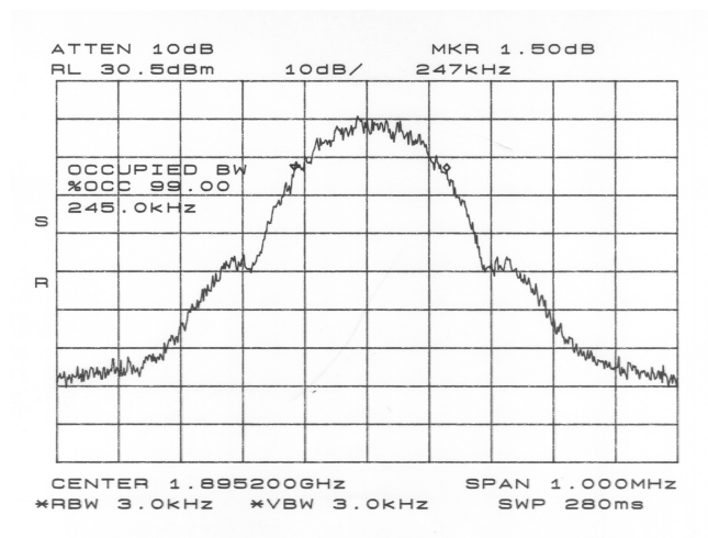
Figure 5.4.11 Block C Lower Edge 99% Power Occupied Bandwidth (Ch 737)
