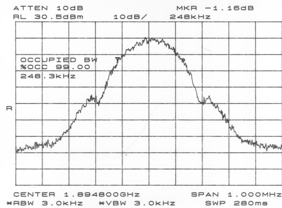
Figure 5.4.10 Block F Upper Edge 99% Power Occupied Bandwidth (Ch 735)
