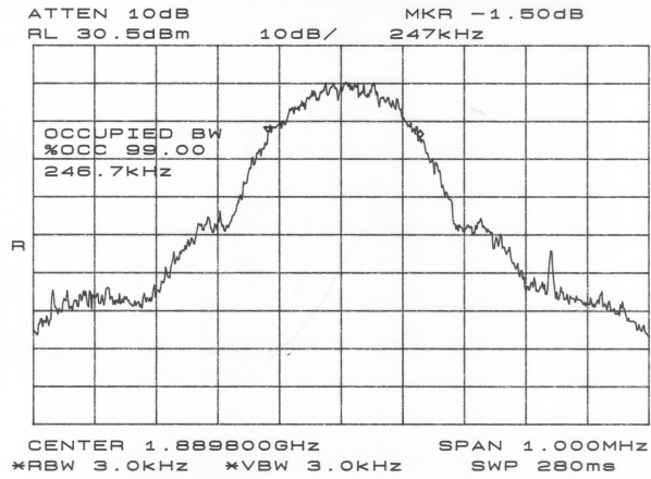
Figure 5.4.8 Block E Upper Edge 99% Power Occupied Bandwidth (Ch 710)
