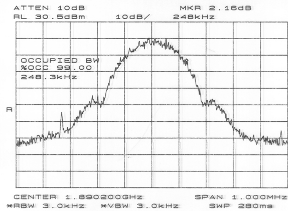
Figure 5.4.9 Block F Lower Edge 99% Power Occupied Bandwidth (Ch 712)
