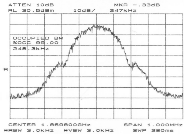
Figure 5.4.4 Block D Upper Edge 99% Power Occupied Bandwidth (Ch 610)
