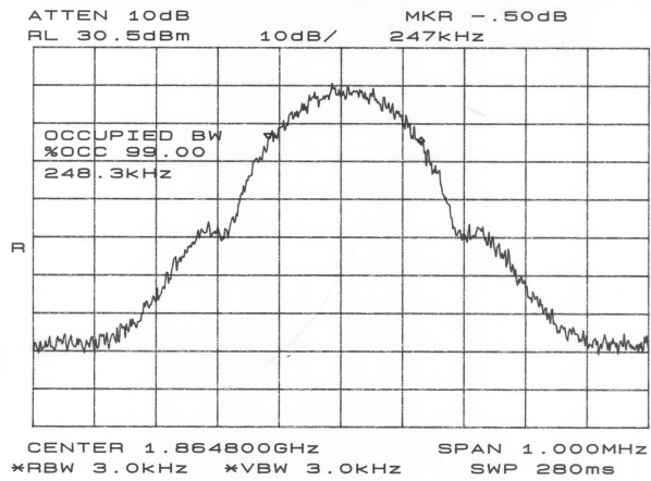
Figure 5.4.2 Block A Upper Edge 99% Power Occupied Bandwidth (Ch 585)
