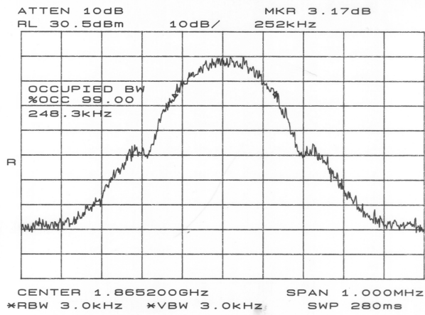
Figure 5.4.3 Block D Lower Edge 99% Power Occupied Bandwidth (Ch 587)
