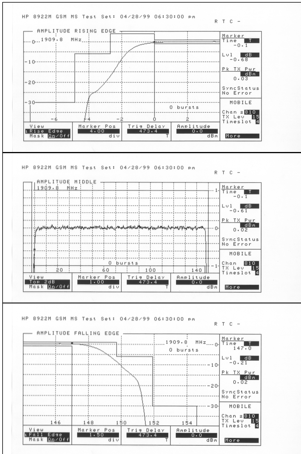
Figure 5.2.9 Carrier 1909.8 MHz (Ch 810) Power Level 15
