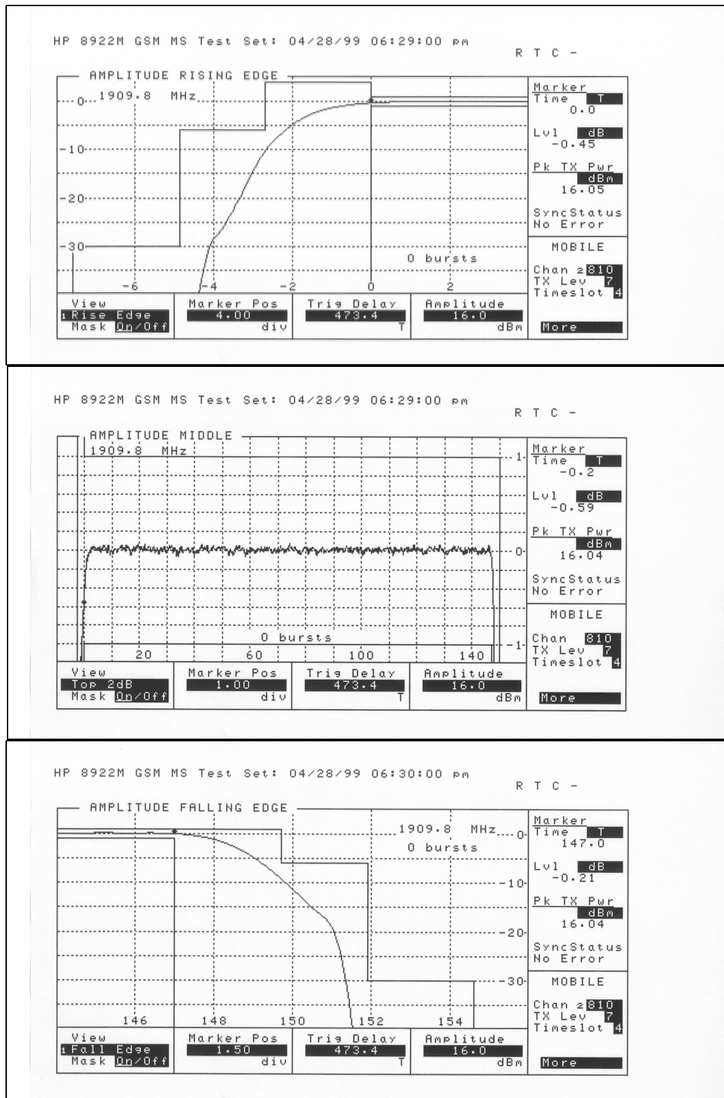
Figure 5.2.8 Carrier 1909.8 MHz (Ch 810) Power Level 7
