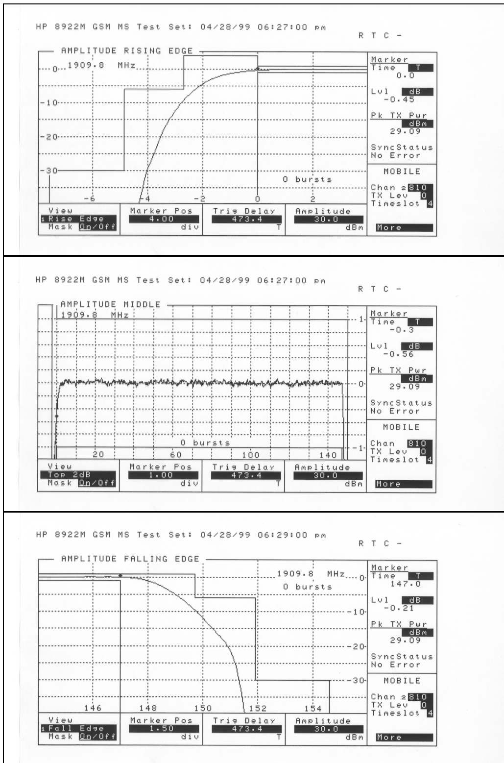
Figure 5.2.7 Carrier 1909.8 MHz (Ch 810) Power Level 0
