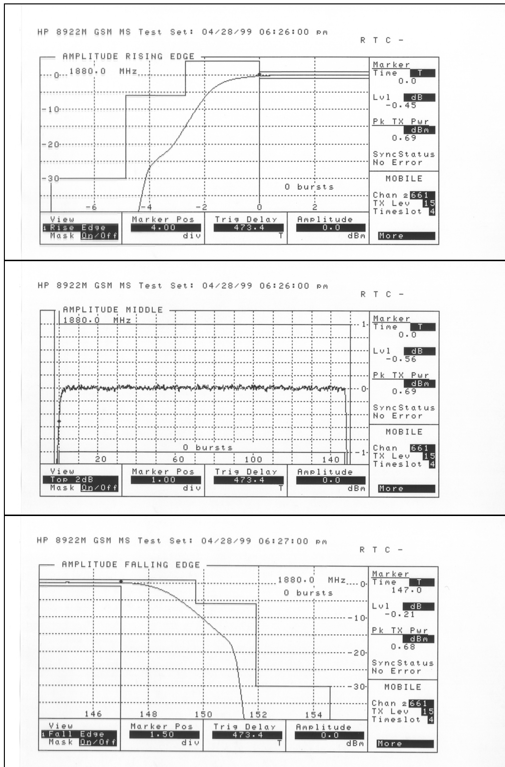
Figure 5.2.6 Carrier 1880.0 MHz (Ch 661) Power Level 15
