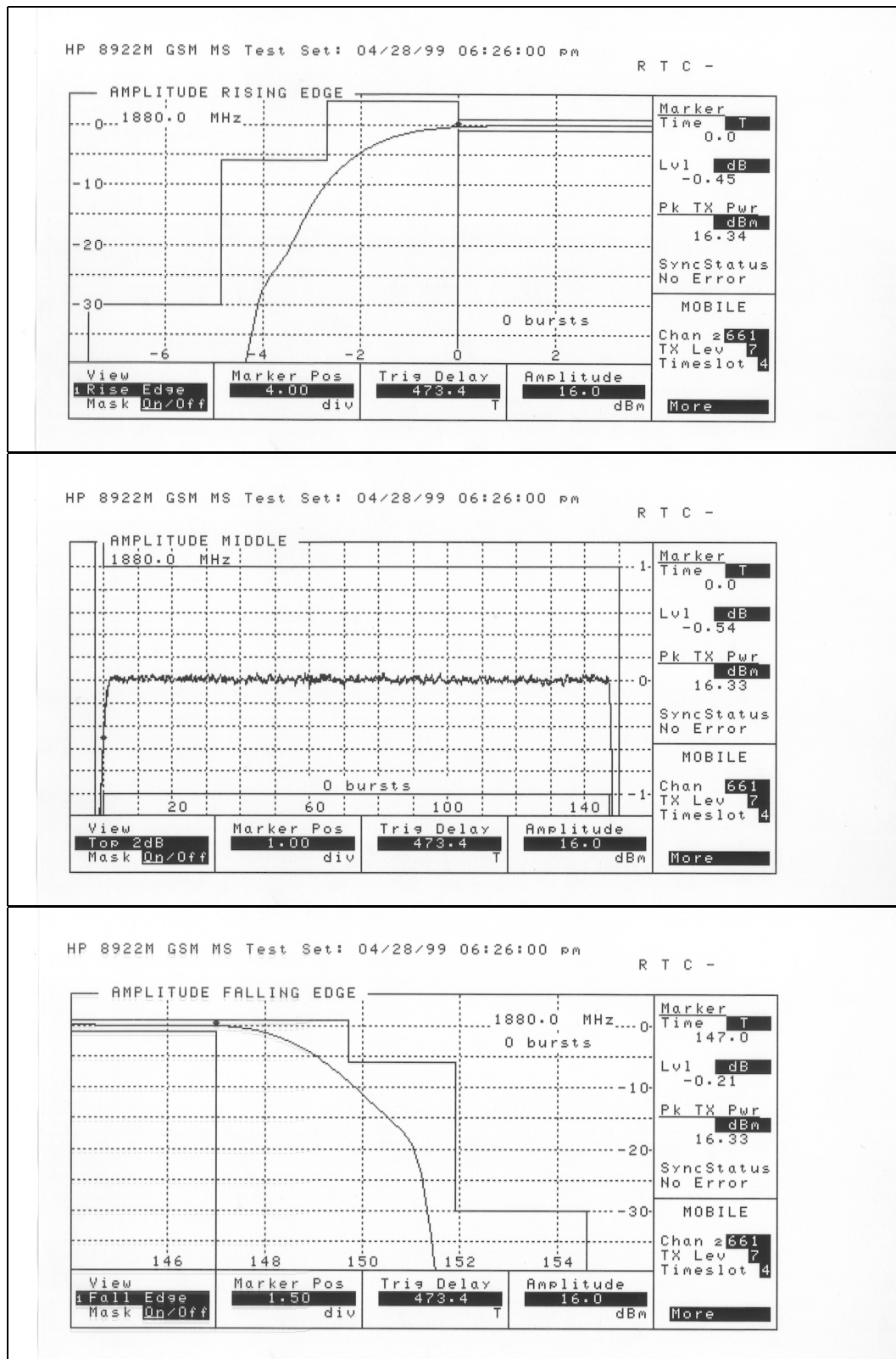
Figure 5.2.5 Carrier 1880.0 MHz (Ch 661) Power Level 7
