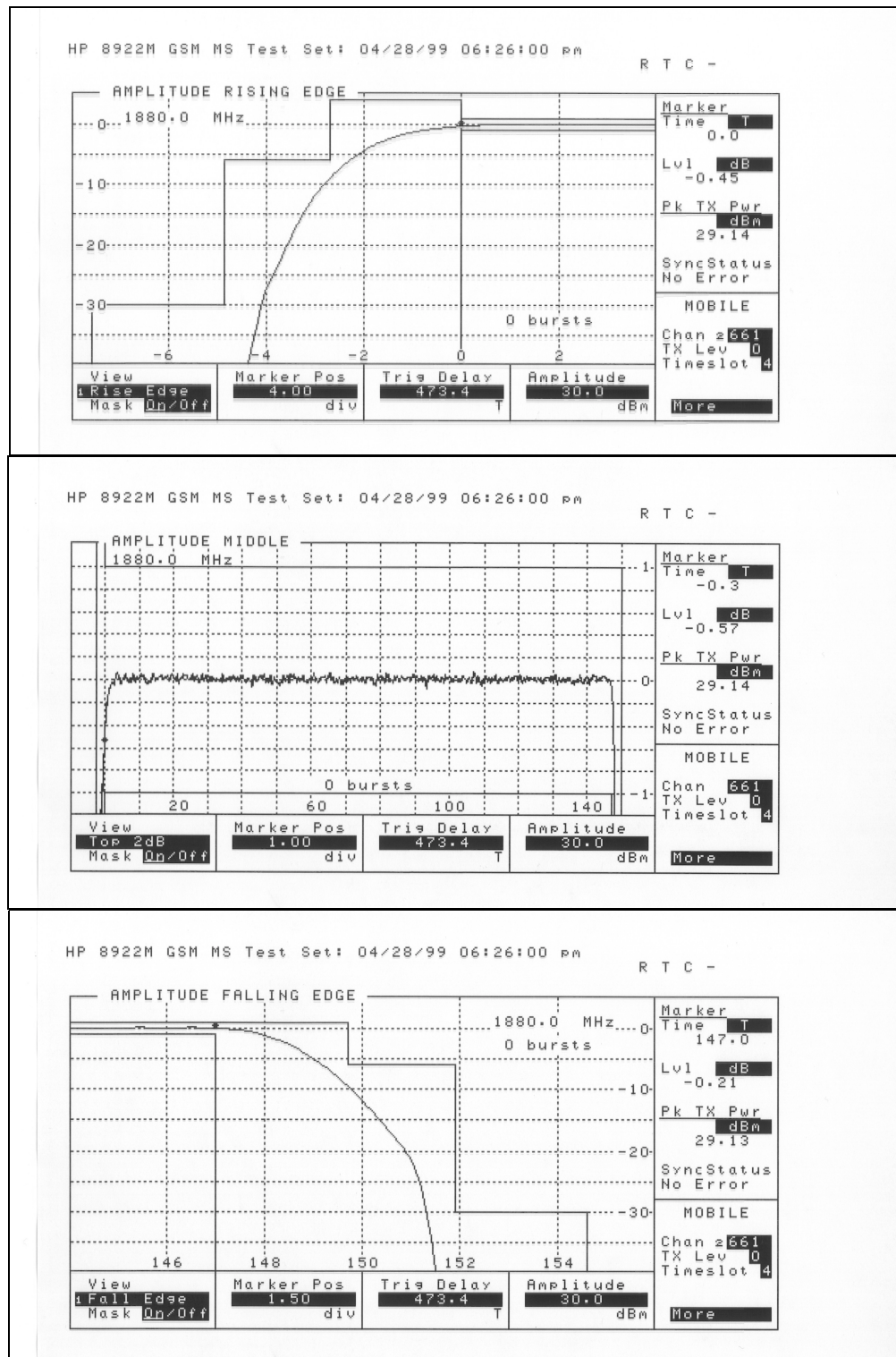
Figure 5.2.4 Carrier 1880.0 MHz (Ch 661) Power Level 0
