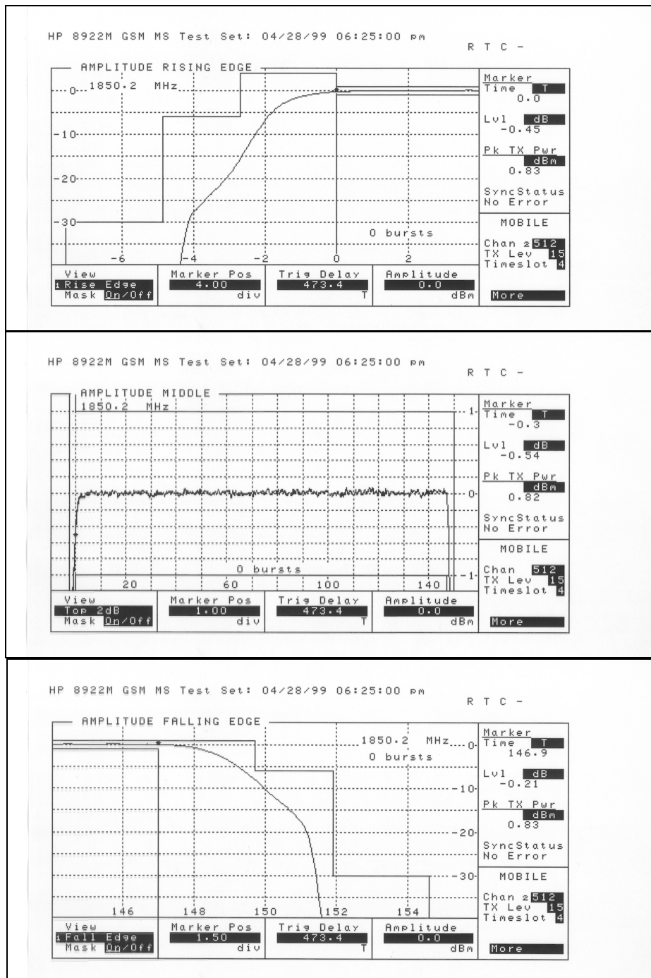
Figure 5.2.3 Carrier 1850.2 MHz (Ch 512) Power Level 15
