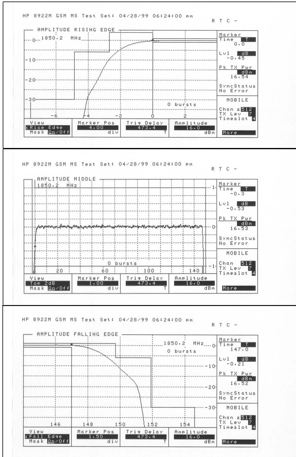
Figure 5.2.2 Carrier 1850.2 MHz (Ch 512) Power Level 7
