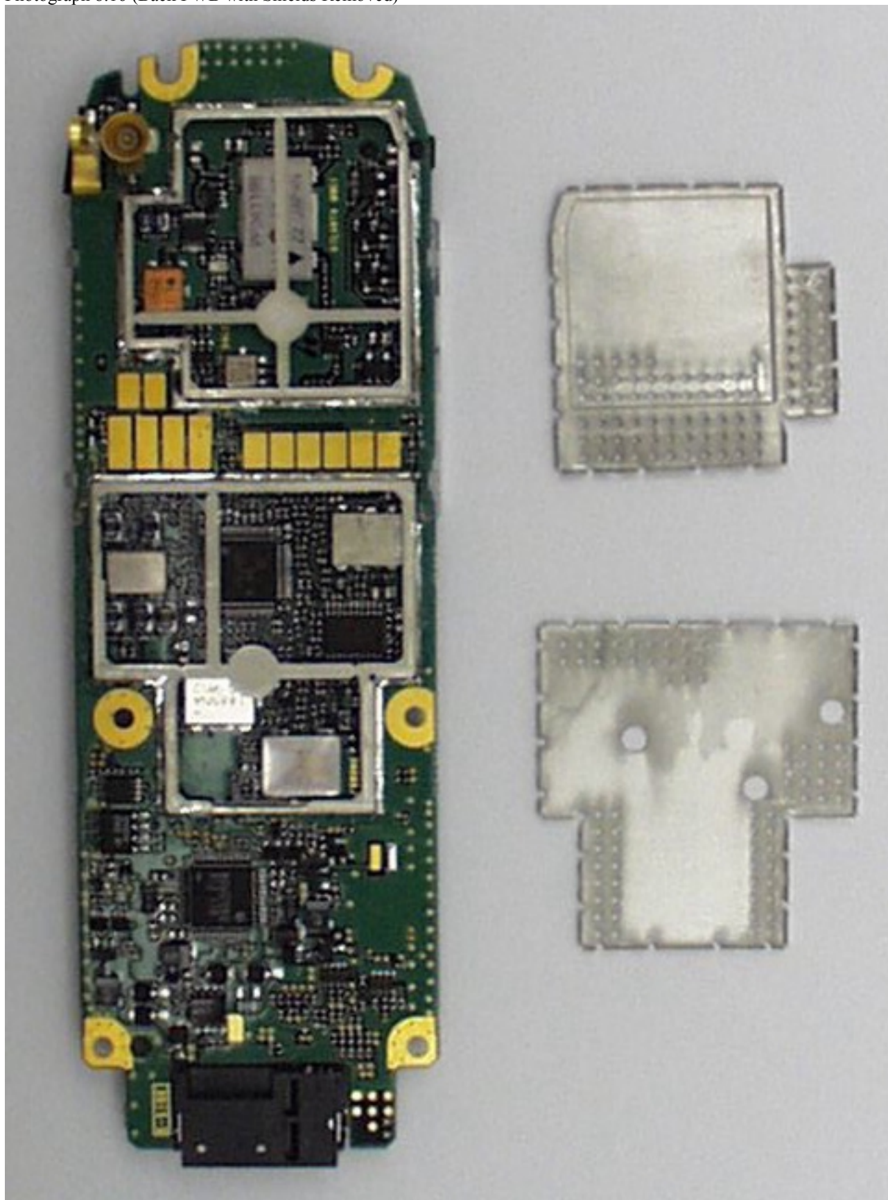
Photograph 8.16 (Back PWB with Shields Removed)
