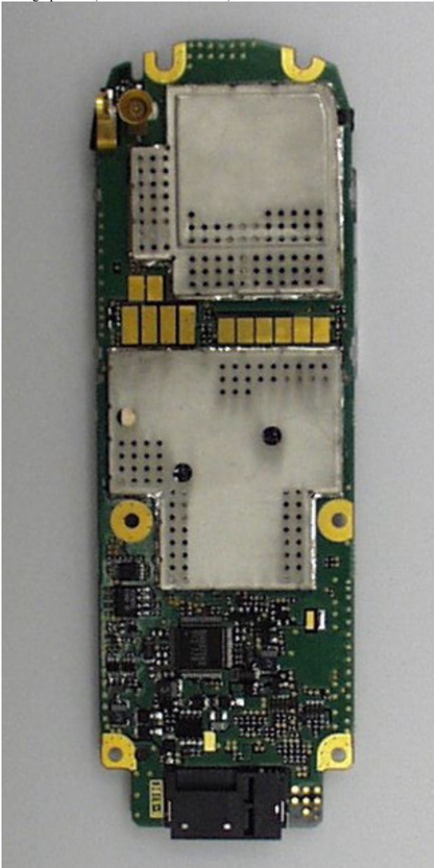
Photograph 8.15 (Back PWB with Shields)
