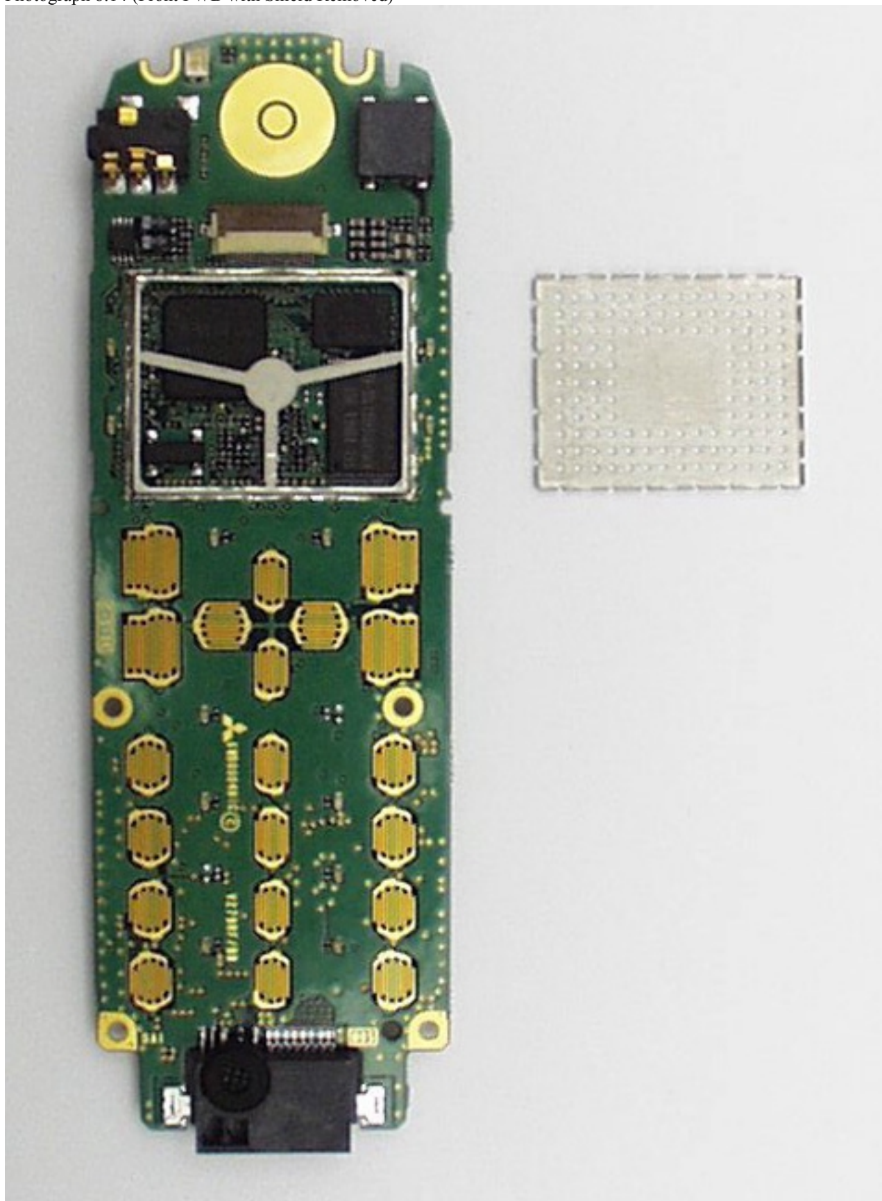
Photograph 8.14 (Front PWB with Shield Removed)
