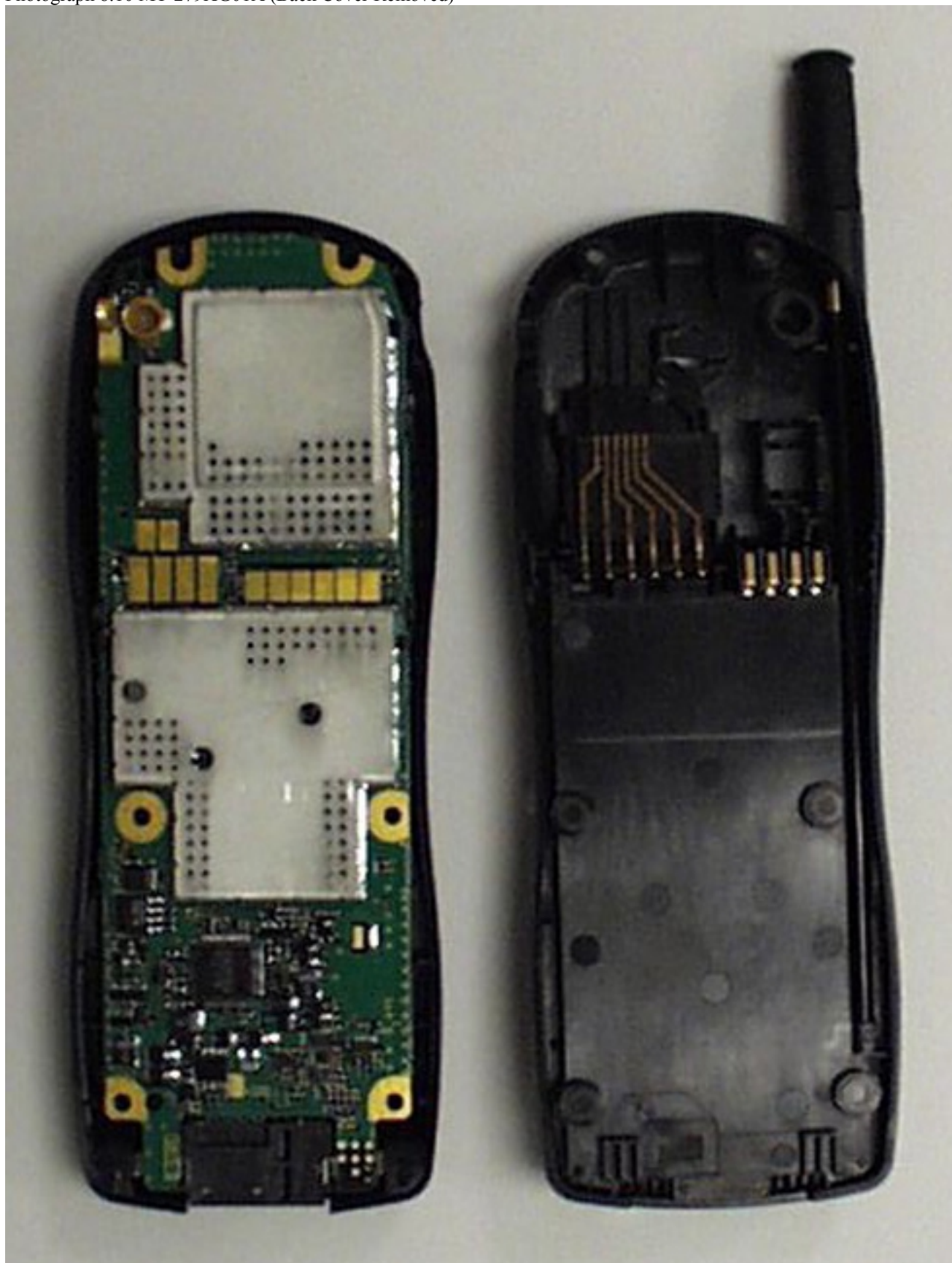
Photograph 8.10 MT-279XG01A (Back Cover Removed)
