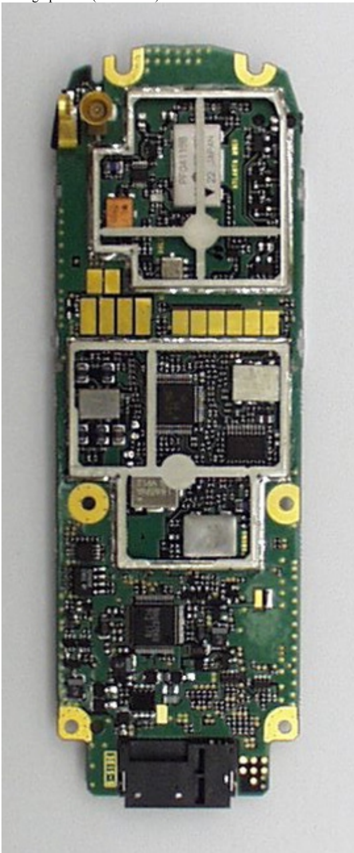
Photograph 8.18 (Back PWB)
