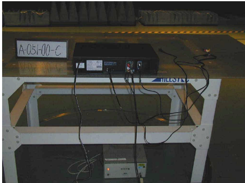
REAR VIEW
