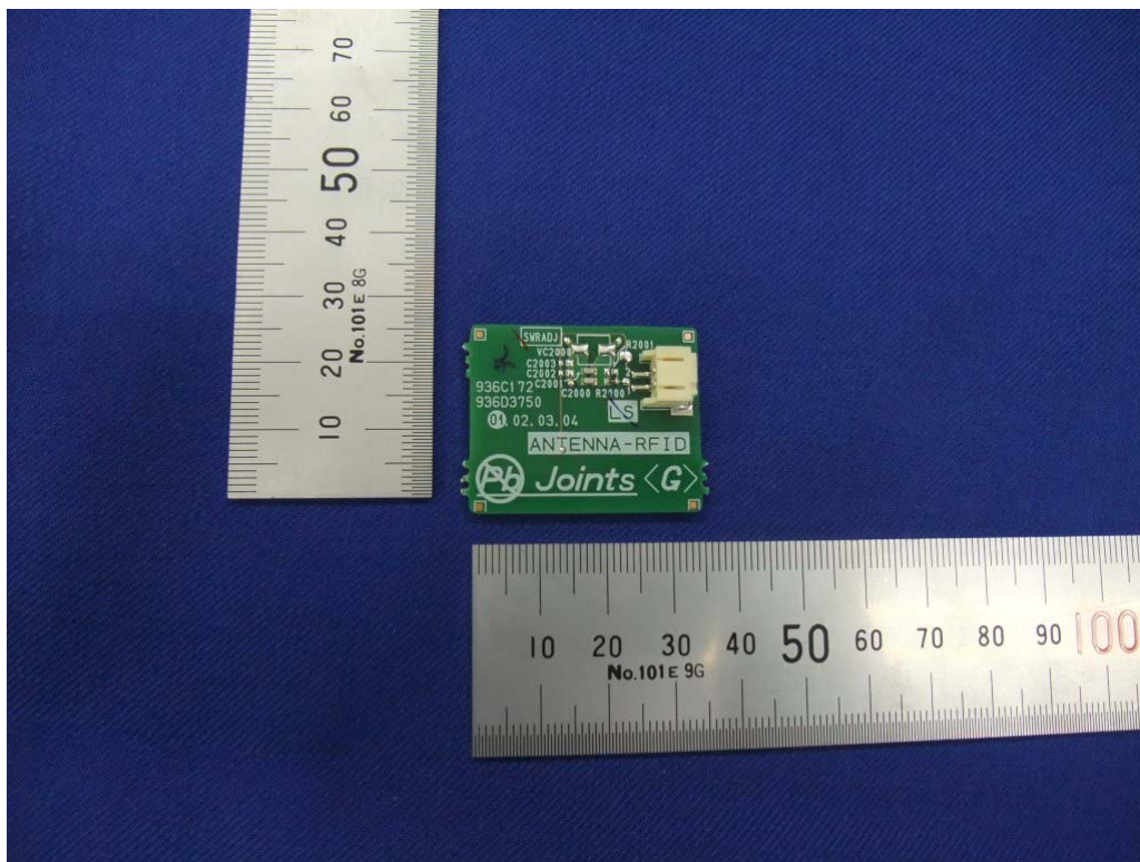
Antenna Board (Top)
