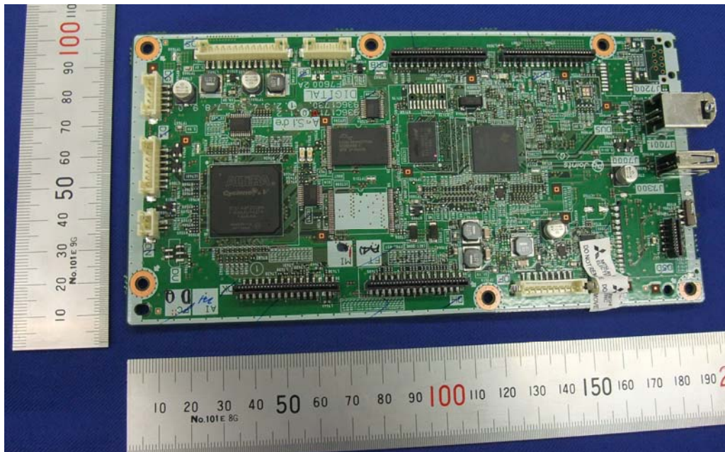
Digital Board (Top)
