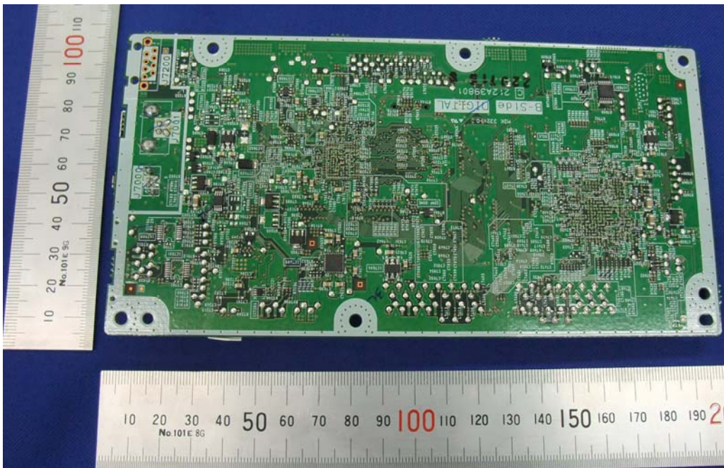
Digital Board (Bottom)
