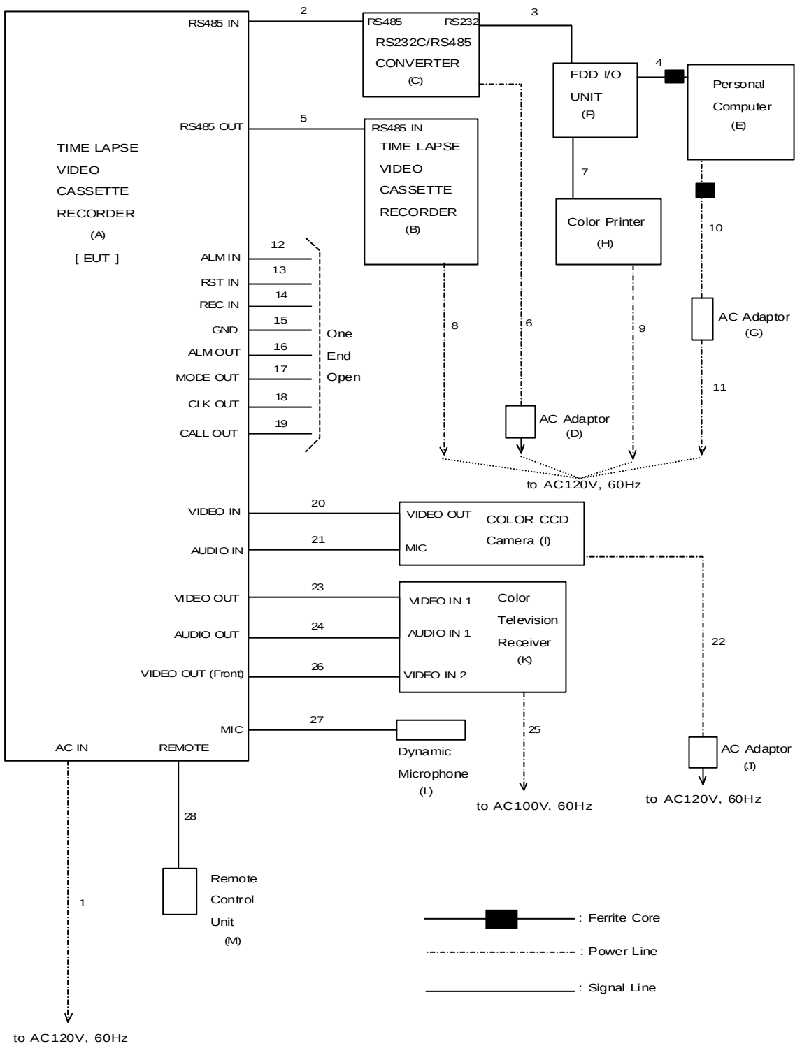
Block Diagram of EUT System
