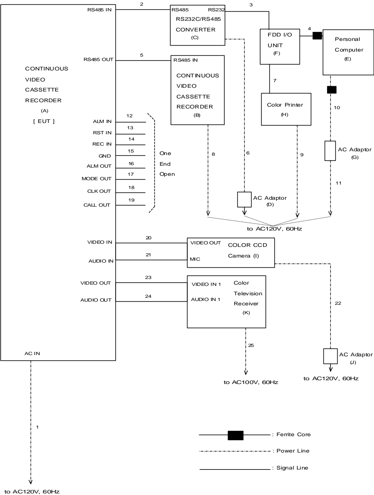
Block Diagram of EUT System
