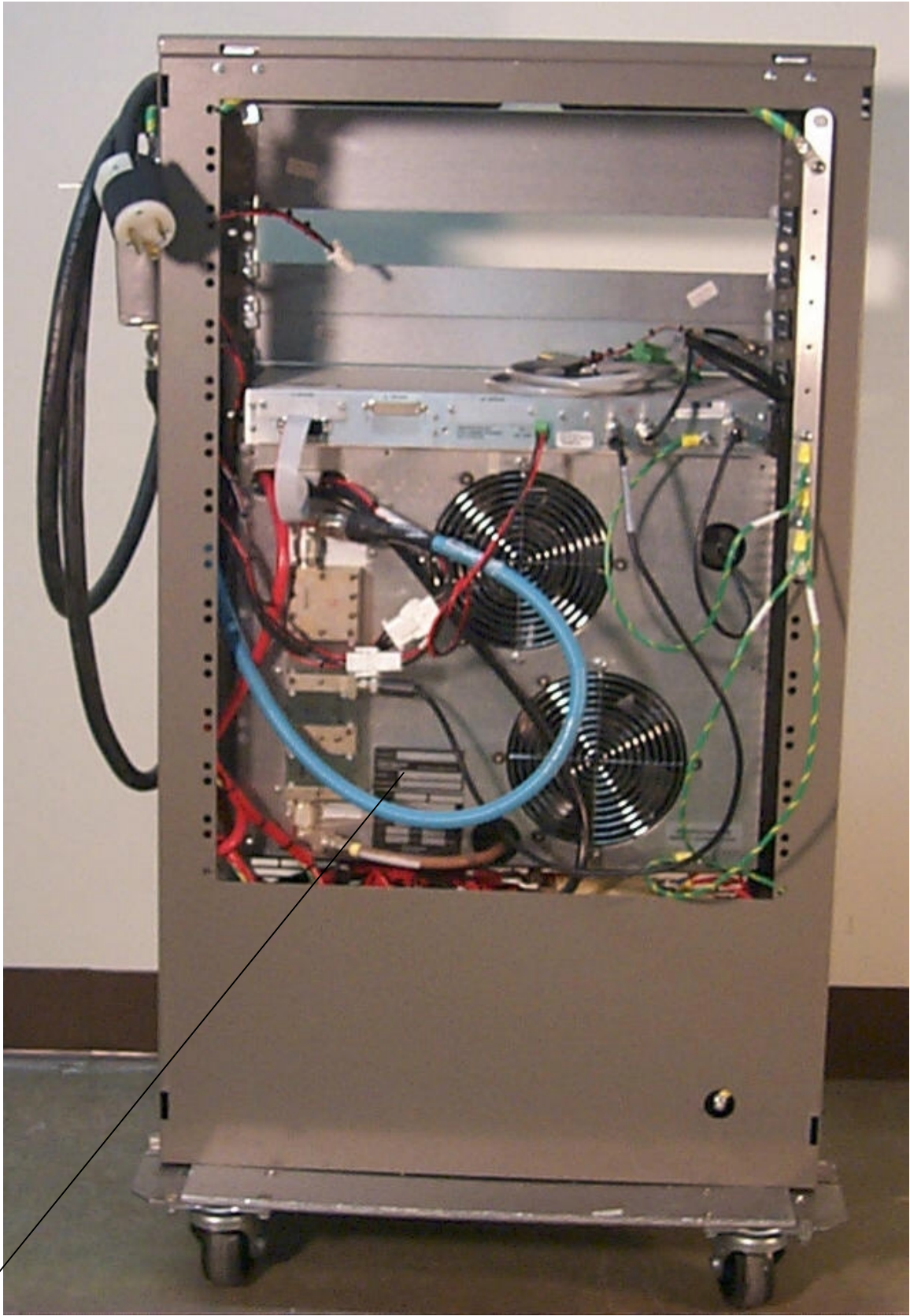
Backside view without cover, transmitter Model: GL-T8600-CN
