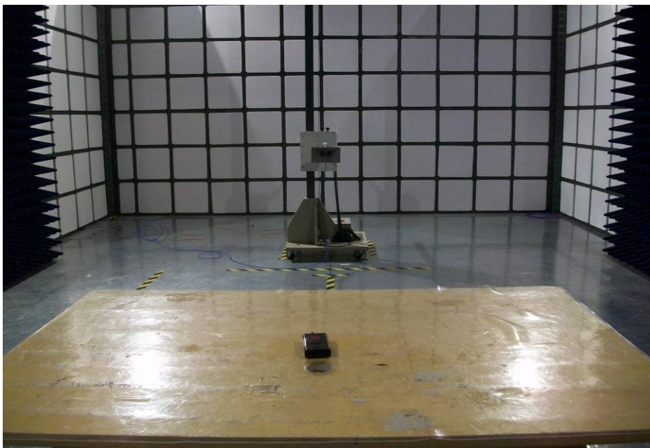
Radiation Emission Test View For 1GHz-10GHz
