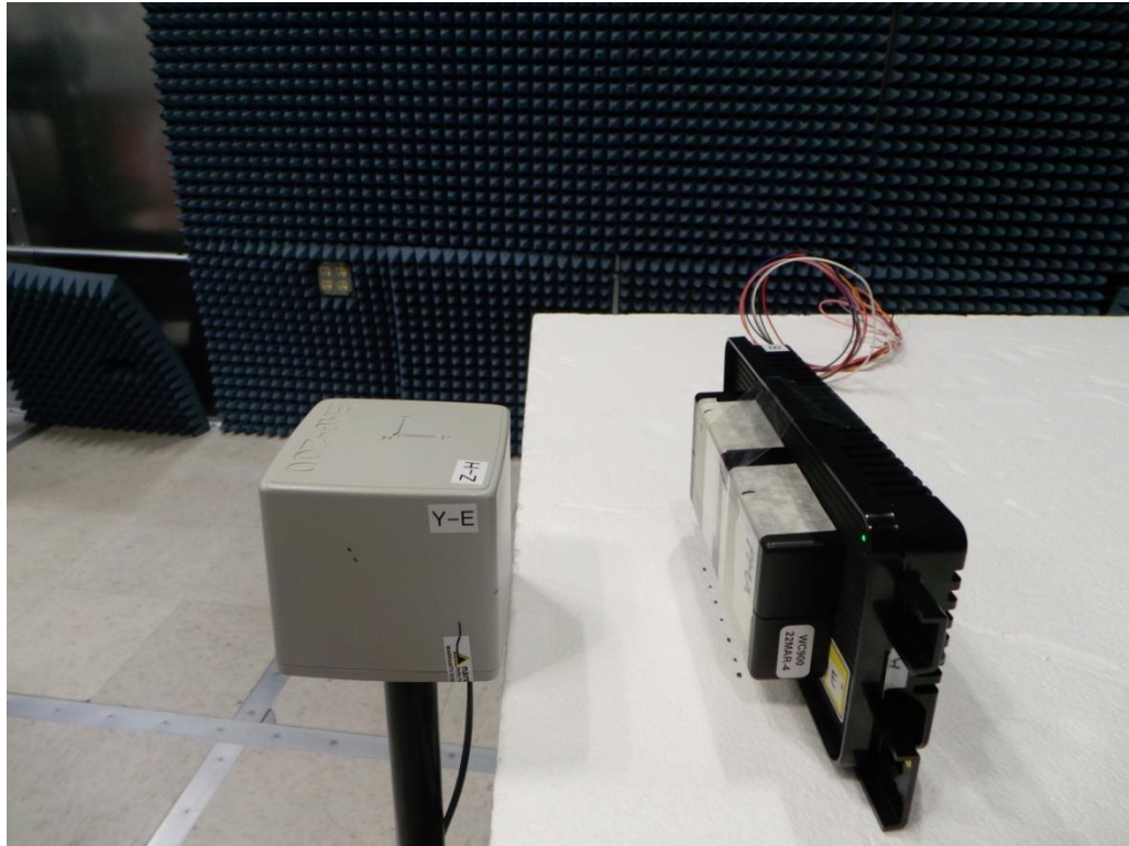
Figure 5. E-Field Measurement (Position E)
