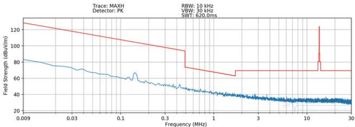
Plot 7-2. Radiated Spurious Plot from 9kHz - 30MHz (Pol. Y)
