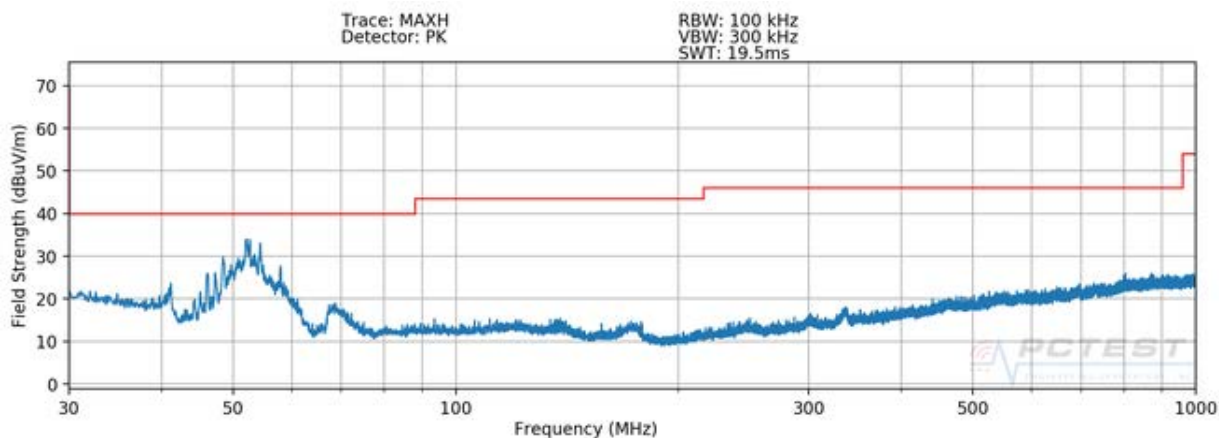
Plot 7-5. Radiated Spurious Plot above 30MHz (Pol. V)
