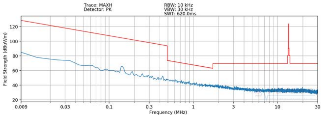
Plot 7-3. Radiated Spurious Plot from 9kHz – 30MHz (Pol. Z)
