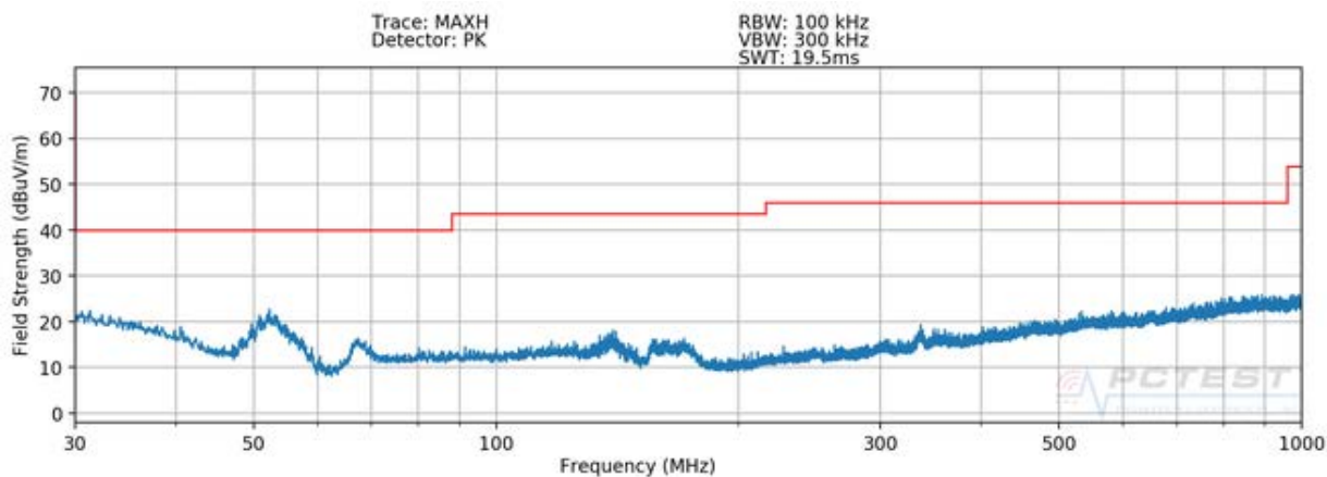
Plot 7-4. Radiated Spurious Plot above 30 MHz (Pol. H)
