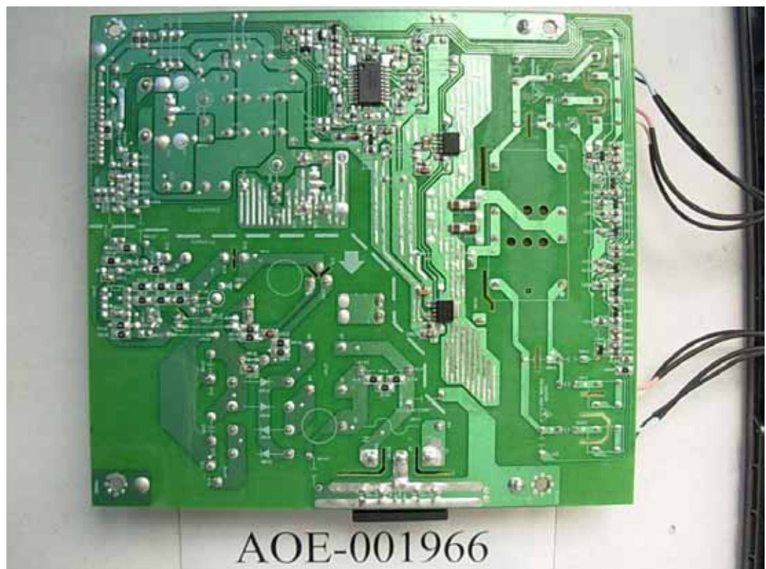
FIGURE 10 LCD MONITOR (M/N: W2261VT) POWER BOARD (SOLDERED SIDE)
