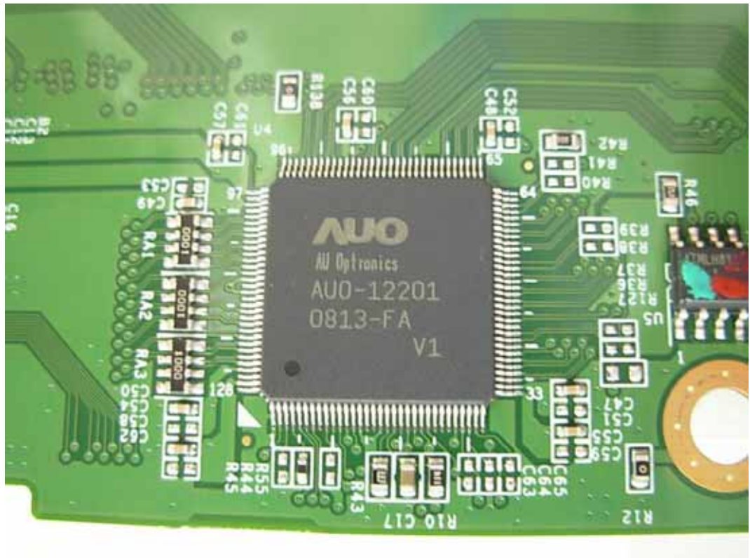
FIGURE 18 LCD MONITOR (M/N: W2261VT) CHIP ON LCD PANEL MAIN BOARD
