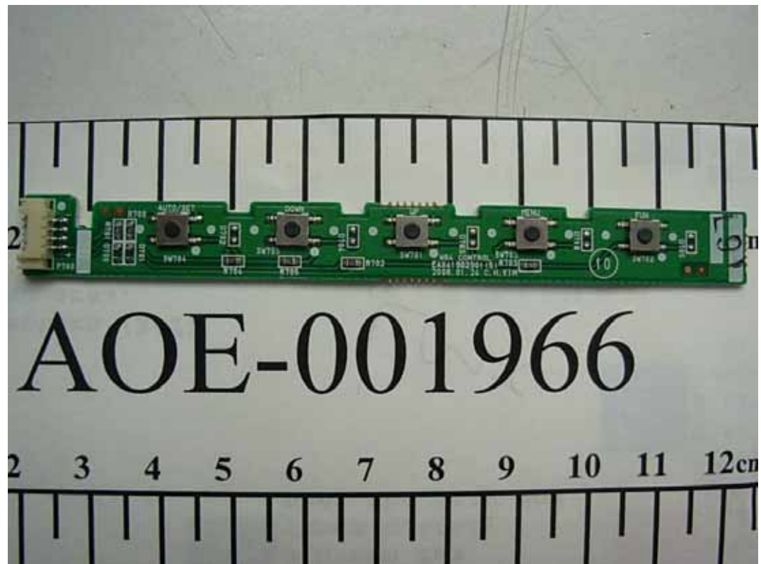
FIGURE 11 LCD MONITOR (M/N: W2261VT) KEY BOARD (COMPONENT SIDE)
