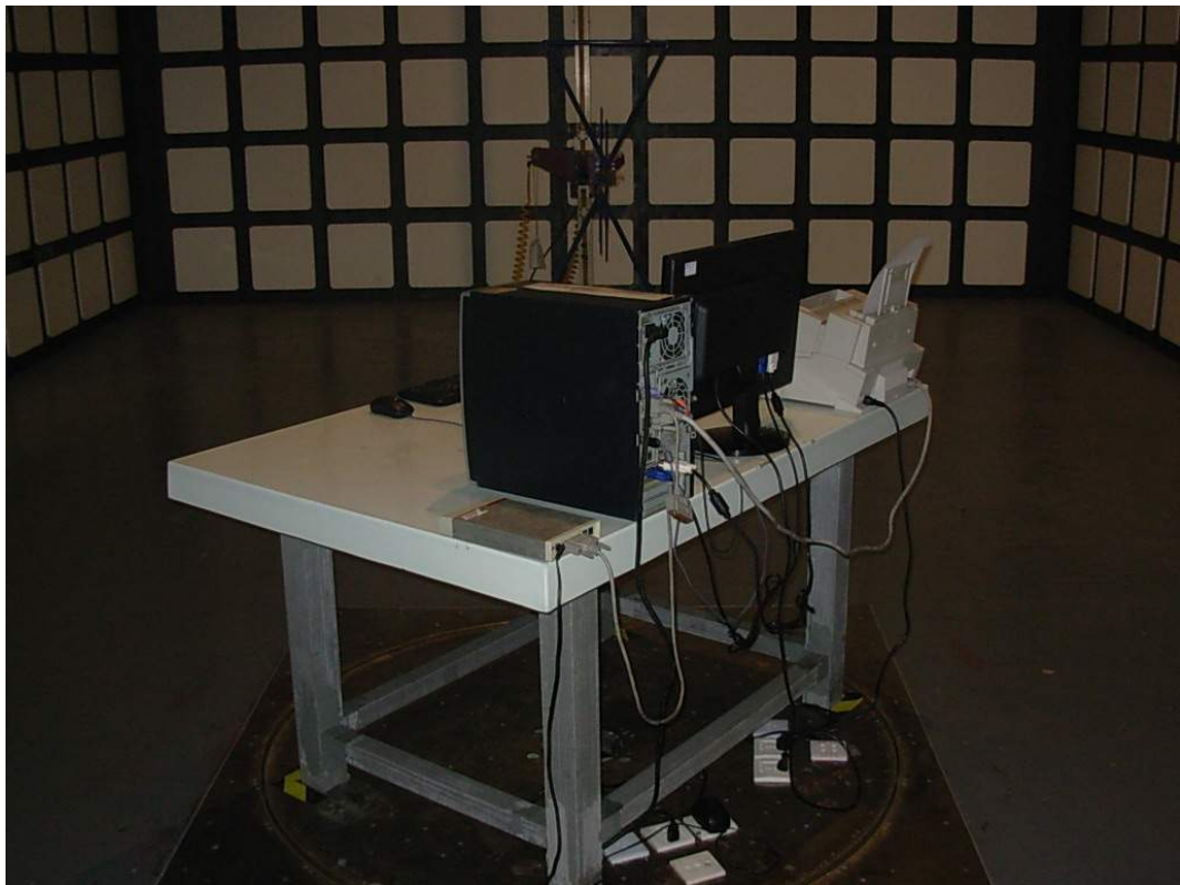
SETUP WITH MAXIMUM DETECTED EMISSION AT VERTICAL POLARIZATION (VGA 640*480@60Hz, Low FREQUENCY) (M/N: W2242TT)
