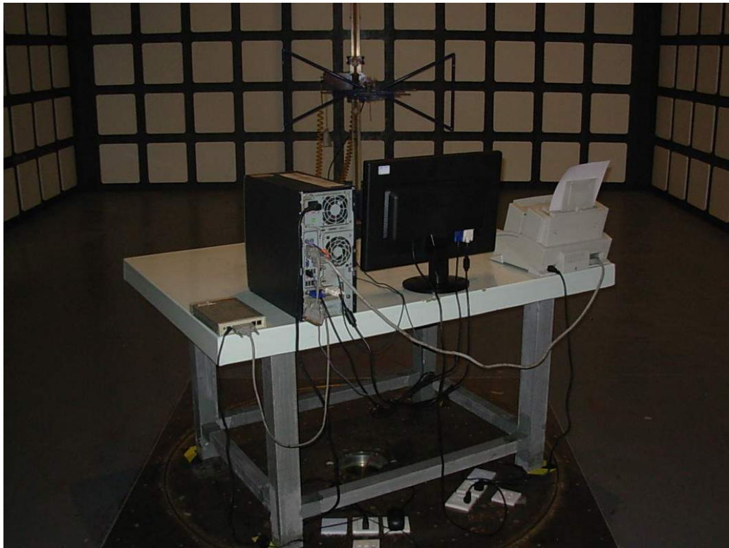
SETUP WITH MAXIMUM DETECTED EMISSION AT HORIZONTAL POLARIZATION (VGA 640*480@60Hz, Low FREQUENCY) (M/N: W2242TT)
