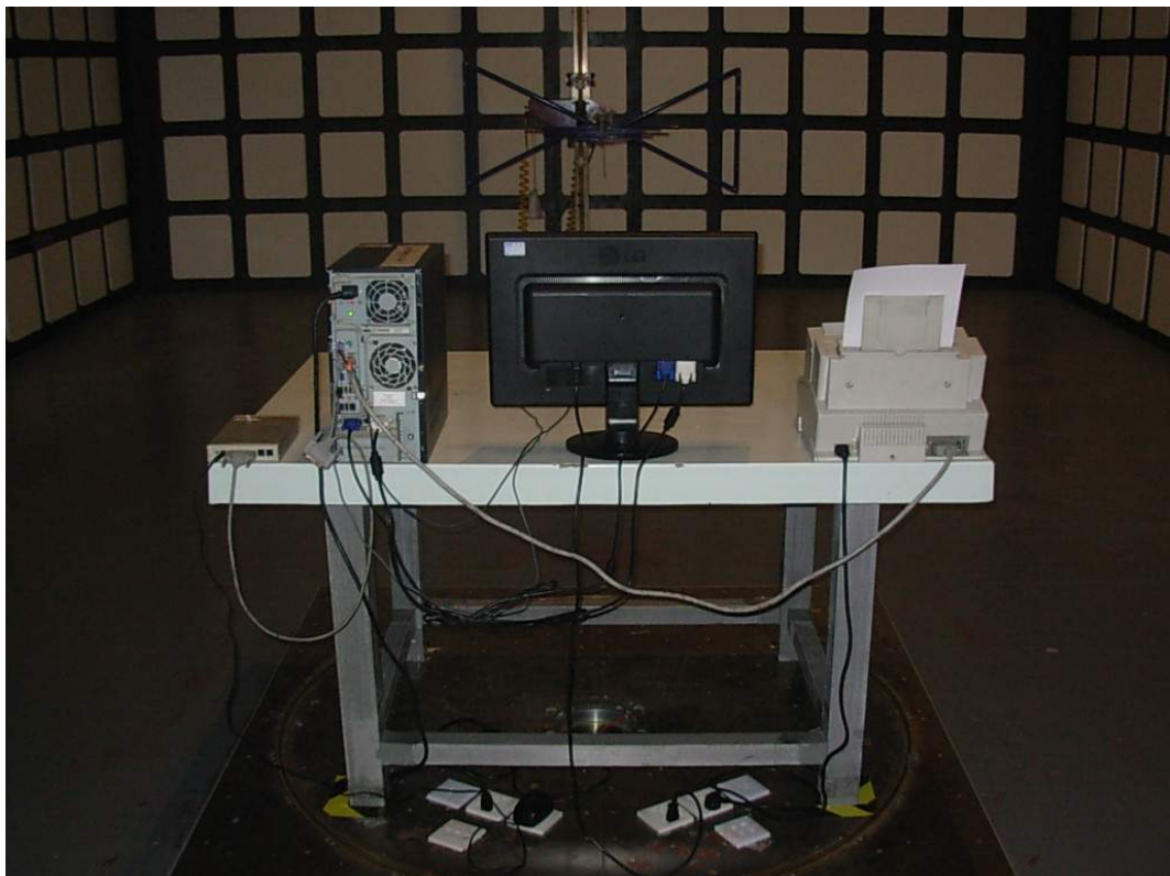
BACK VIEW OF RADIATED EMISSION TEST (LOW FREQUENCY)
