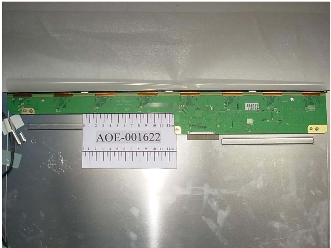
FIGURE 31 LCD MONITOR (M/N: W2242ST) LCD PANEL MAIN BOARD (FRONT VIEW)
