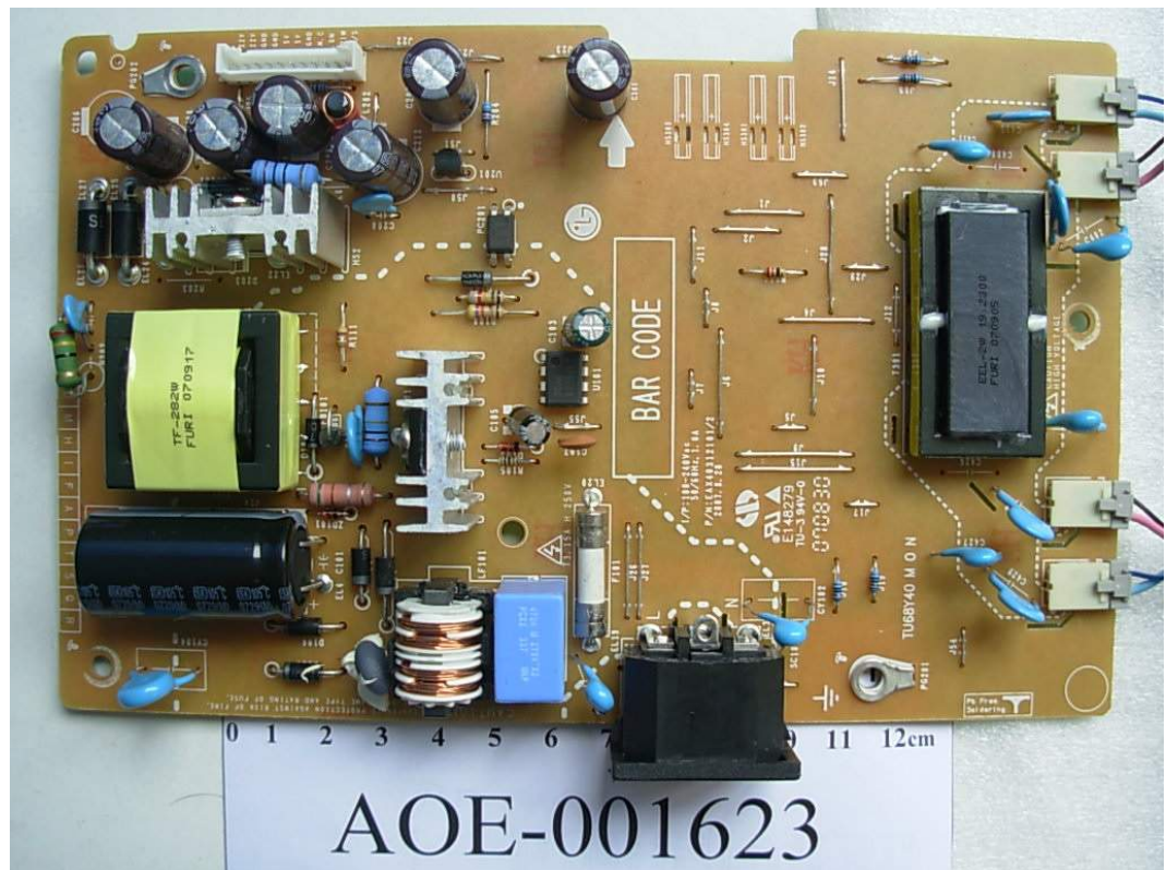
FIGURE 5 LCD MONITOR (M/N: W2242TT) POWER BOARD (COMPONENT SIDE)
