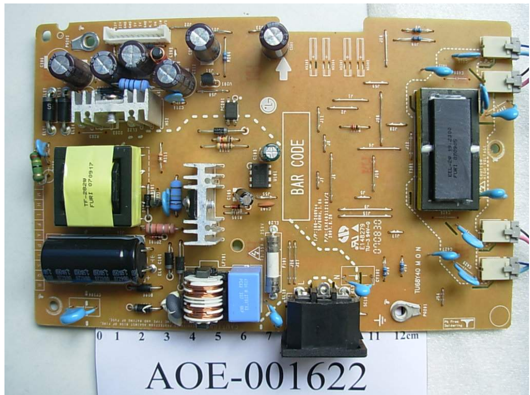
FIGURE 23 LCD MONITOR (M/N: W2242ST) POWER BOARD (COMPONENT SIDE)
