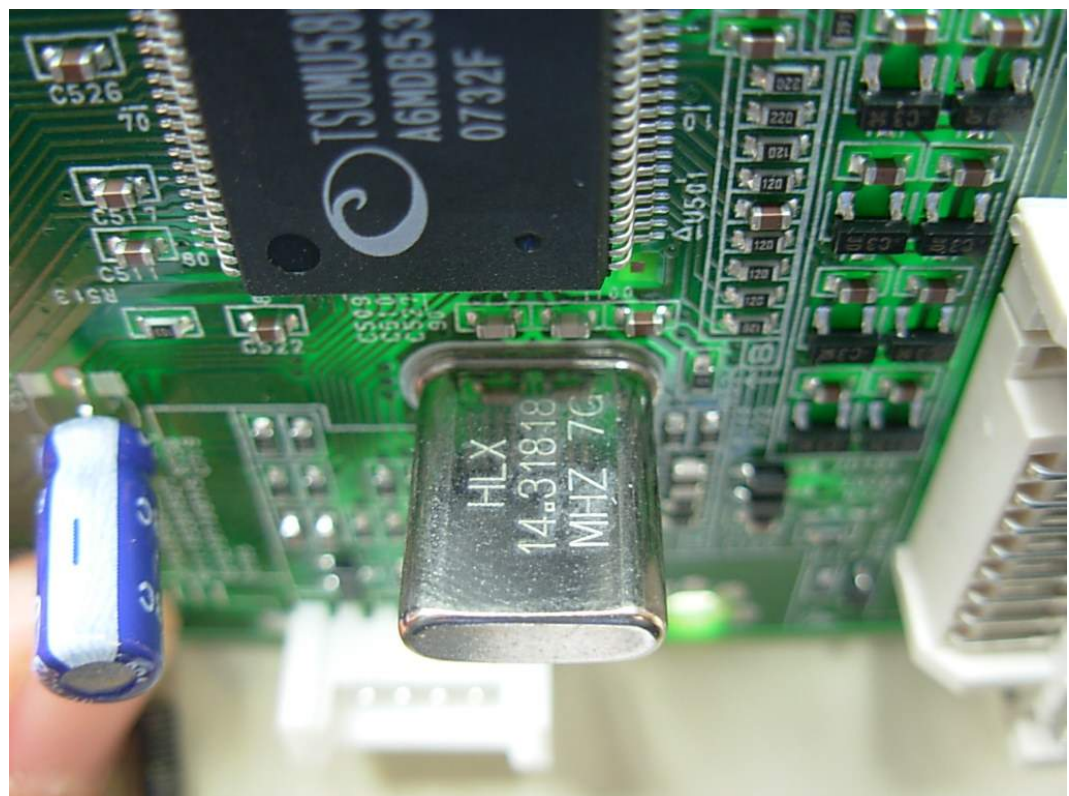
FIGURE 10 LCD MONITOR (M/N: W2242TT) CRYSTAL ON MAIN BOARD
