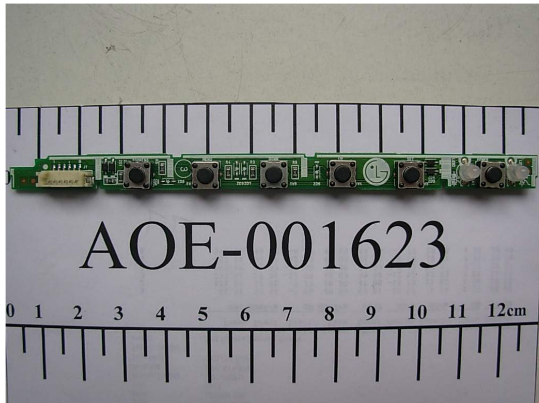
FIGURE 2 LCD MONITOR (M/N: W2242TT) BUTTON BOARD (FRONT VIEW)
