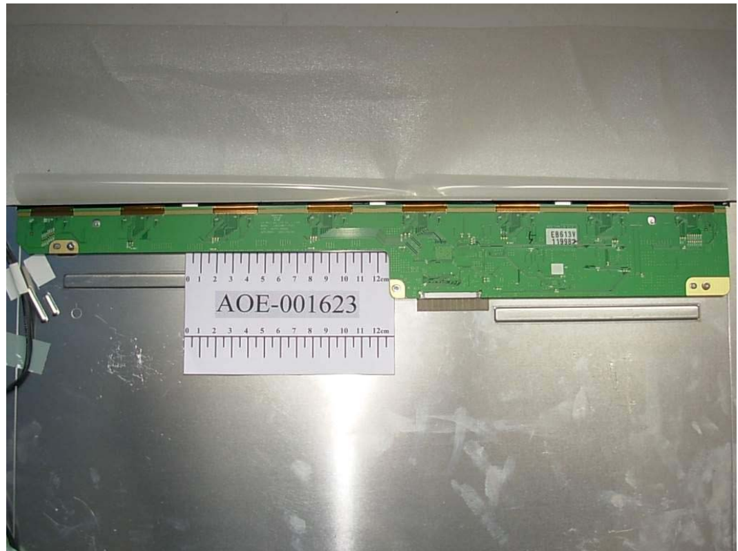
FIGURE 13 LCD MONITOR (M/N: W2242TT) LCD PANEL MAIN BOARD (FRONT VIEW)
