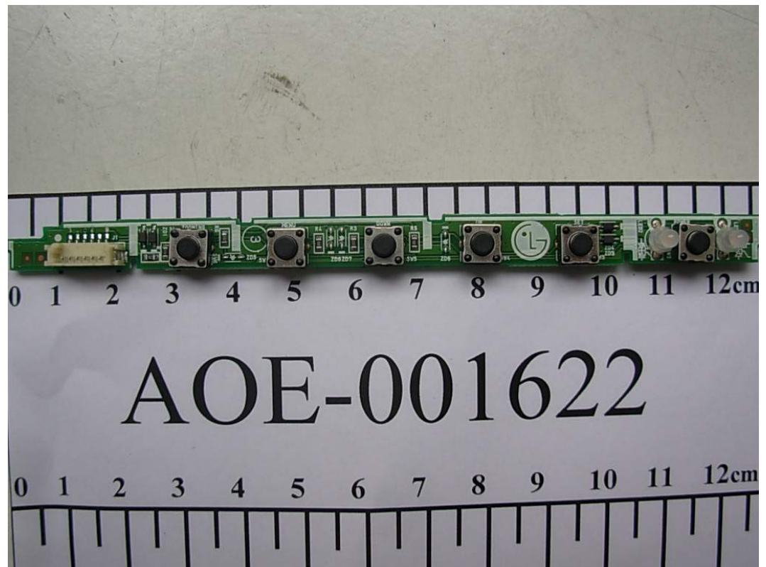
FIGURE 20 LCD MONITOR (M/N: W2242ST) BUTTON BOARD (FRONT VIEW)
