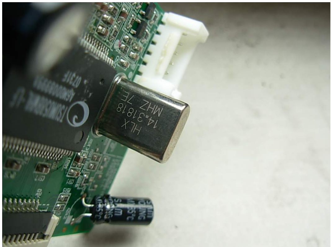
FIGURE 28 LCD MONITOR (M/N: W2242ST) CRYSTAL ON MAIN BOARD
