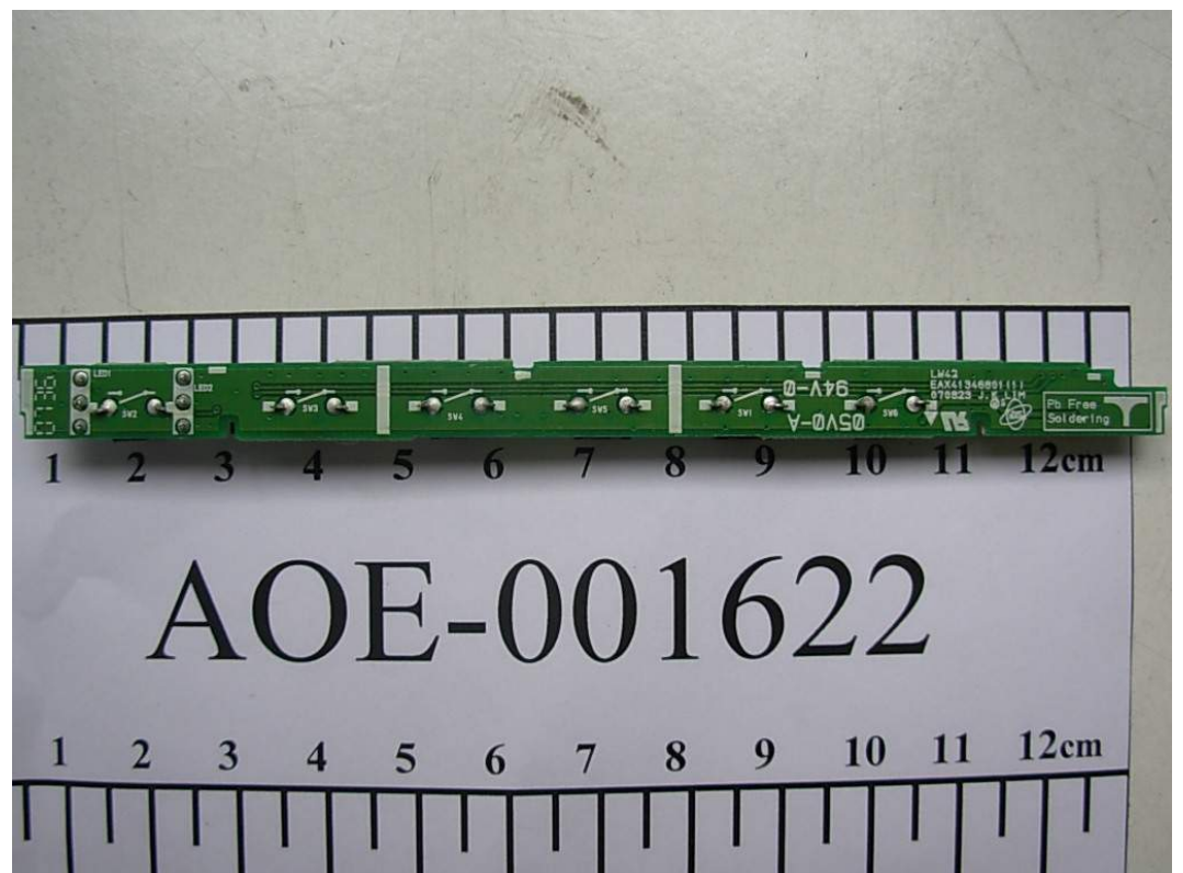
FIGURE 21 LCD MONITOR (M/N: W2242ST) BUTTON BOARD (BACK VIEW)
