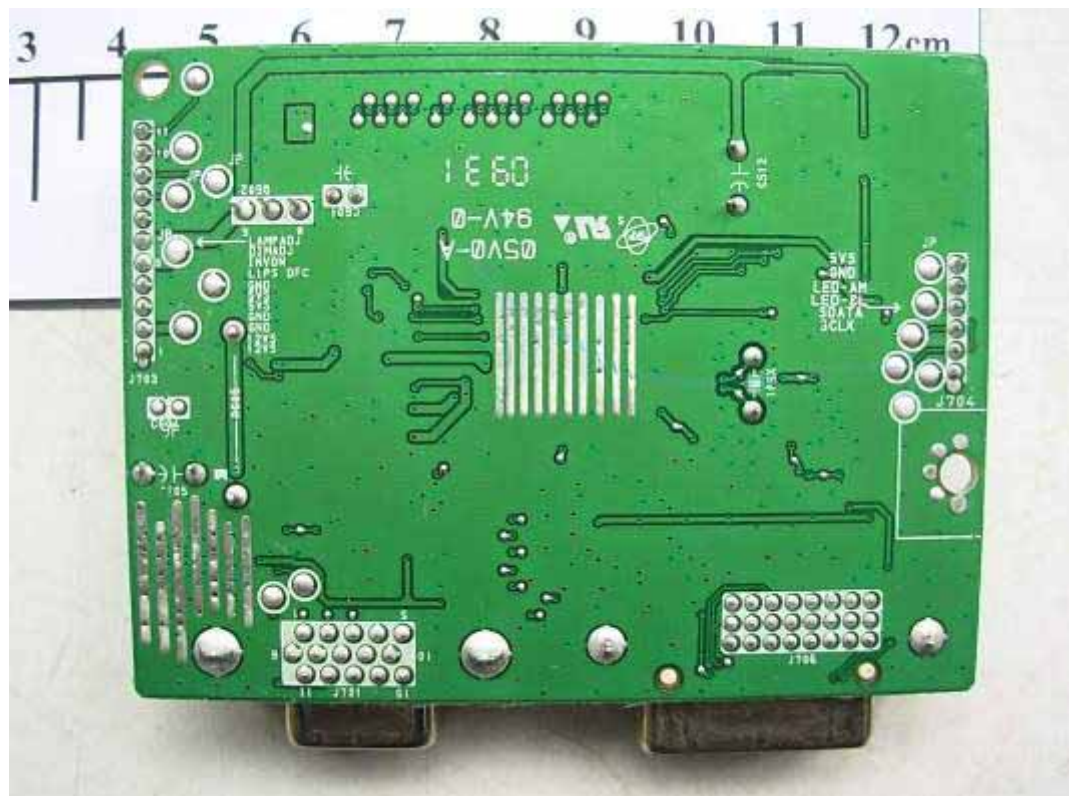
FIGURE 6 LCD MONITOR (M/N: W2040TV) MAIN BOARD (SOLDERED SIDE)
