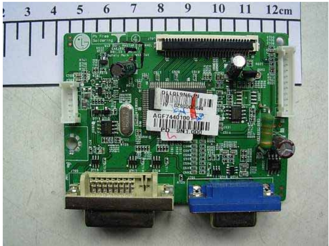
FIGURE 5 LCD MONITOR (M/N: W2040TV) MAIN BOARD (COMPONENT SIDE)
