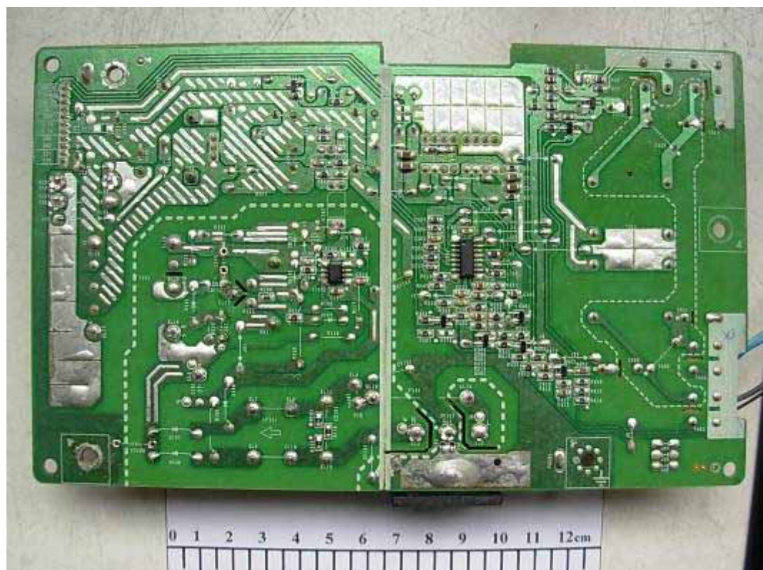
FIGURE 9 LCD MONITOR (M/N: W2040TV) POWER BOARD (SOLDERED SIDE)
