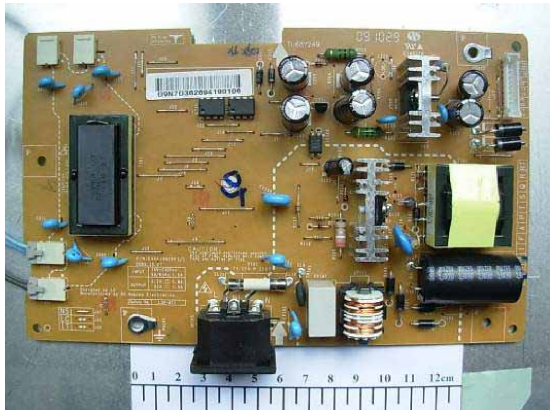
FIGURE 8 LCD MONITOR (M/N: W2040TV) POWER BOARD (COMPONENT SIDE)
