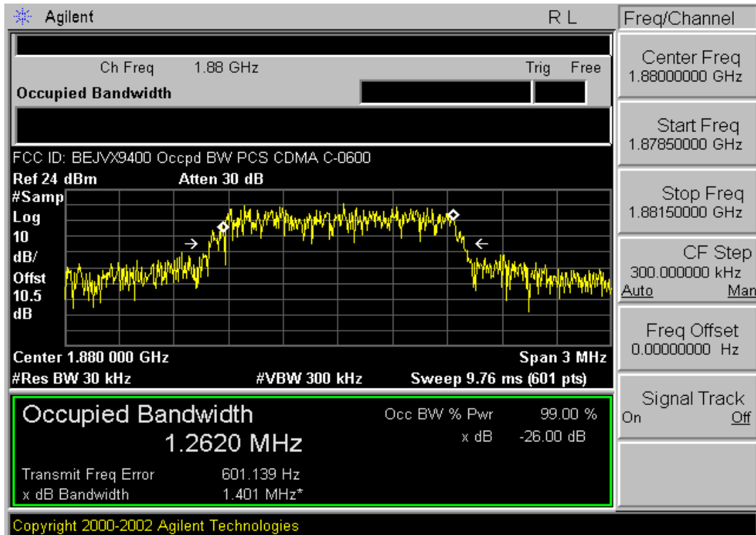
Plot A-19. Occupied Bandwidth (PCS CDMA Mode – Ch. 600)
