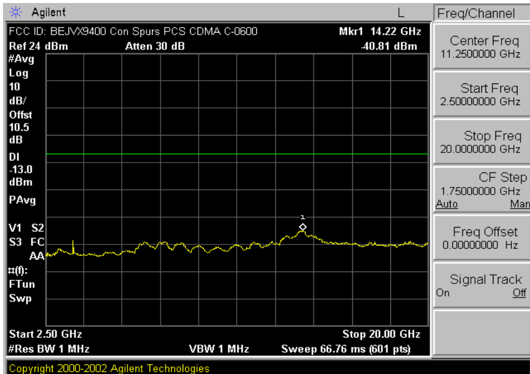
Plot A-18. Conducted Spurious (PCS CDMA Mode – Ch. 600)
