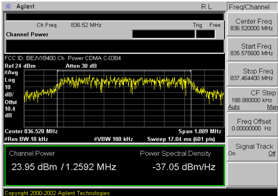
Plot A-8. Channel Power (Cellular CDMA Mode – Ch. 384)
