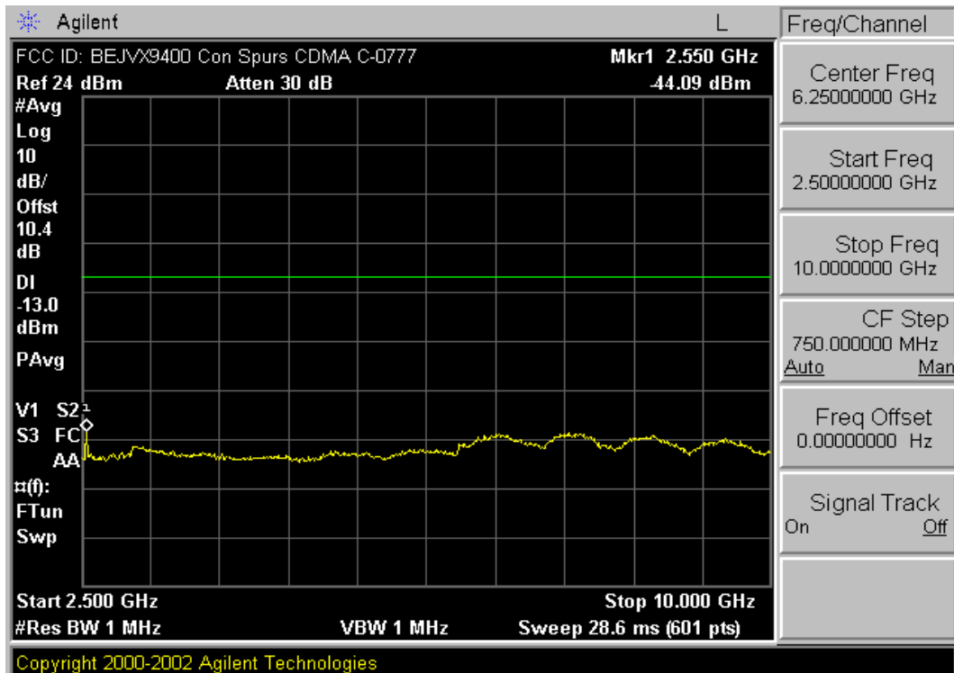
Plot A-10. Conducted Spurious (Cellular CDMA Mode – Ch. 777)
