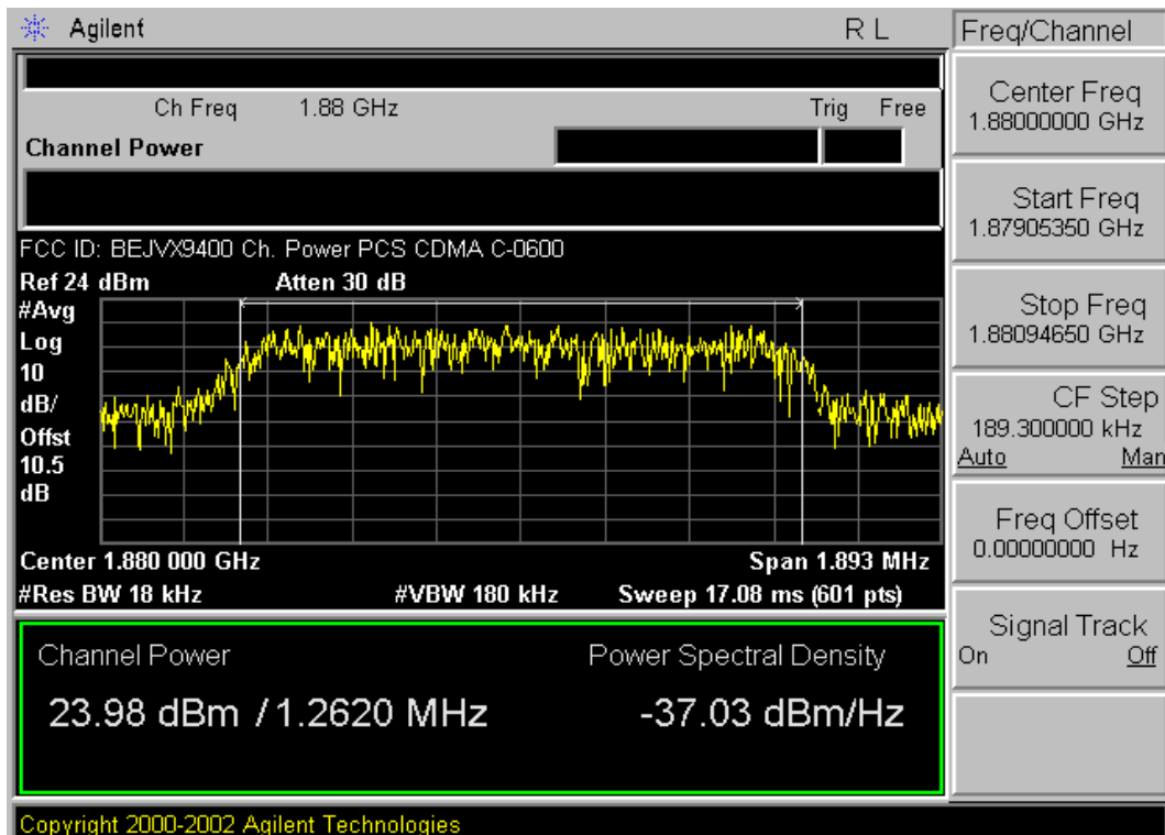
Plot A-20. Channel Power (PCS CDMA Mode – Ch. 600)
