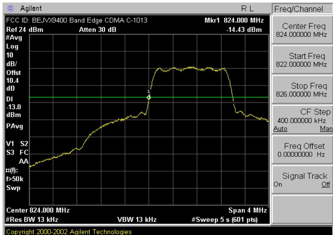
Plot A-3. Band Edge (Cellular CDMA Mode – Ch. 1013)
