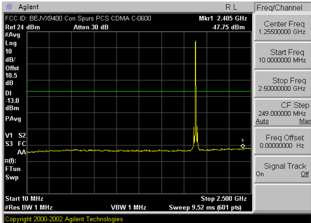
Plot A-17. Conducted Spurious (PCS CDMA Mode – Ch. 600)
