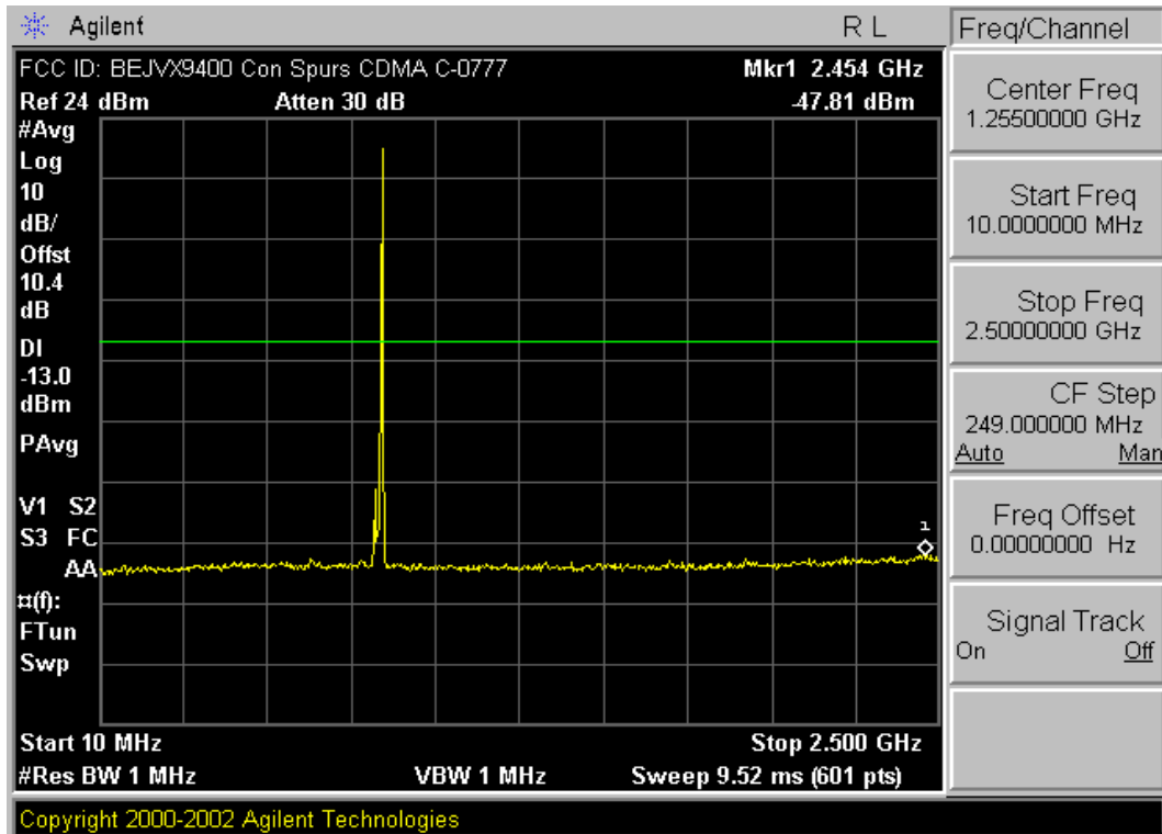
Plot A-9. Conducted Spurious (Cellular CDMA Mode – Ch. 777)
