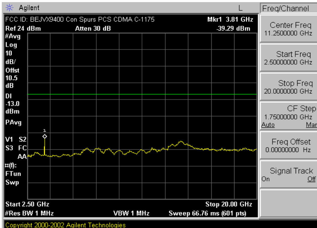
Plot A-22. Conducted Spurious (PCS CDMA Mode – Ch. 1175)
