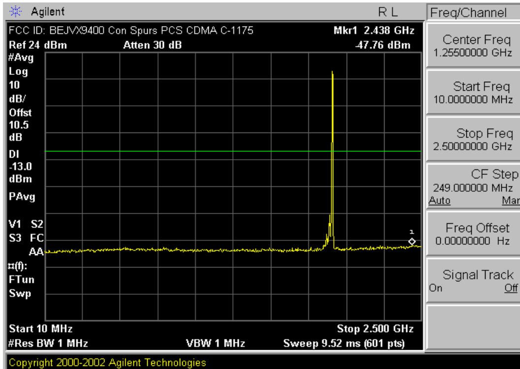
Plot A-21. Conducted Spurious (PCS CDMA Mode – Ch. 1175)
