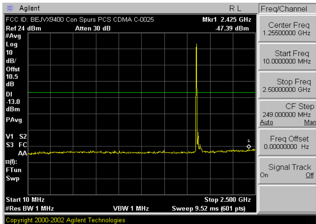
Plot A-13. Conducted Spurious (PCS CDMA Mode – Ch. 25)
