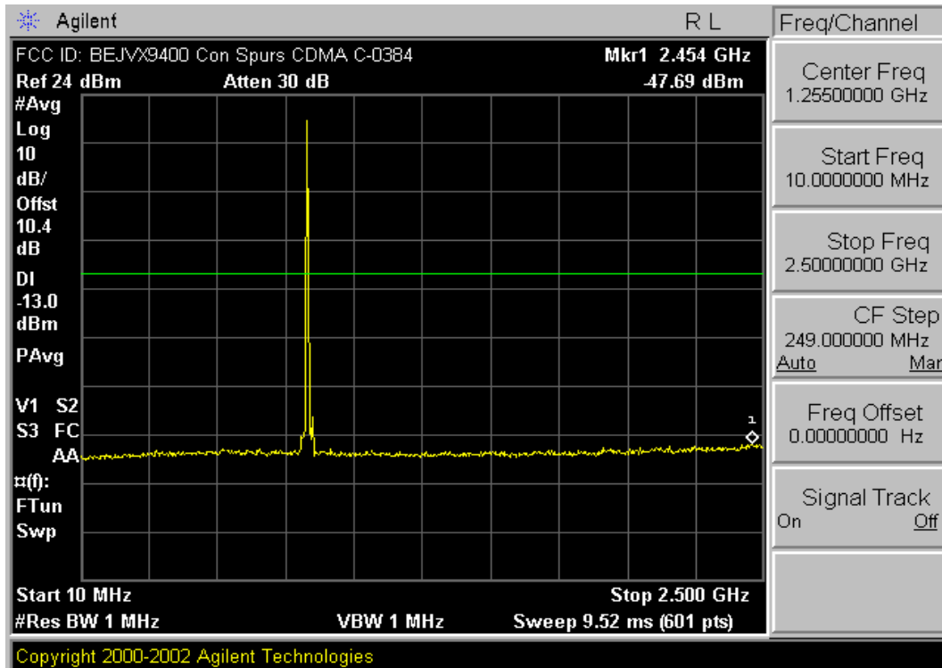
Plot A-5. Conducted Spurious (Cellular CDMA Mode – Ch. 384)
