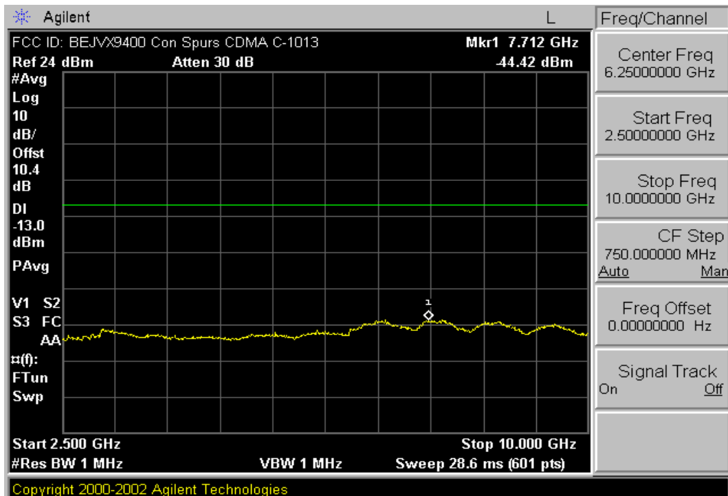
Plot A-2. Conducted Spurious (Cellular CDMA Mode – Ch. 1013)
