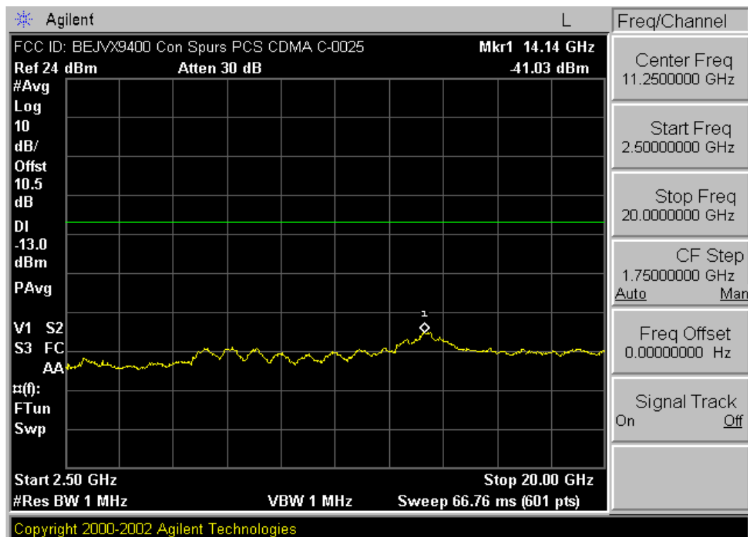
Plot A-14. Conducted Spurious (PCS CDMA Mode – Ch. 25)
