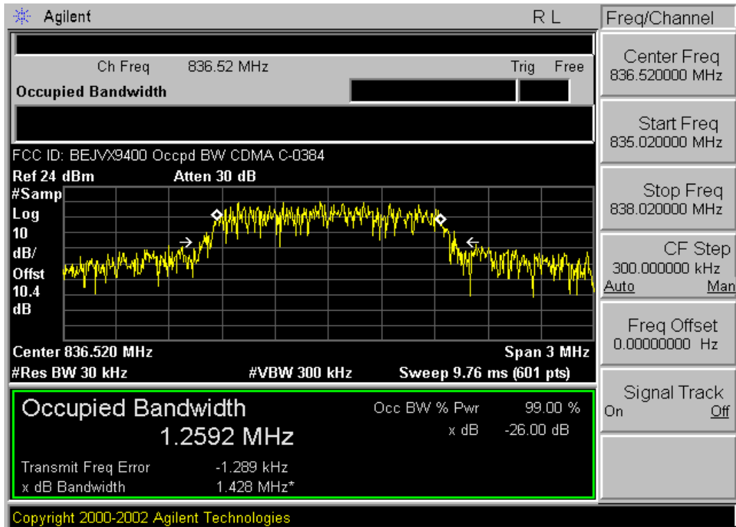
Plot A-7. Occupied Bandwidth (Cellular CDMA Mode – Ch. 384)
