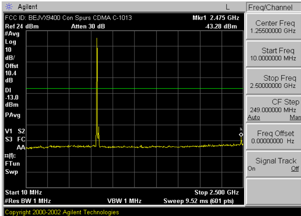
Plot A-1. Conducted Spurious (Cellular CDMA Mode – Ch. 1013)
