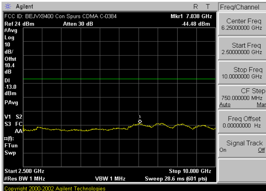
Plot A-6. Conducted Spurious (Cellular CDMA Mode – Ch. 384)
