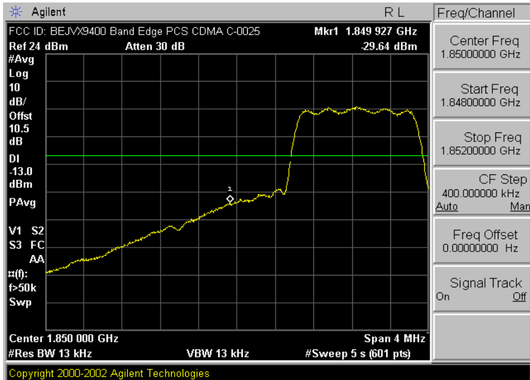
Plot A-15. Band Edge (PCS CDMA Mode – Ch. 25)
