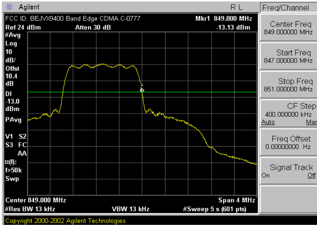
Plot A-11. Band Edge (Cellular CDMA Mode – Ch. 777)
