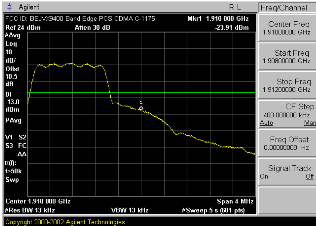
Plot A-23. Band Edge (PCS CDMA Mode – Ch. 1175)
