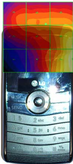
Figure 17-4 E-Field WD Scan overlay
