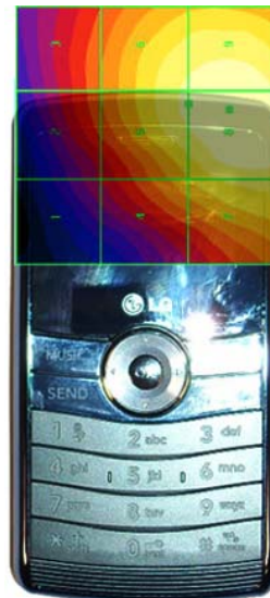
Figure 17-5 H-Field WD Scan overlay
