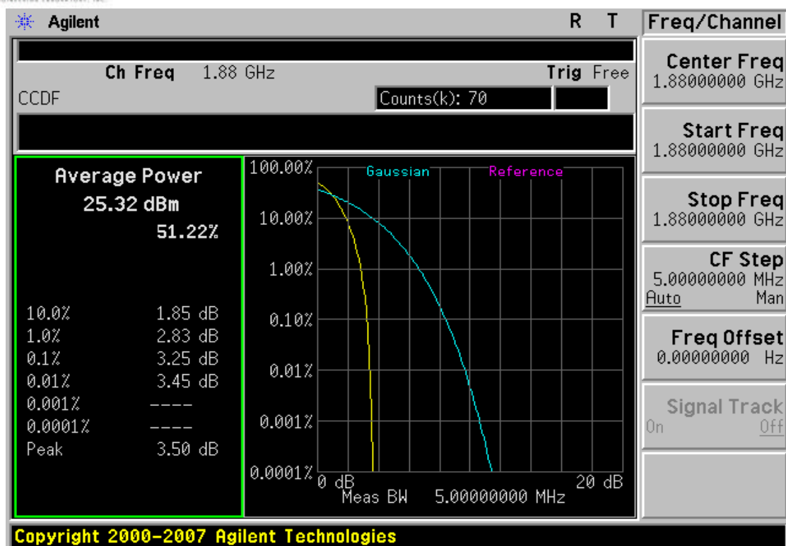
Plot 7-19. Peak-Average Ratio Plot (PCS CDMA Mode – Ch. 600)
