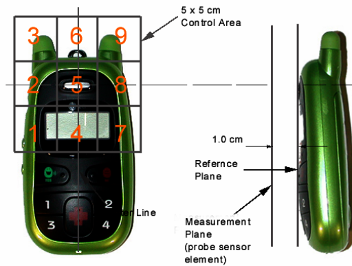
Figure 13 E/H-Field Emissions Test Setup Diagram
