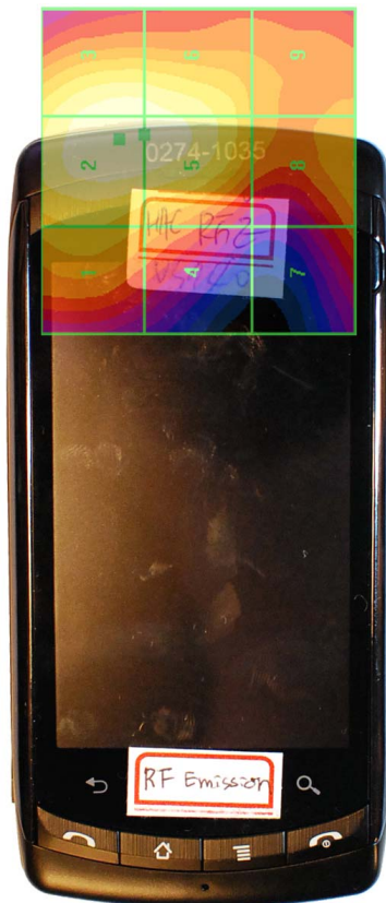
Figure 17-4 E-Field WD Scan overlay
