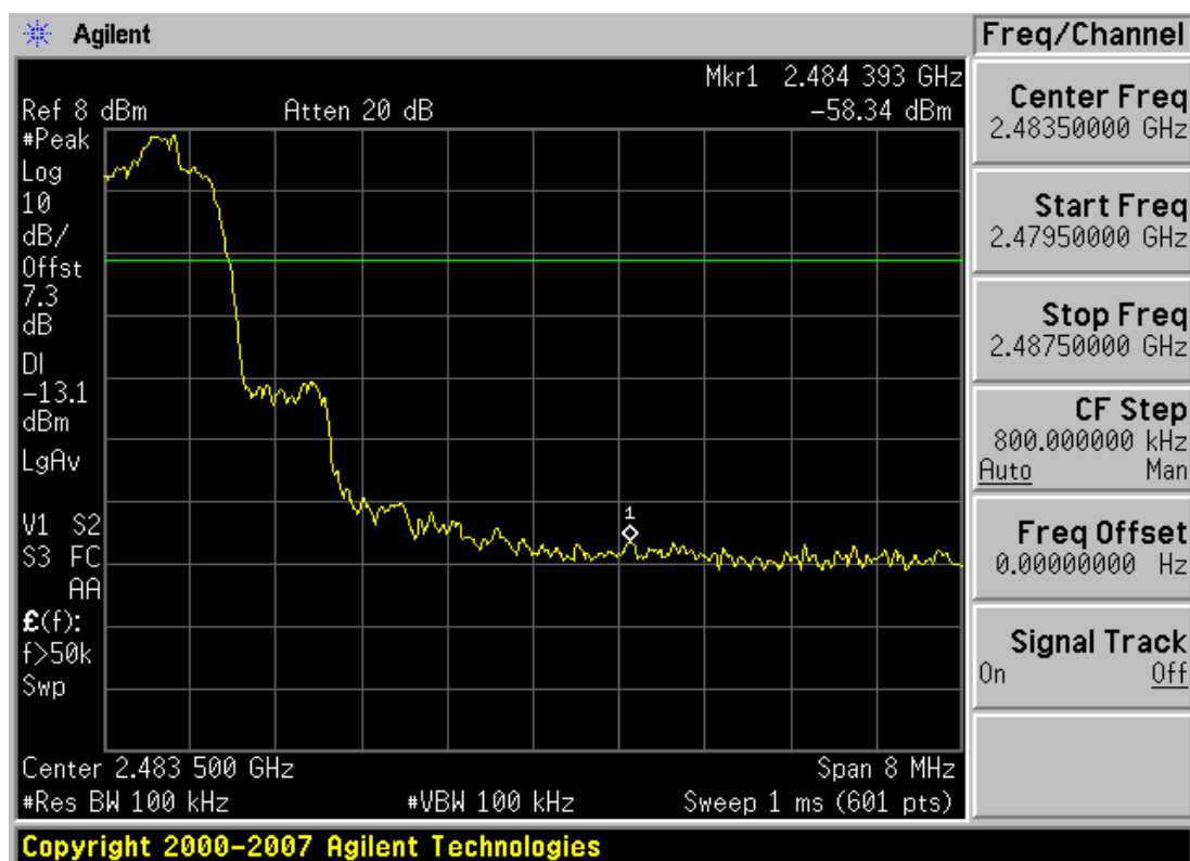
Plot 6-7. Band Edge Plot (Bluetooth 2.0 with Enhanced Data Rates – Ch. 78)
