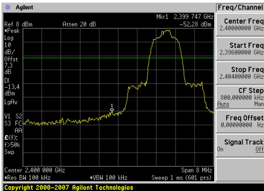
Plot 6-6. Band Edge Plot (Bluetooth 2.0 with Enhanced Data Rates – Ch. 0)
