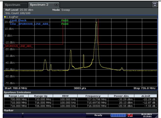
QPSK High Channel - 1 RB - Right
