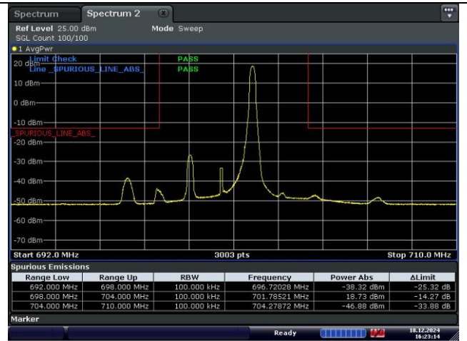
16QAM Low Channel - 1 RB - Right
