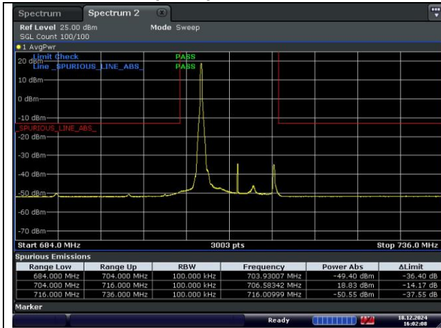
QPSK High Channel - 1 RB - Left
