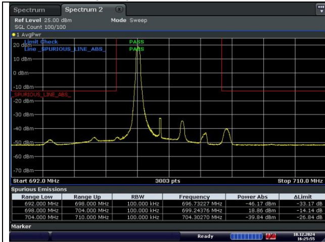
16QAM Low Channel - 1 RB - Left
