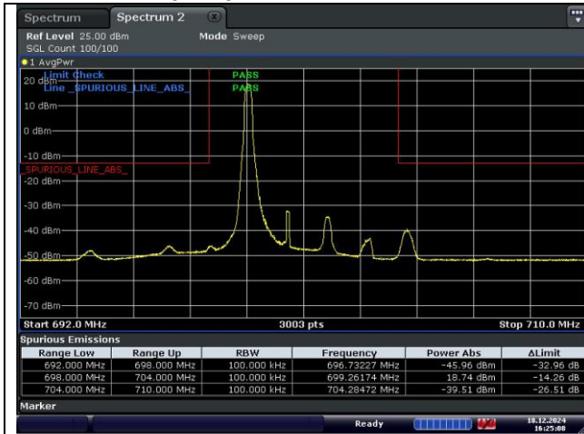
QPSK Low Channel - 1 RB - Left
