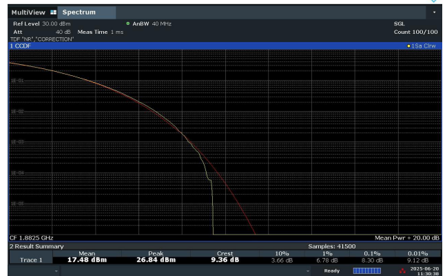
30 MHz Middle Channel - CP-OFDM 256QAM
