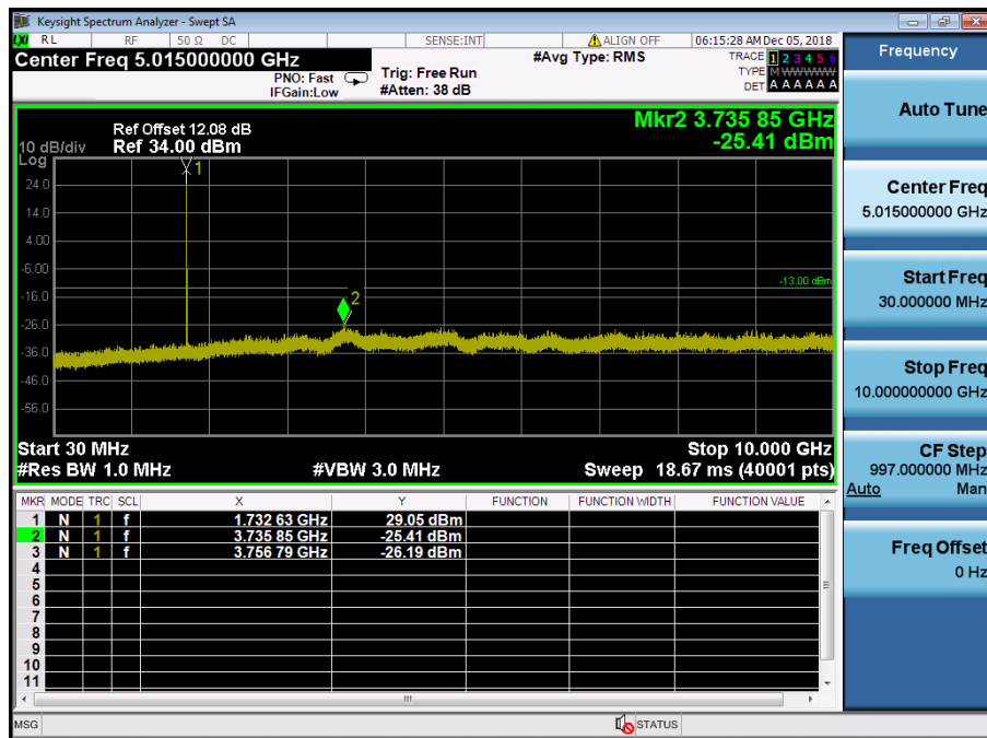
LTE Band 4 / 3MHz / QPSK - RB Size/Offset (1/7) – Mid Channel
