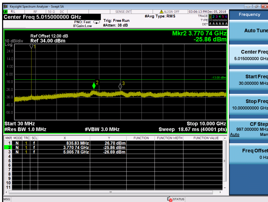
LTE Band 5 / 3MHz / QPSK - RB Size/Offset (8/0) – Mid Channel
