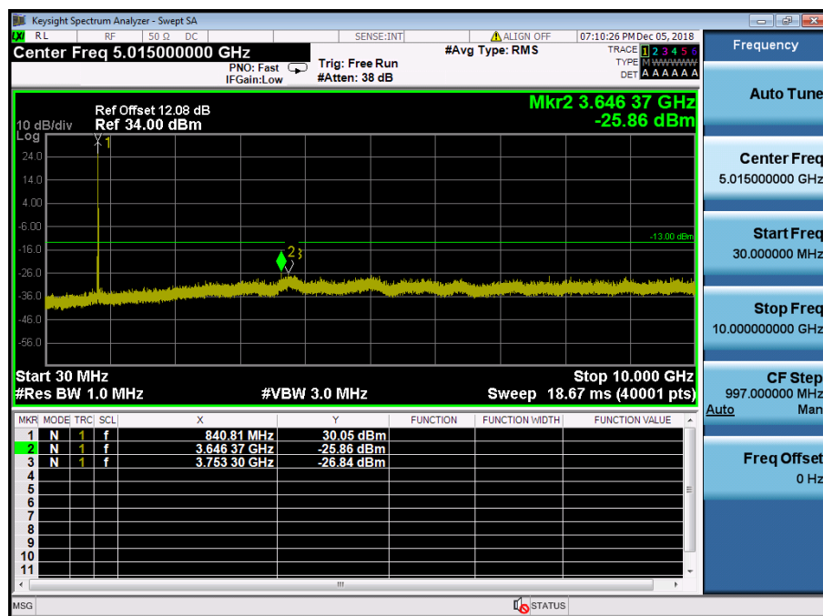
LTE Band 5 / 10MHz / 16QAM - RB Size/Offset (1/49) – Mid Channel
