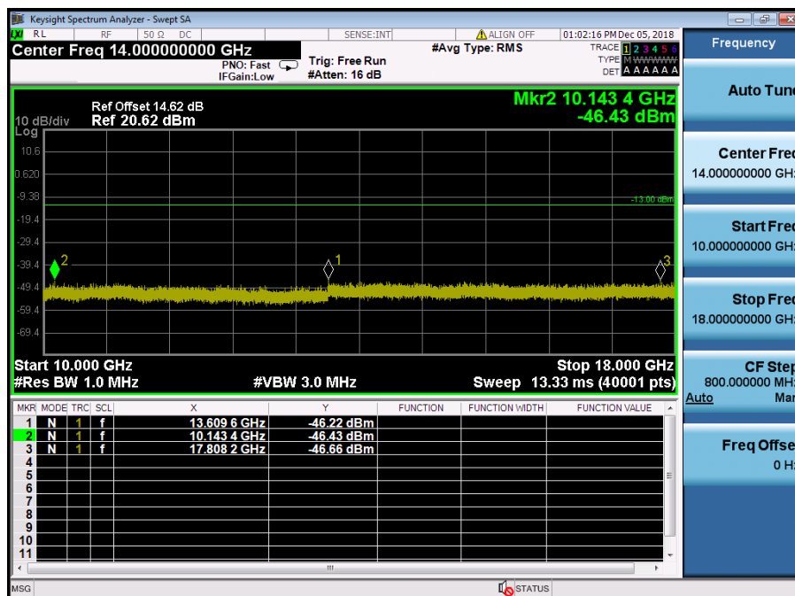
LTE Band 4 / 15MHz / 16QAM - RB Size/Offset (1/36) – Mid Channel
