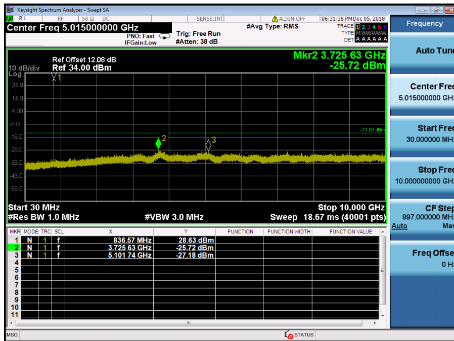
LTE Band 5 / 5MHz / 16QAM - RB Size/Offset (1/12) – Mid Channel
