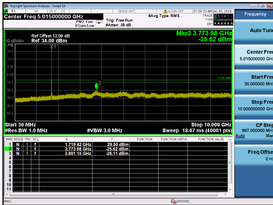
LTE Band 4 / 10MHz / QPSK - RB Size/Offset (1/49) – Low Channel
