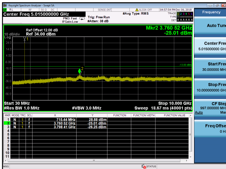
LTE Band 12 / 1.4MHz / 16QAM - RB Size/Offset (1/2) – High Channel
