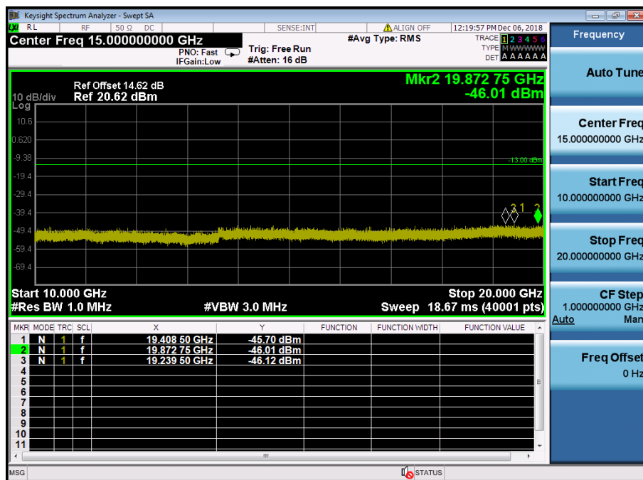
LTE Band 2 / 10MHz / 16QAM - RB Size/Offset (25/25) – Mid Channel
