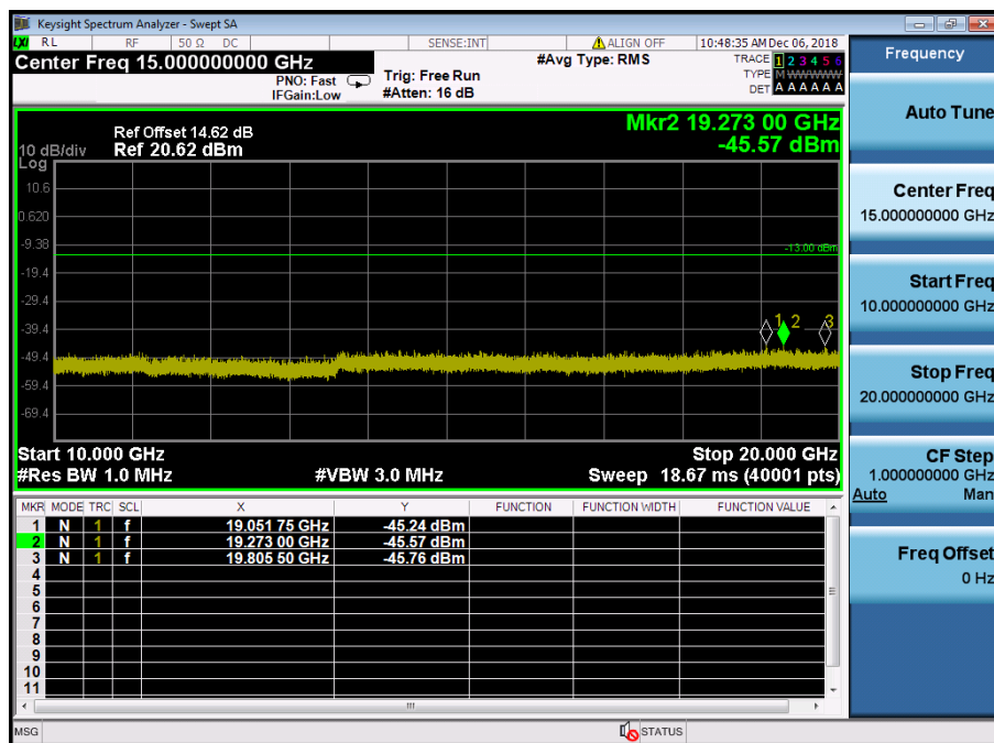
LTE Band 2 / 3MHz / 16QAM - RB Size/Offset (8/0) – Mid Channel
