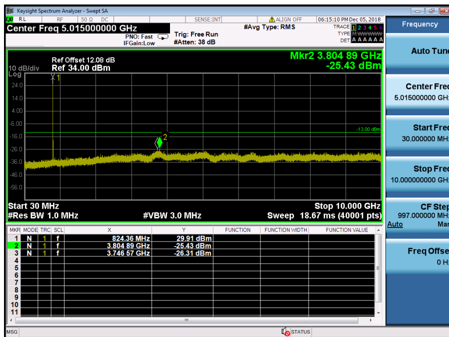
LTE Band 5 / 5MHz / 16QAM - RB Size/Offset (1/0) – Low Channel
