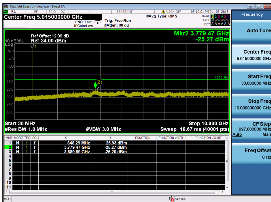
LTE Band 5 / 1.4MHz / 16QAM - RB Size/Offset (6/0) – High Channel
