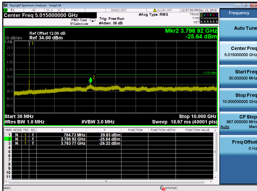
LTE Band 13 / 5MHz / 16QAM - RB Size/Offset (1/12) – High Channel
