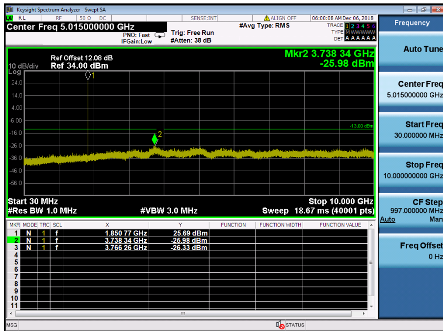
LTE Band 2 / 3MHz / QPSK - RB Size/Offset (8/0) – Low Channel
