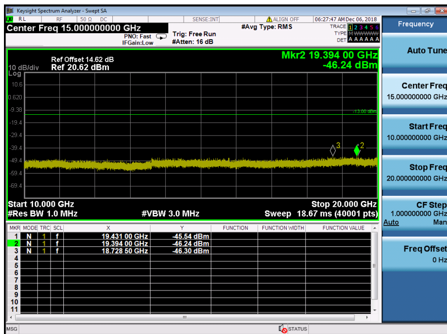
LTE Band 2 / 3MHz / QPSK - RB Size/Offset (8/4) – High Channel
