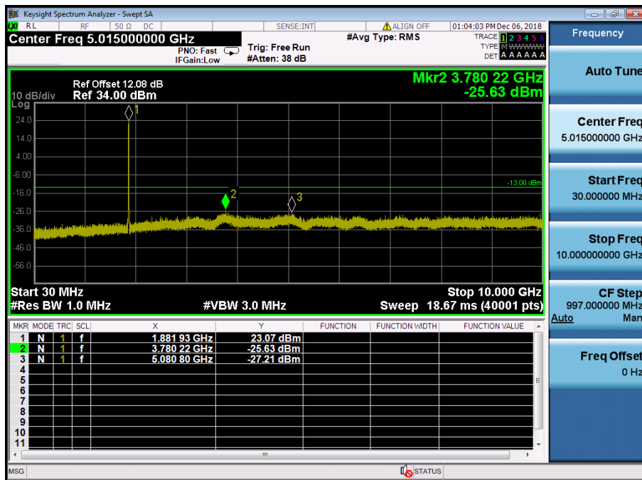
LTE Band 2 / 15MHz / 16QAM - RB Size/Offset (36/39) – Mid Channel
