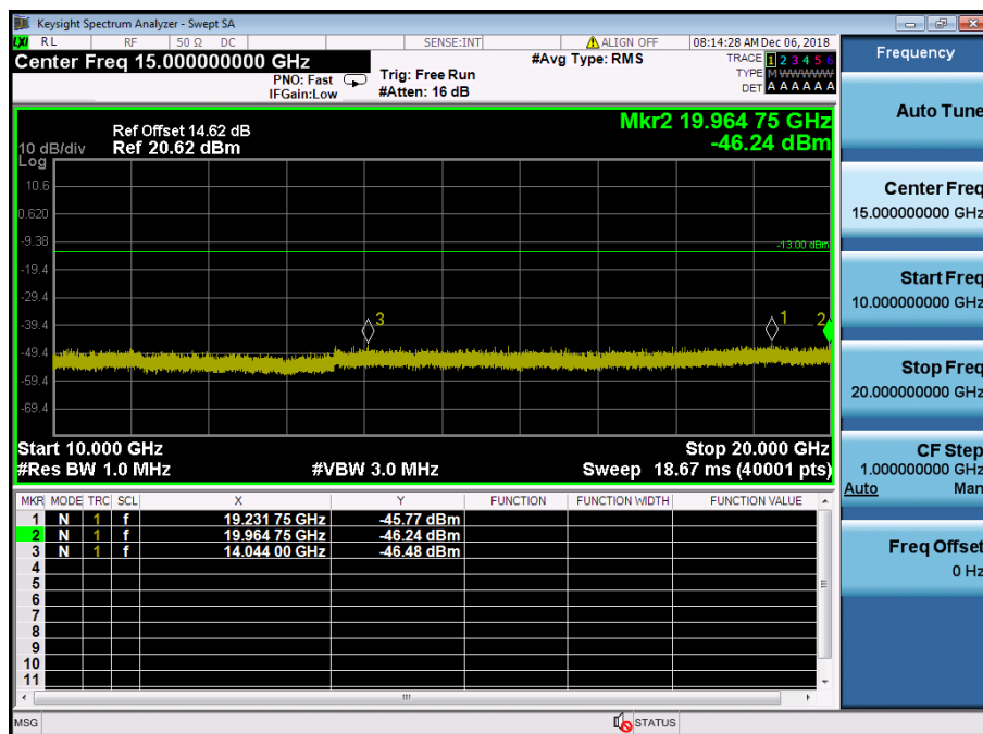
LTE Band 2 / 15MHz / QPSK - RB Size/Offset (36/18)–Low Channel
