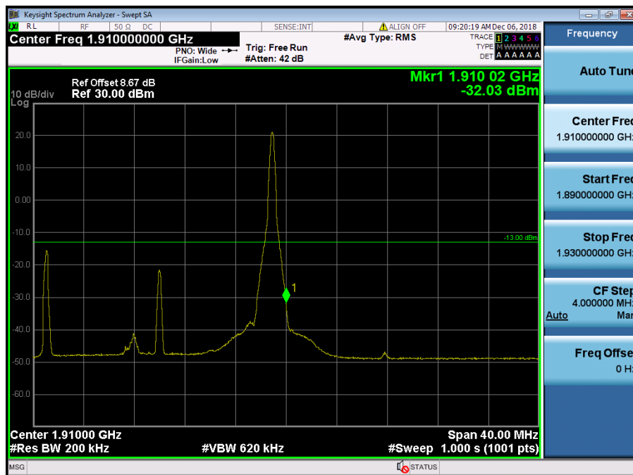
LTE Band 2 / 2MHz / QPSK - RB Size/Offset (1/99)
