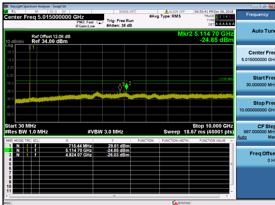
LTE Band 12,17 / 10MHz / 16QAM - RB Size/Offset (1/49) – High Channel
