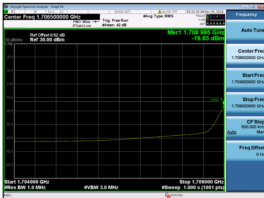
LTE Band 4 / 1.4MHz / QPSK - RB Size/Offset (8/4)
