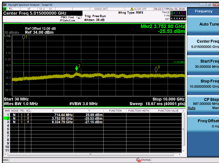
LTE Band 12,17 / 5MHz / 16QAM - RB Size/Offset (12/13) – High Channel
