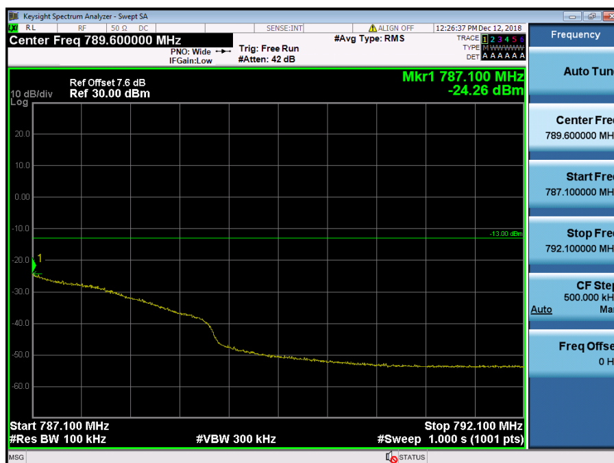
LTE Band 13 / 5MHz / QPSK - RB Size/Offset (12/13)
