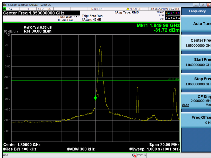
LTE Band 2 / 10MHz / 16QAM - RB Size/Offset (1/0)
