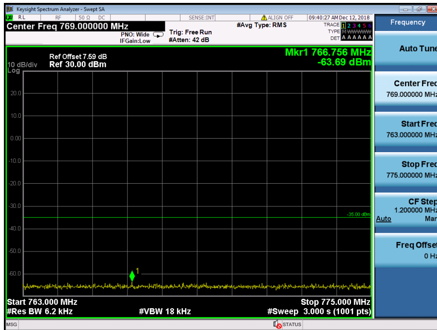
LTE Band 13 / 5MHz / QPSK - RB Size/Offset (1/12)
